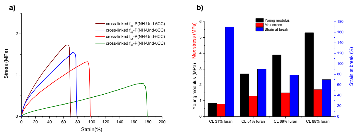
Figure 30: a) Tensile tests performed at 65^\circ\text{C} for various polycarbonate materials and b) the corresponding Young's modulus, max stress, and strain at break
