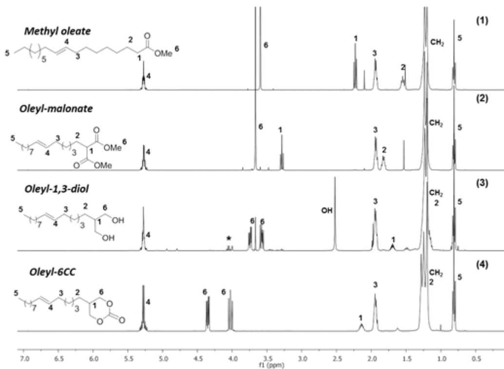
ESI Figure 1: Stacked 1 H NMR spectra of (1) methyl oleate, (2) Ole-malonate, (3) Ole-1,3-diol and (4) Ole-6CC. (All analyses were performed in CDCl 3 )(* impurities).
