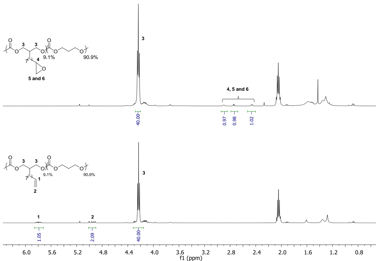
Figure 5: Stacked ^1\text{H} NMR of P(TMC- co -Und-6CC) and epoxidized P(TMC- co -Und-6CC) in \text{CDCl}_3
