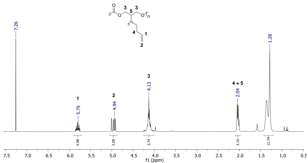
ESI Figure 4: 1 H NMR spectra of P(Und-6CC) in CDCl 3
