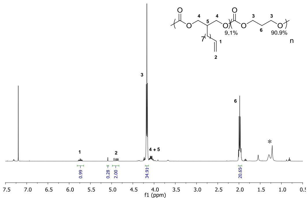
Figure 8: 1 H NMR spectrum of P(TMC-co-Und-6CC) (Table 1, entry 4)(* : CH 2 signals of Und-6CC units).
