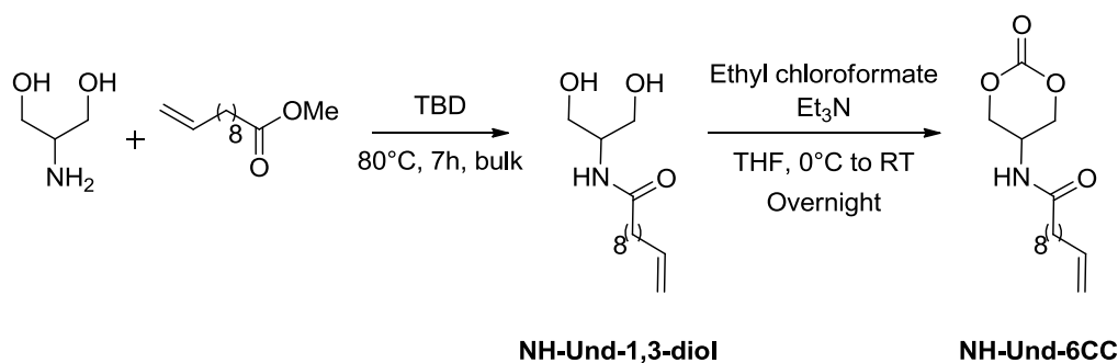
Scheme 3: Synthesis of 6-membered cyclic carbonate from 2-amino-1,3-propanediol and methyl undecenoate
