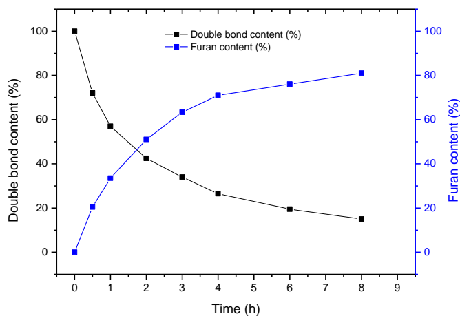
Figure 22: Kinetic profile of the P(NH-Und-6CC) functionalization by furan rings.
