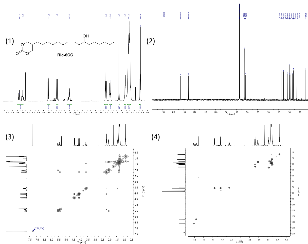
ESI Figure 2: Characterization of Ric-6CC (1) ^1\text{H} NMR (2) ^{13}\text{C} NMR, (3) ^1\text{H} - ^1\text{H} COSY NMR and (4) ^1\text{H} - ^{13}\text{C} HSQC-NMR. (Analysis performed in \text{CDCl}_3 )
