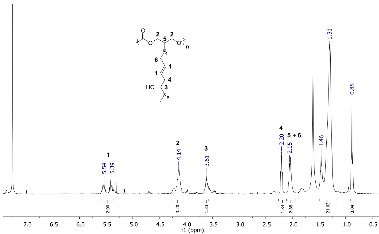
ESI Figure 7: 1 H NMR spectra of P(Lin-6CC) in CDCl 3
