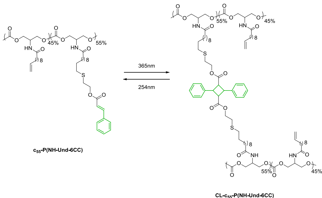
Figure 37: Photo-reversible cross-linking of c_{55} -P(NH-Und-6CC)
