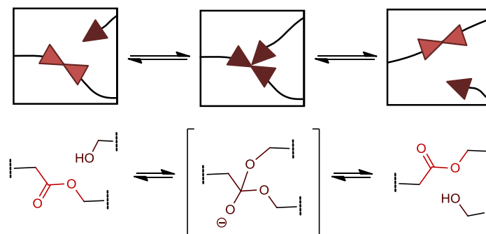
Figure 15: Non-dynamic reversible addition (top) and dynamic reversible exchange (bottom) cross-linking reactions 33
