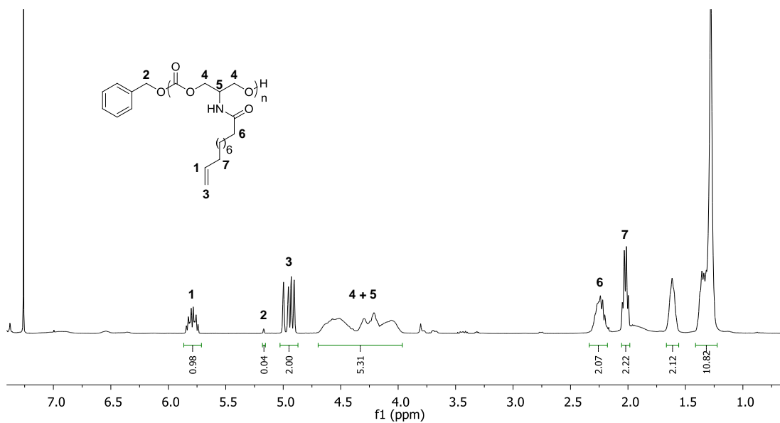
Figure 14: ^1H NMR spectrum of P(NH-Und-6CC) in CDCl_3
