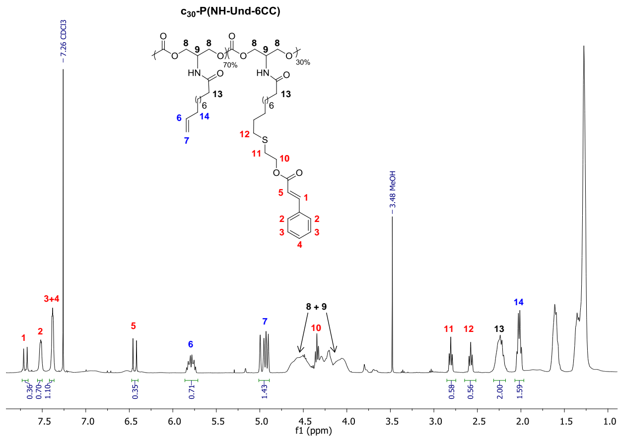
Figure 35: 1 H NMR spectrum of c 30 -P(NH-Und-6CC) in CDCl 3
