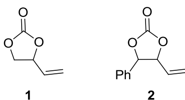
Figure 4: Vinylic-functionalized 5CCs
