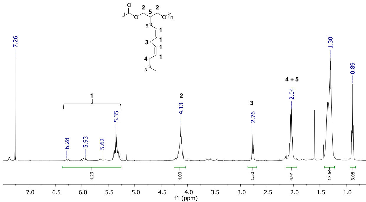
ESI Figure 6: 1 H NMR spectra of P(Lin-6CC) in CDCl 3
