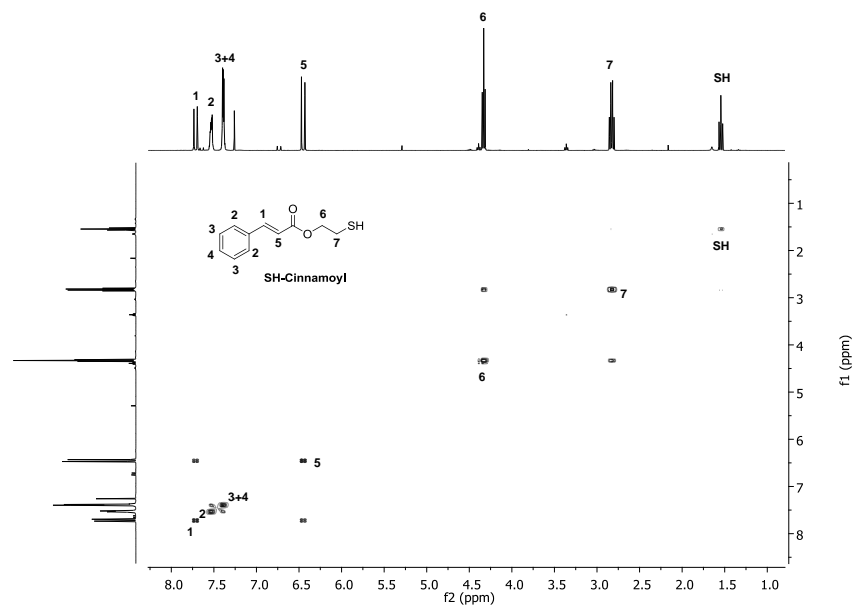
Figure 34: COSY NMR spectrum of SH-Cinnamoyl in \text{CDCl}_3
