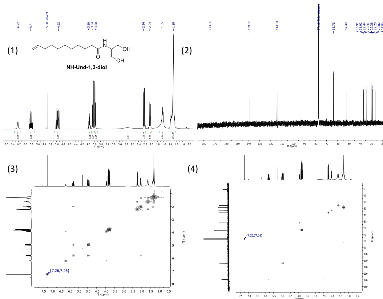
ESI Figure 8: Characterization of NH-Und-1,3-diol (1) 1 H NMR (2) 13 C NMR, (3) 1 H- 1 H COSY NMR and (4) 1 H- 13 C HSQC-NMR. (Analysis performed in CDCl 3 )
