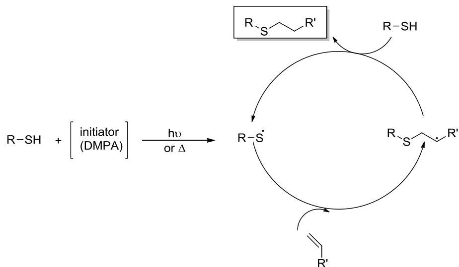
Figure 6: Mechanism of thiol-ene addition on terminal alkene
