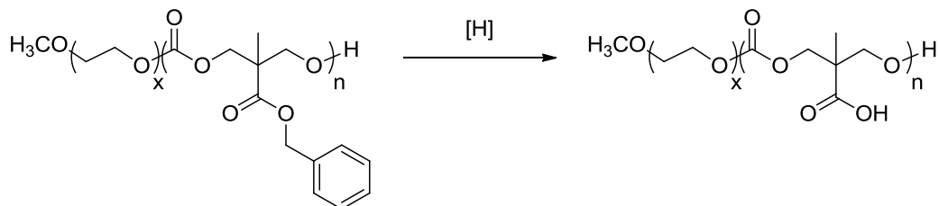
Scheme 34: Hydrogenolysis of protected copolycarbonate
