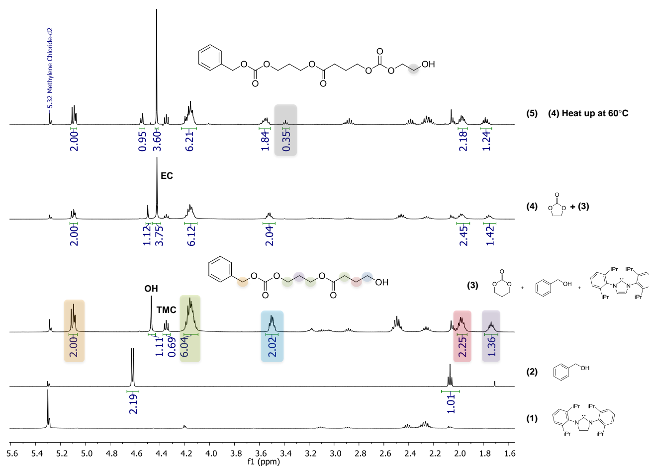
Figure 5: 1 H NMR spectra towards a better understanding of EC/TMC copolymerization in CD 2 Cl 2
