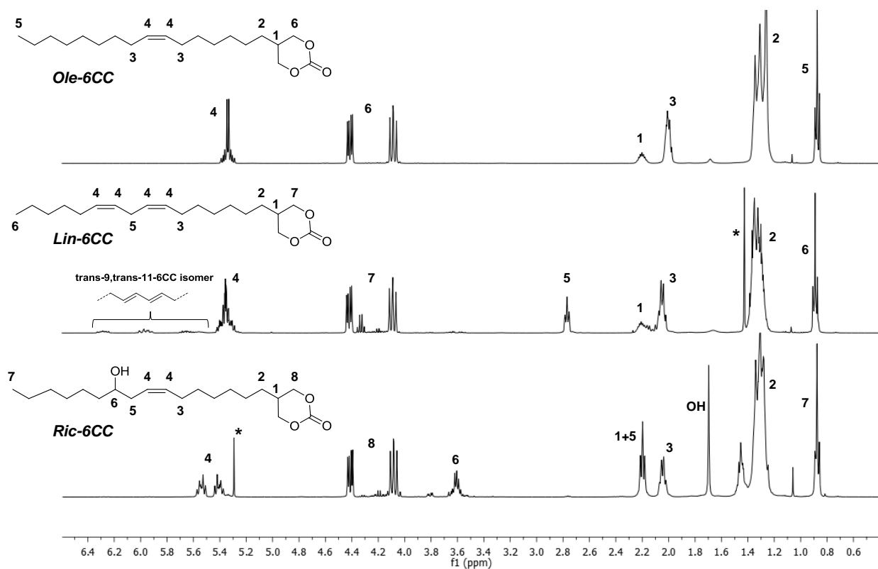
Figure 3: Stacked 1 H NMR of Ole-6CC, Lin-6CC and Ric-6CC in CDCl 3
