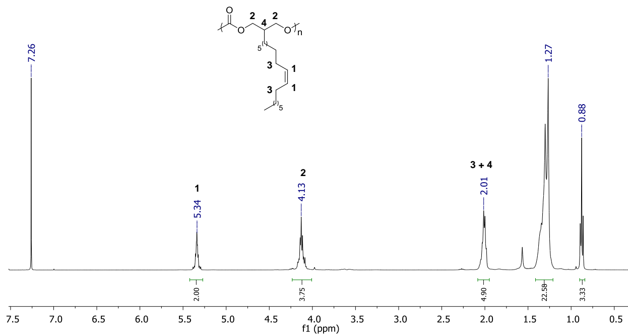
ESI Figure 5: 1 H NMR spectra of P(Ole-6CC) in CDCl 3
