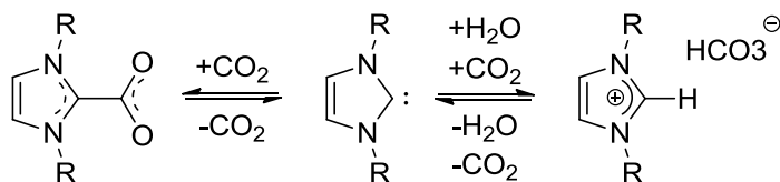
Scheme 18: Reversible generation of NHCs from [\text{NHC}(\text{H})] [\text{HCO}_3] salts and NHC- \text{CO}_2 adducts
