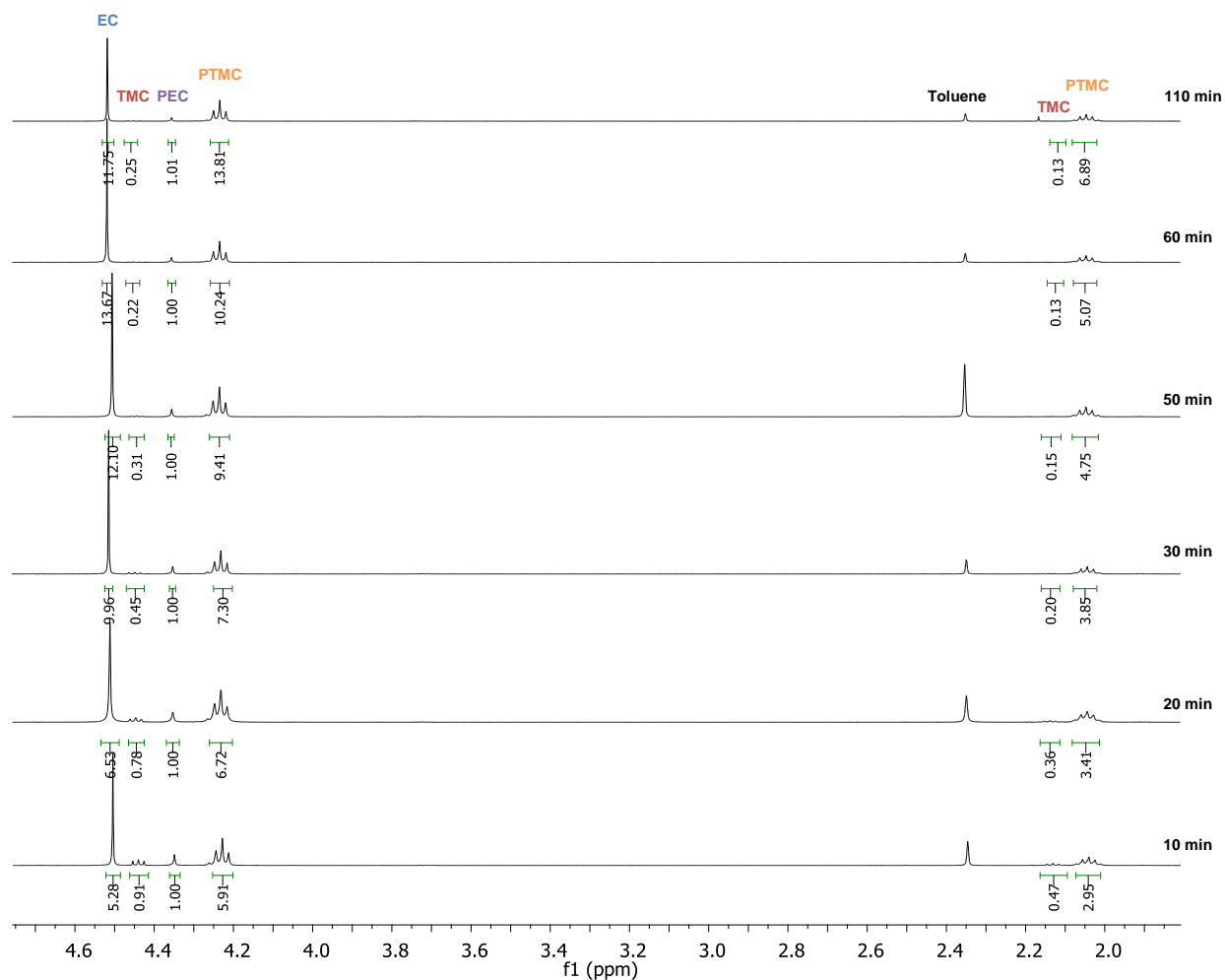
Figure 3: Stacked 1 H NMR spectra used for the kinetic study of the EC/TMC copolymerization in CDCl 3
