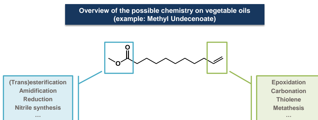
Figure 2: Methyl undecenoate as a source of various building blocks
