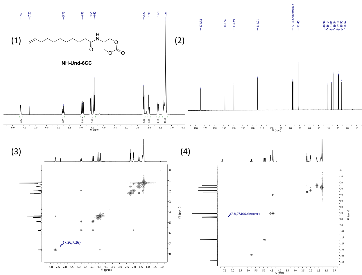
ESI Figure 9: Characterization of NH-Und-6CC (1) ^1\text{H} NMR (2) ^{13}\text{C} NMR, (3) ^1\text{H} - ^1\text{H} COSY NMR and (4) ^1\text{H} - ^{13}\text{C} HSQC-NMR. (Analysis performed in \text{CDCl}_3 )
