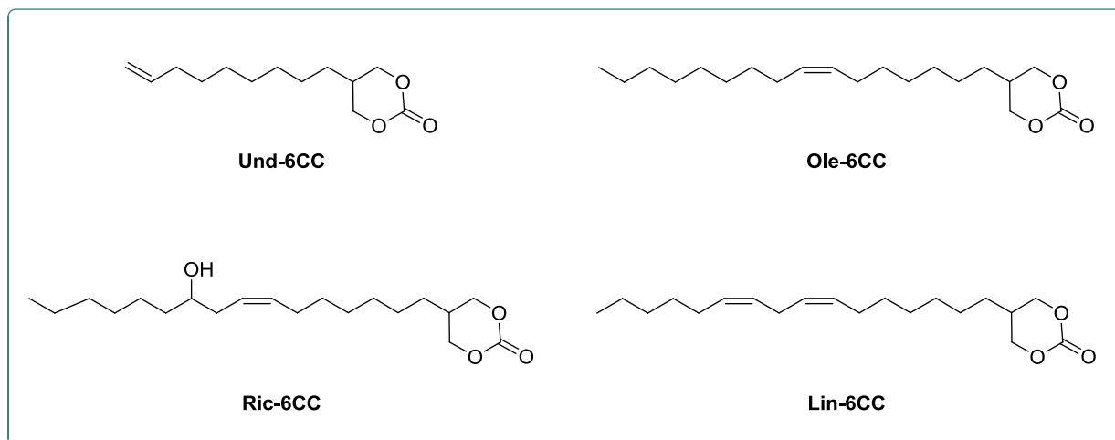
Figure 2: First platform of fatty acid-based 6-membered cyclic carbonates
