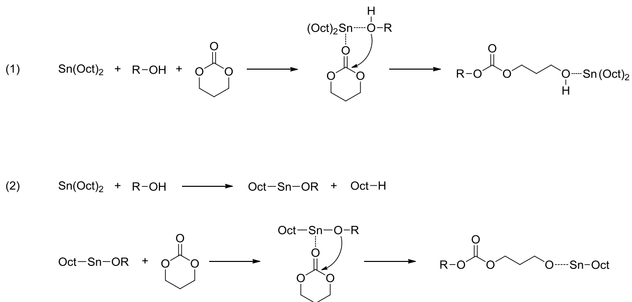
Scheme 27: Mechanisms proposed for the ROP of TMC catalyzed by Sn(Oct) 2
