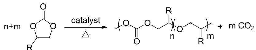
Scheme 11: Poly(alkylene carbonate- co -alkylene oxide) prepared by ROP of 5CCs
