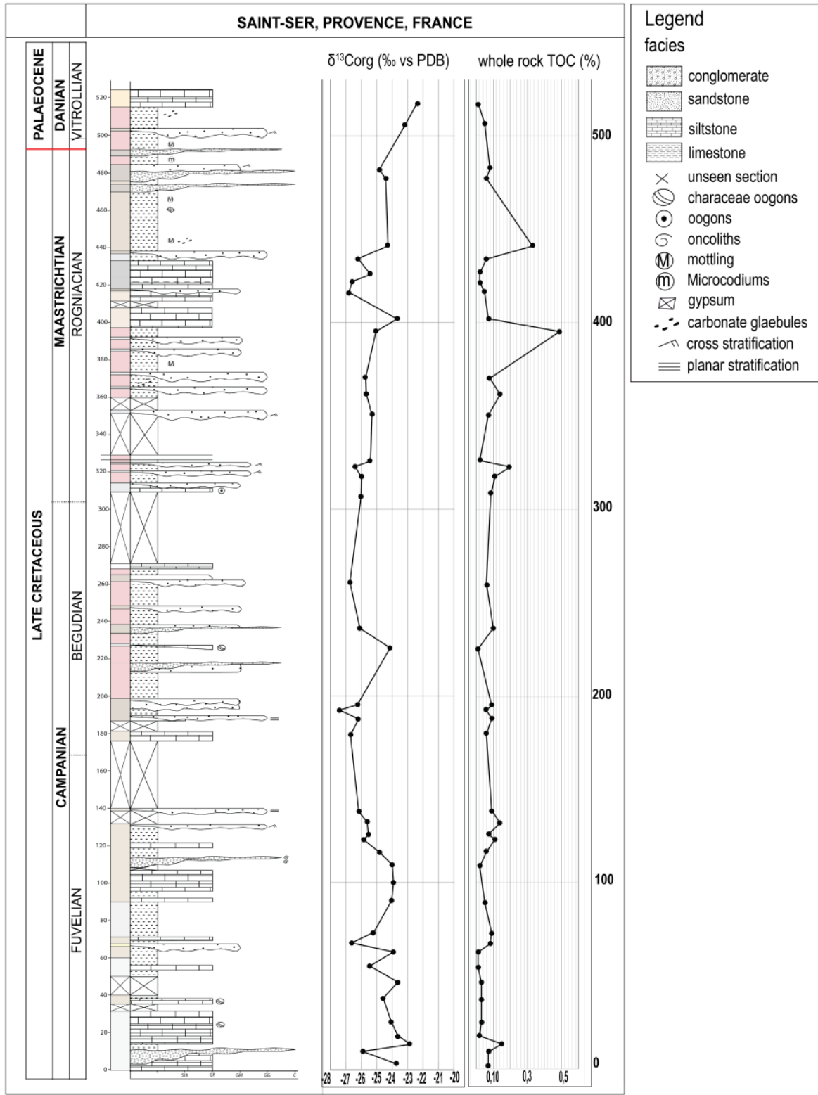
Fig.7.3: Results of TOC and \delta^{13}\text{C}_{\text{org}} analyses of Saint-Ser section. The analyses were performed on decarbonated samples.
