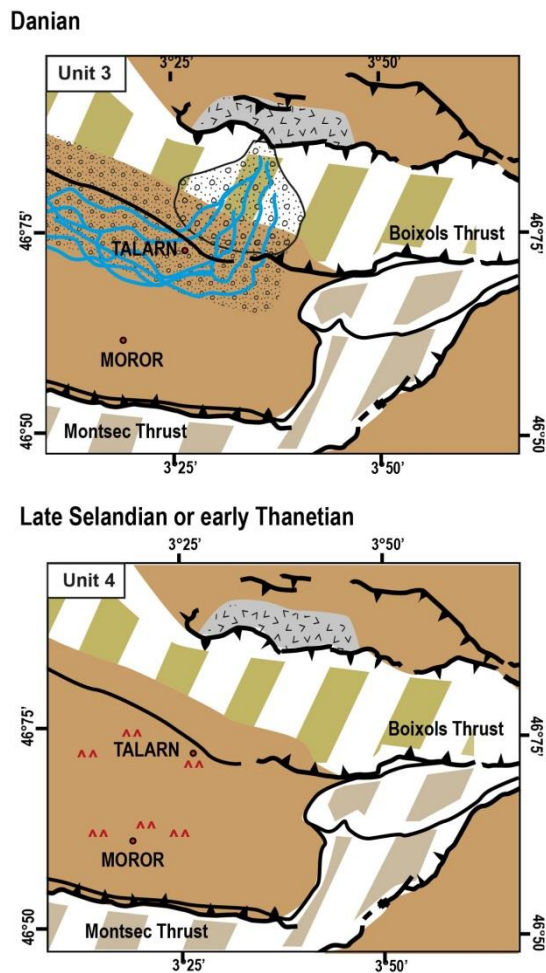
Fig. 3.15: Paleogeographic diagram of the Tresp-Graus Basin showing deposits environments during the Danian and the late Selandian/early Thanetian.
