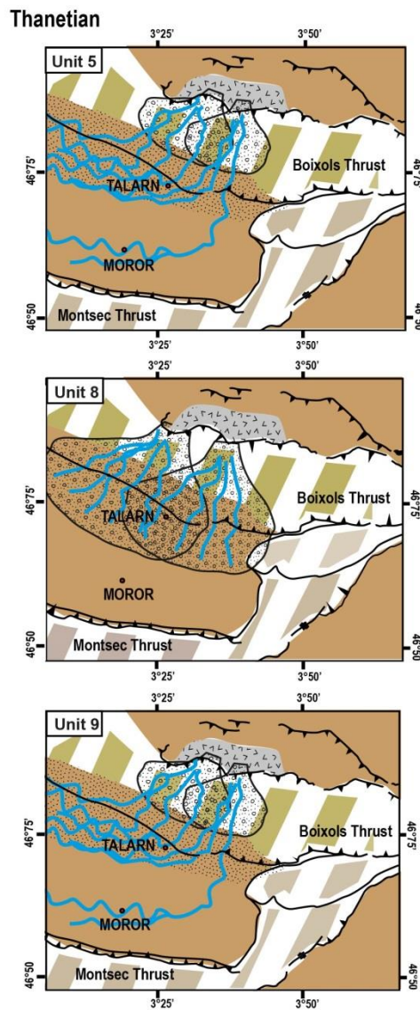
Fig.3.16 : Paleogeographic diagram of the Tremp-Graus Basin showing deposits environments during the Thanetian.
