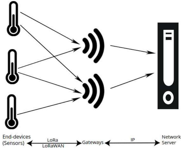
Figure 2.4: LoRaWAN architecture.
