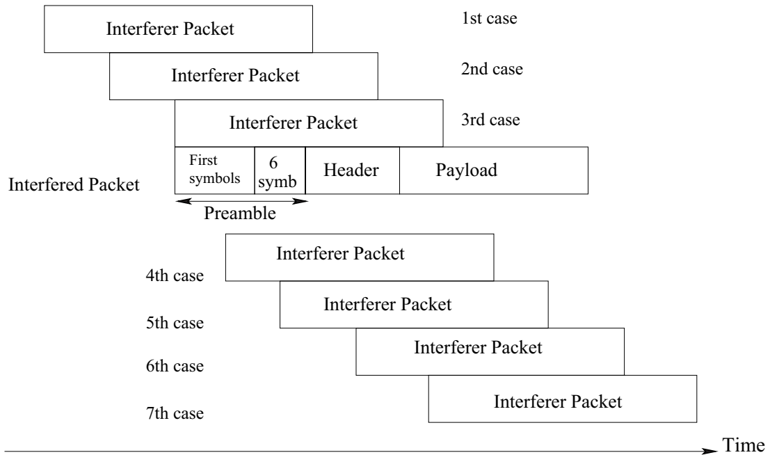
Figure 3.4: All the possible cases where an interferer can collide with an interfered.
