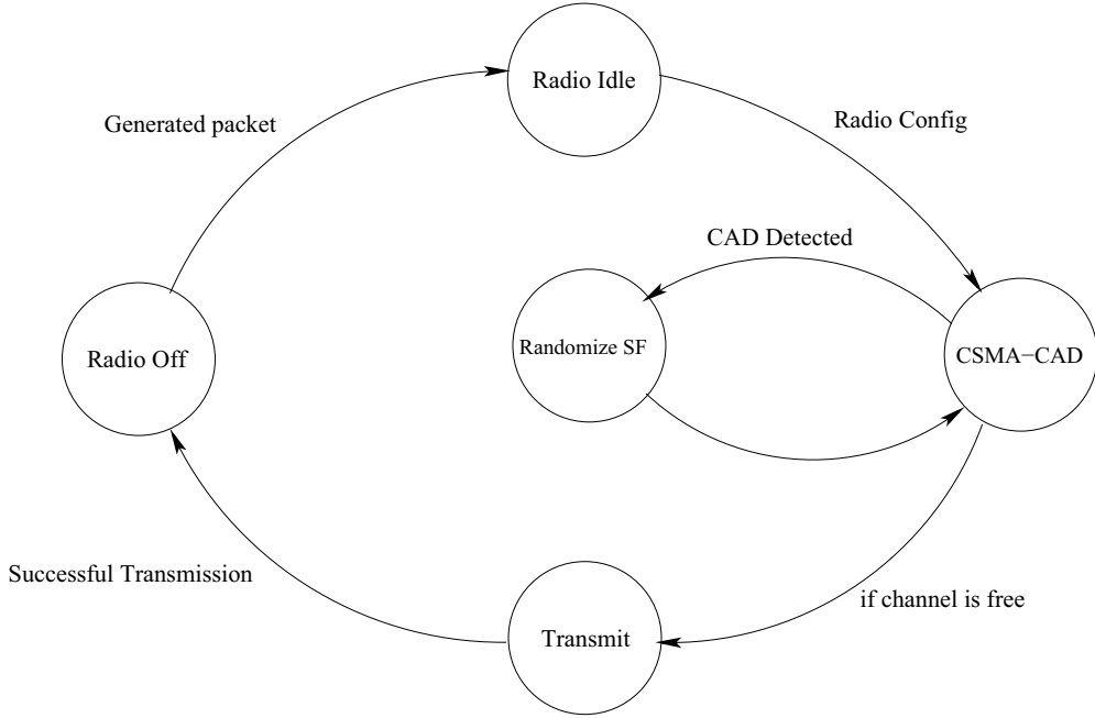
Figure 3.3: The CSMA-CAD mechanism for an end-device [3].
