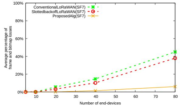
Figure 5.13: Average percentage of bitmap and frame losses in a small network with dc = 10\% .
