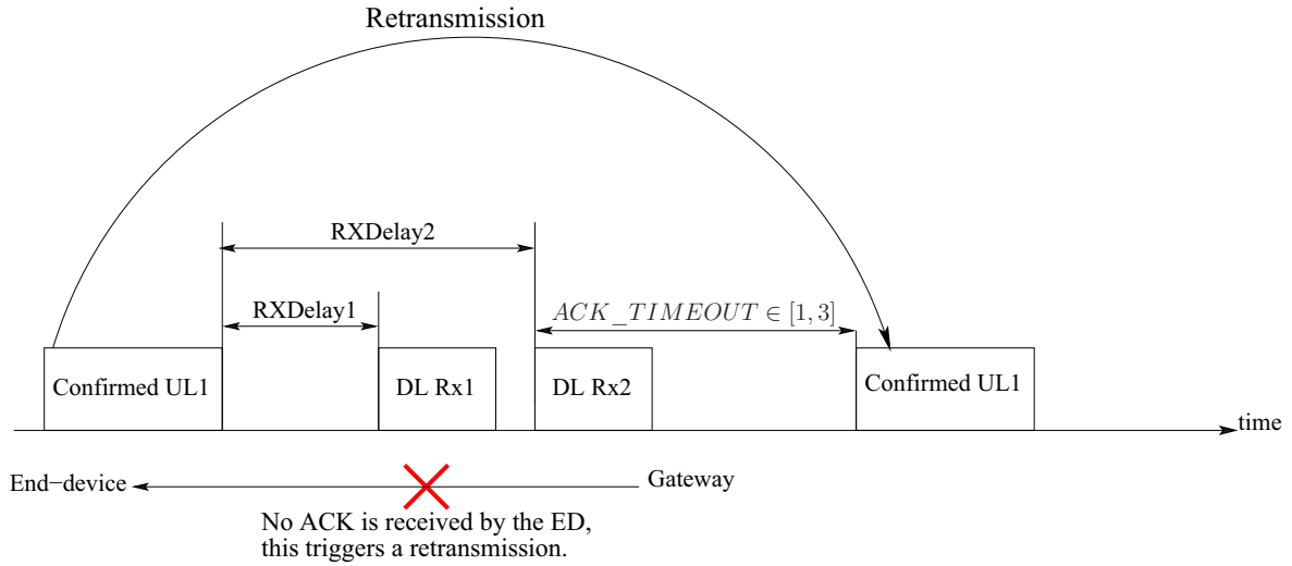
Figure 2.6: LoRaWAN Retransmission Procedure.
