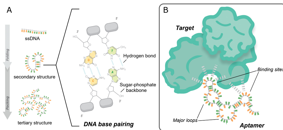
Figure 1.5: a) The aptamer structure resulting from base pairing, b) Aptamer binding the target through hydrogen bonding and dipolar interactions. (adapted from [38]).
