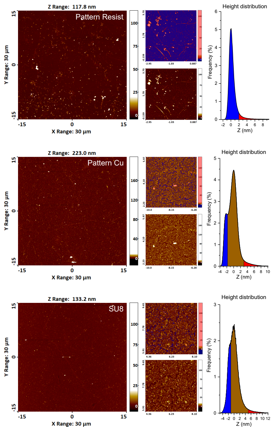
Figure 3.5: 30 μm × 30 μm 2D maps of the graphene surface (left), raw zoomed view (middle-bottom) and colorized (middle-top) with the associated height distribution (right) after graphene patterning and passivation.
