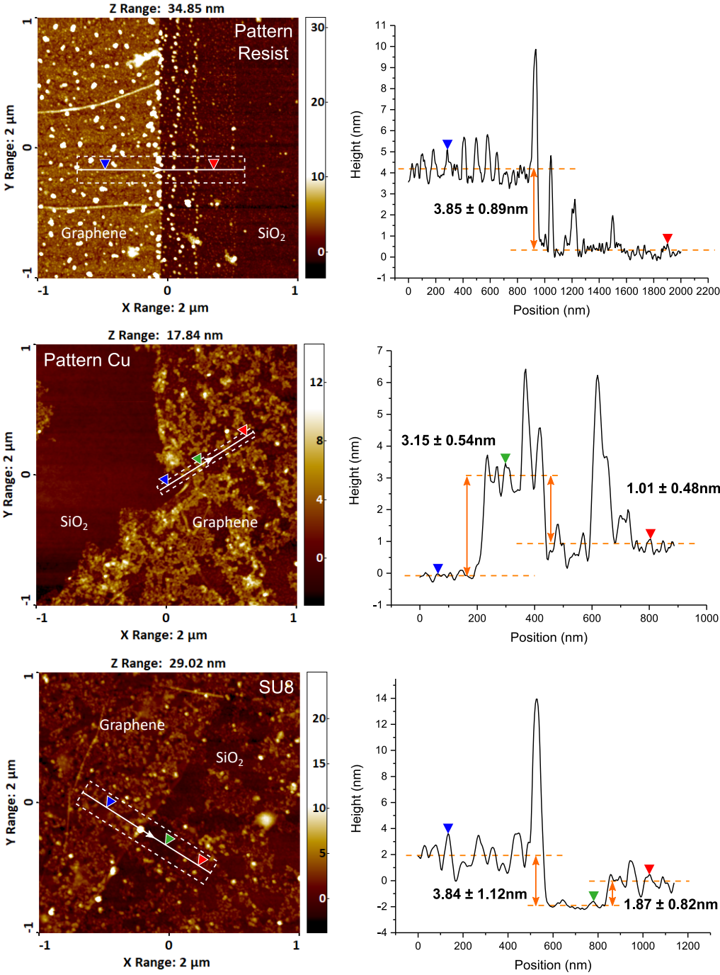
Figure 3.4: 2\ \mu\text{m} \times 2\ \mu\text{m} scan (left) at the graphene/SiO 2 interface and the associated step height (right) after graphene patterning and passivation. Colormaps are harmonized (white spots are higher than 10nm).
