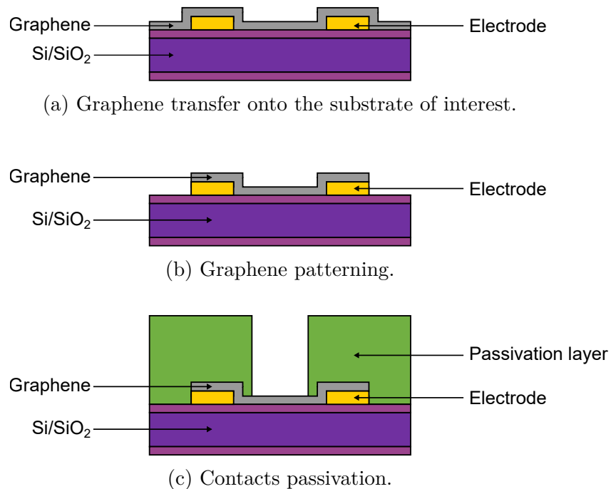
Figure 2.2: Main steps of the fabrication process developed and optimized.
