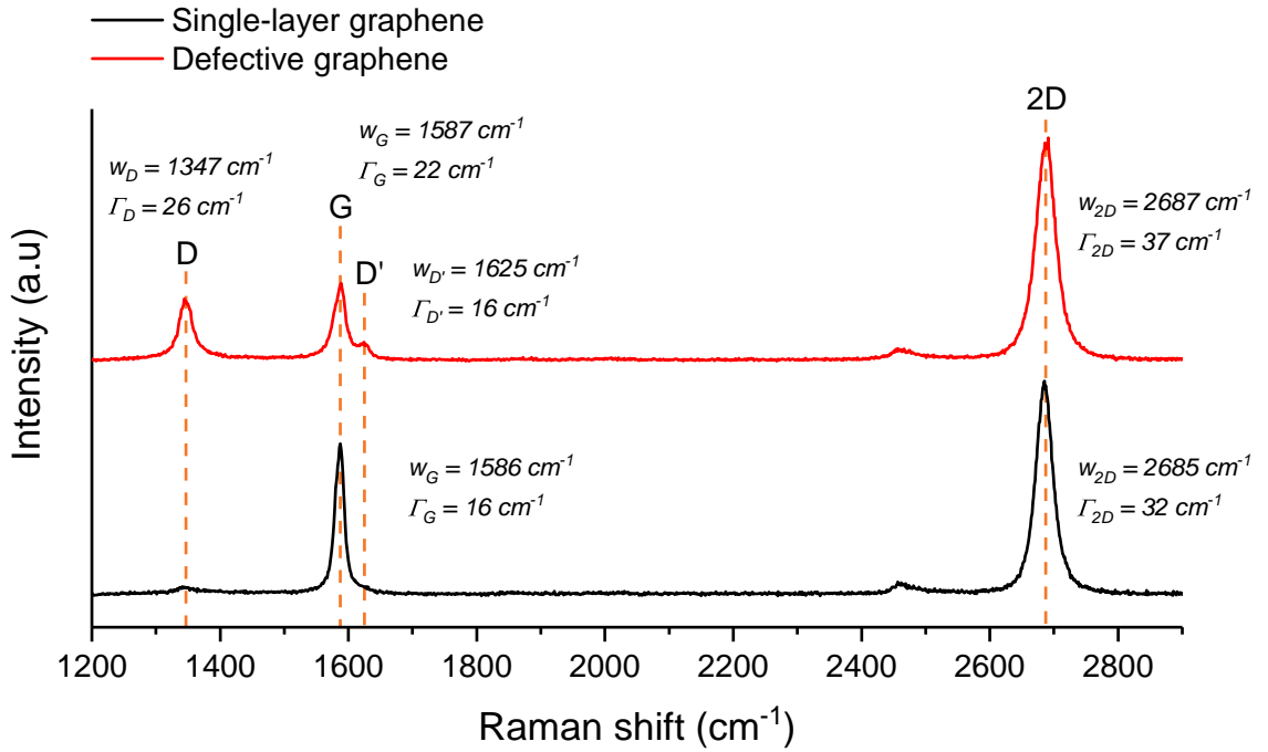
Figure 3.14: Raman spectra of typical graphene single-layer transferred onto SiO 2 substrate, and defective graphene.
