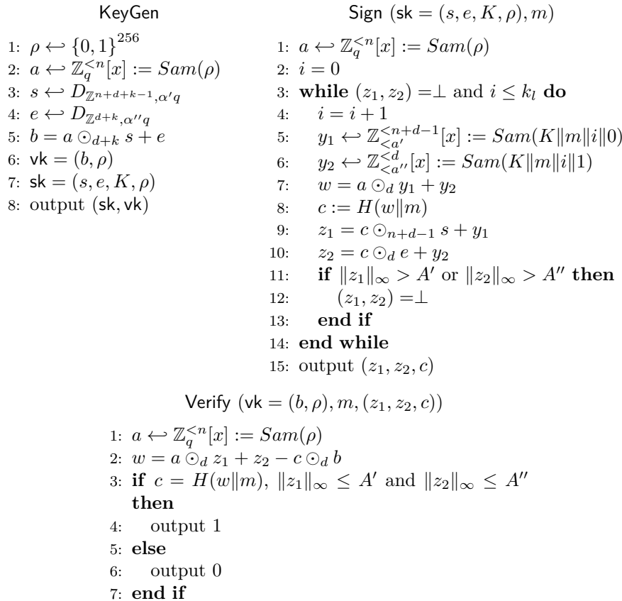
Fig. 5.6: The signature scheme.
