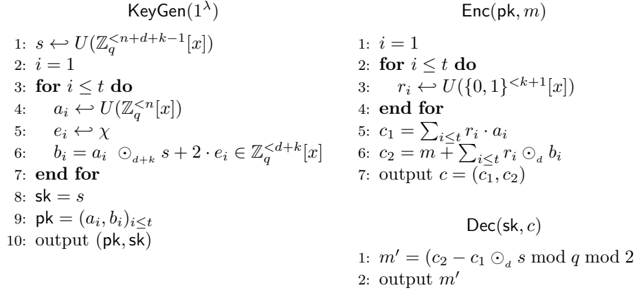
Fig. 5.1: PKE scheme from MP-LWE.
