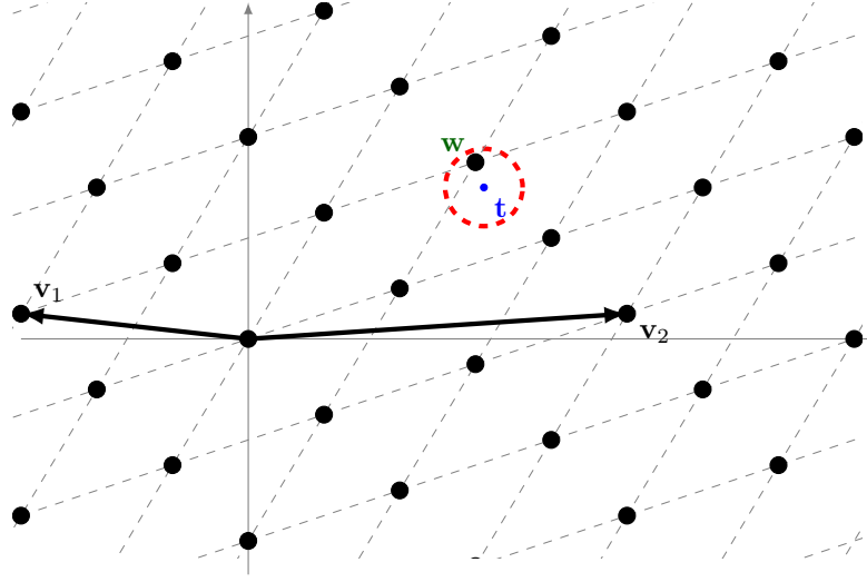
Fig. 2.3: The vector w is the closest vector to t belonging to L = L(v_1, v_2) .
