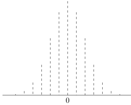
Fig. 2.4: Discrete Gaussian distribution on \mathbb{Z} of standard deviation r = 1.2 .
