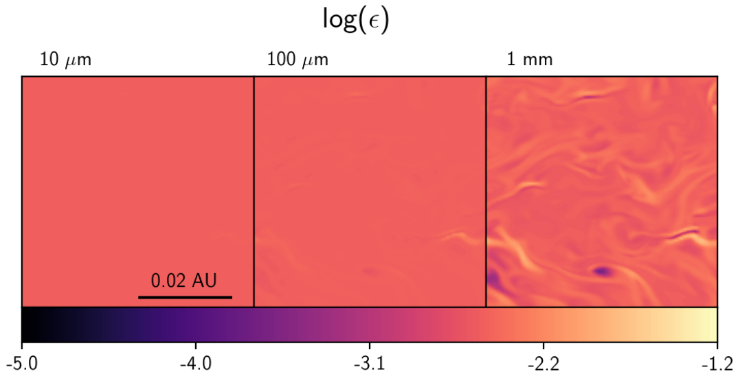
Figure 6.15: Same as figure 6.7 for the UNSTR-O10A10D10R1 model. The colormap is set to match the one in figure 6.7
