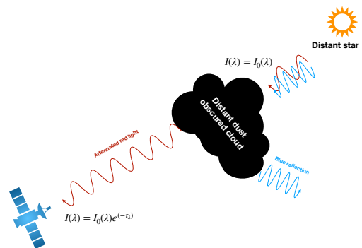
(b) Cartoon illustration explaining the dust extinction process. The blue light is almost completely absorbed by the dust while some of the red light can penetrate all the way through. A blue reflection, due to scattering by the dust grains, can be observed when the cloud is illuminated on the same side as the observer is.
