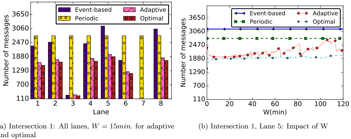
Figure 7.4: Impact of adaptive message generation. For periodic messages generation, \varphi = 30 s.
