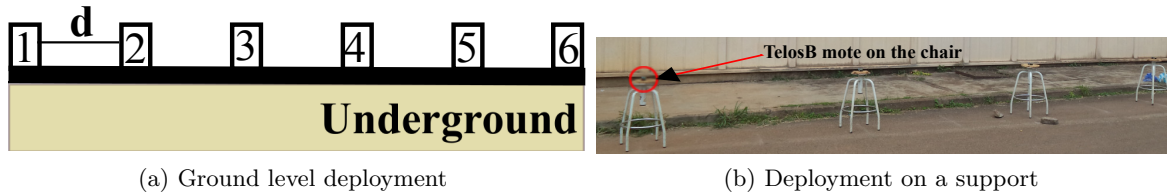
Figure 3.3: Sensors deployment.
