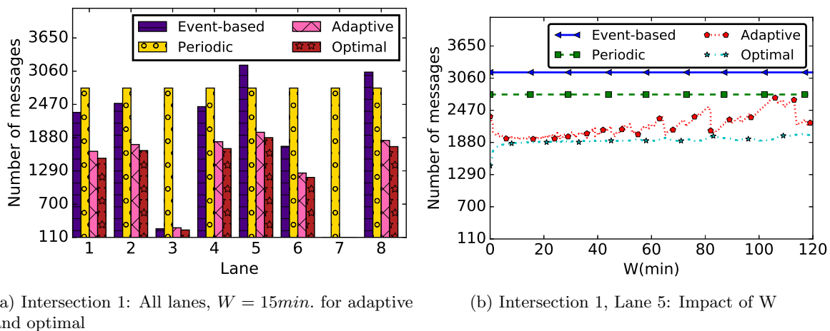
Figure 7.4: Impact of adaptive message generation. For periodic messages generation, \varphi = 30 s.
