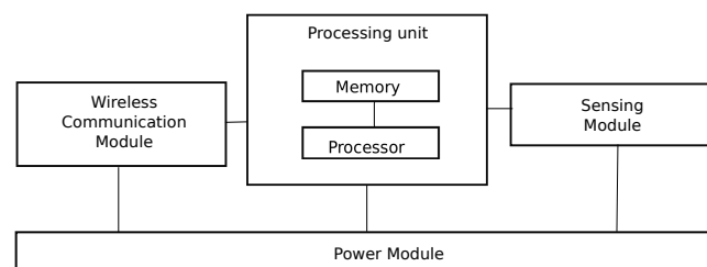
Figure 2.4: Sensor architecture
