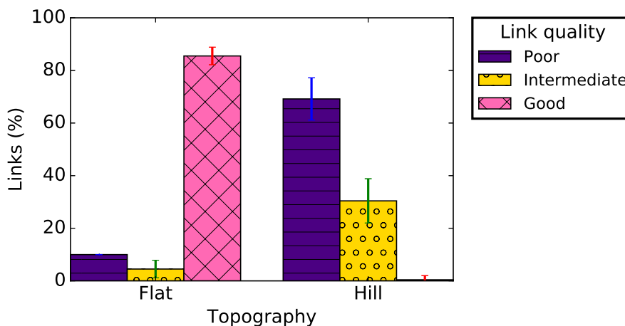
Figure 3.14: Link quality classification for different deployment environments.
