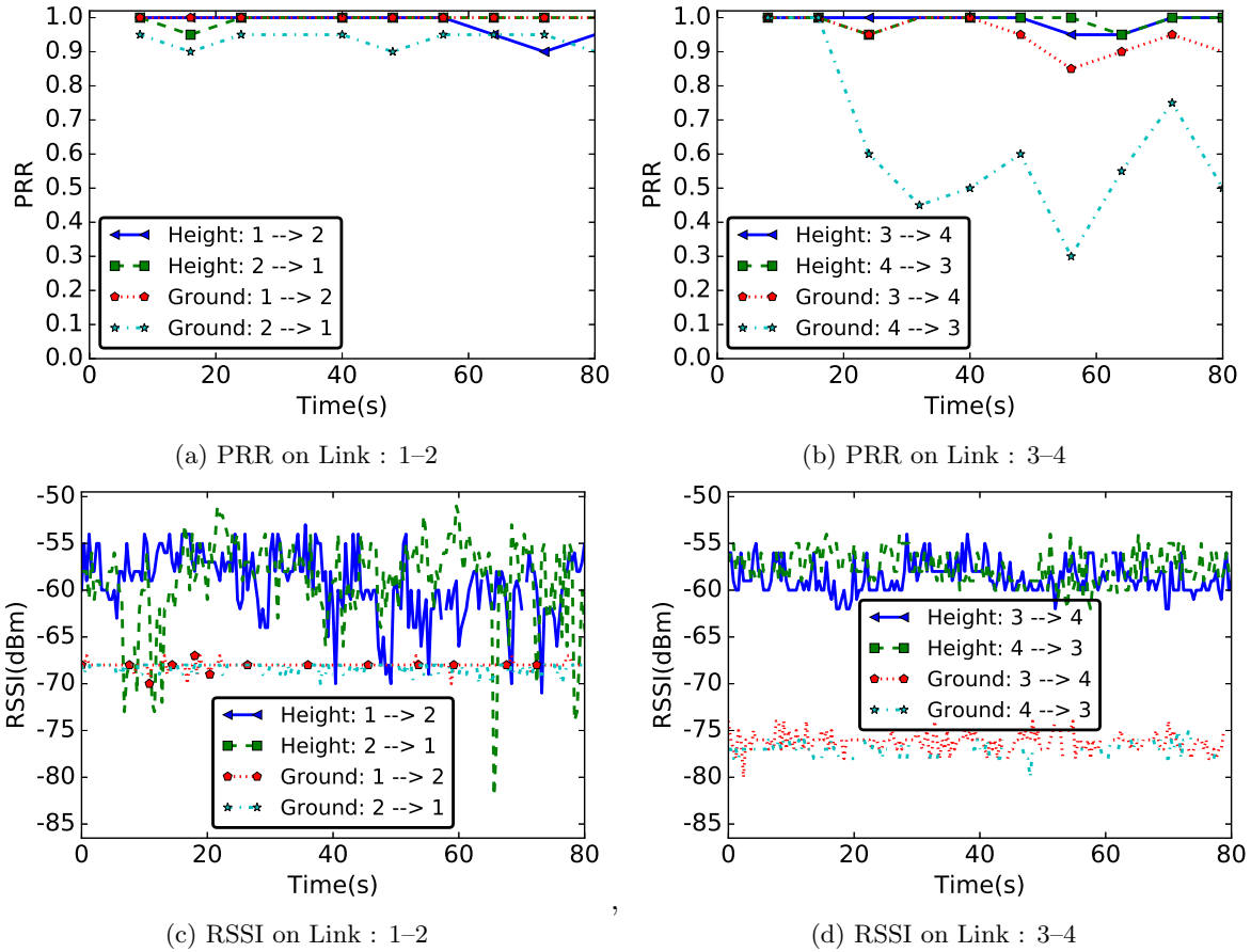
Figure 3.5: Variation of PRR and RSSI values over time on wireless links 1-2 and 3-4 , with the same distance of 3 m, in two different deployments: one with sensors deployed at ground level (labeled “Ground”) and another with sensors deployed on a support of height 57 cm ( labeled “Height”)
