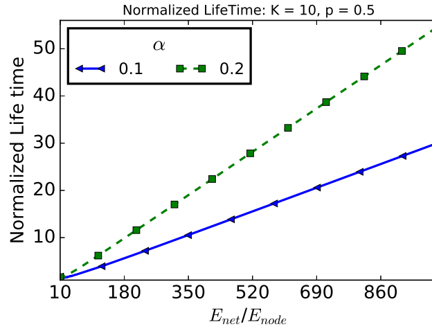
Figure 5.12: Energy distribution vs Virtual nodes-based: Impact of the energy budget when K = 10, p = 0.5 .
