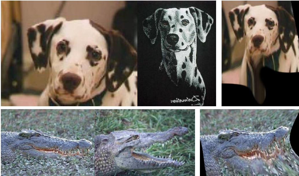
(a) Caltech-101
