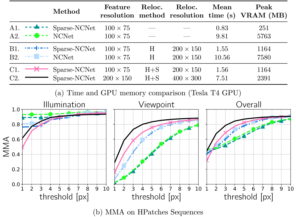
Figure 6-4: Sparse-NCNet vs. NCNet on HPatches. Sparse-NCNet can obtain equivalent results to NCNet, both without relocalization ( cf. A1 vs. A2), and with hard relocalization (H) ( cf. B1 vs. B2), while greatly reducing execution time and memory consumption. The proposed two-stage relocalization (H+S) brings an improvement in matching accuracy with a minor increase in execution time ( cf. C1 vs. B1). Finally, the reduced memory consumption in Sparse-NCNet allows for processing in higher resolution, which produces the best results, while still being faster and more memory efficient than NCNet ( cf. C2 vs. B2).
