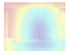
Flow field
