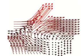
Flow field
