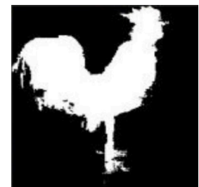
Transferred mask
