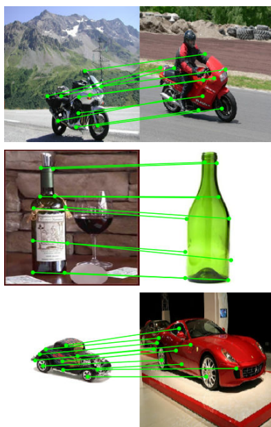
(b) PF-Willow
