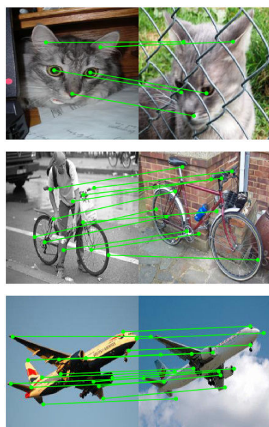
(a) PF-Pascal
