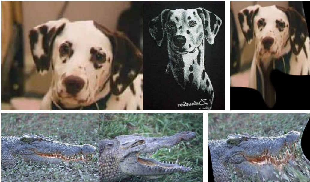
(a) Caltech-101
