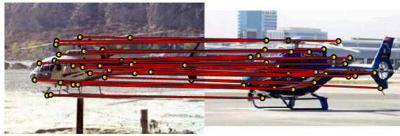
Sparse matches
