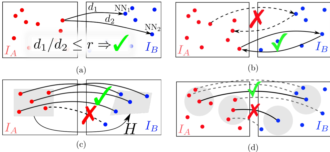
Figure 2-10: Methods for filtering incorrect matches. (a) Lowe’s second nearest-neighbour test (or ratio test) retains matches where the ratio of distances to the first and second nearest-neighbours is below a threshold. (b) The mutual correspondence test retains correspondences that are mutual when matching in both directions. (c) RANSAC can be used to robustly fit a geometric model (such as homography in the case of planar objects) and reject the matches that are not in agreement with the model. (d) Neighbourhood consensus retains correspondences which have a number of coherent supporting matches in their neighbourhoods.
