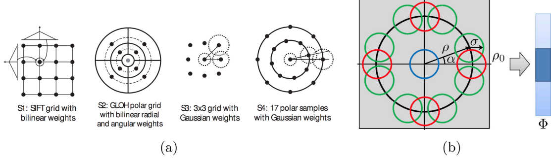
Figure 2-6: Parametric descriptors inspired by SIFT. (a) Different spatial-aggregation configurations evaluated by Winder and Brown [2007]. (b) Parametric spatial-aggregation configuration of Simonyan et al. [2014]. Figures reproduced from the respective works.
