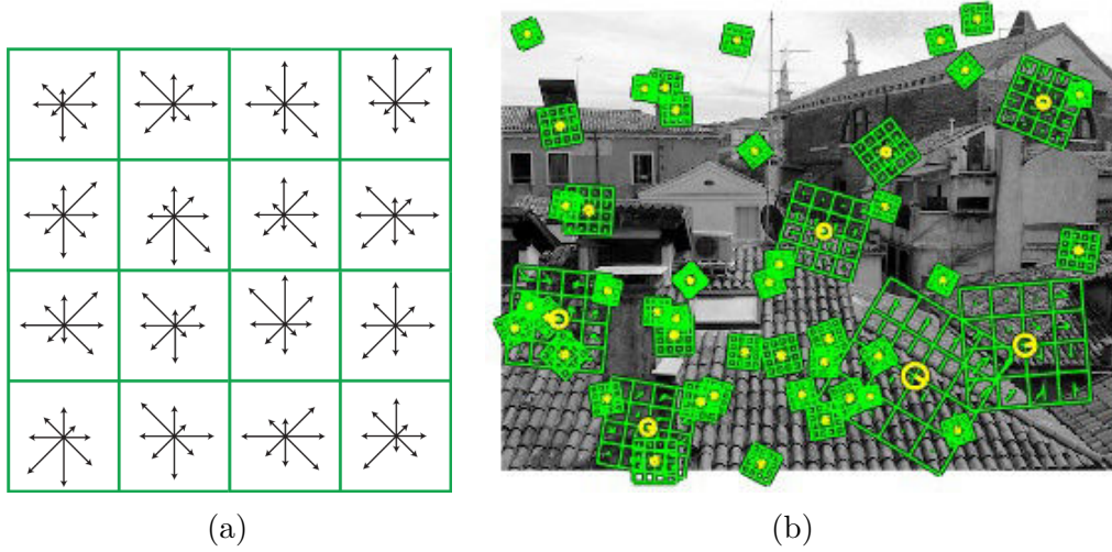
Figure 2-5: SIFT descriptor. (a) Illustration of the descriptor. The descriptor is composed by 16 histograms arranged in a 4 \times 4 grid, as shown in green. Each of these histograms contains 8 orientation bins, shown by the arrows, which accumulate the orientation of image gradients in a 4\text{px} \times 4\text{px} image cell. (b) Example SIFT descriptors (green) extracted on oriented DoG keypoints (yellow). Figures reproduced from [Lowe, 2004] and Vedaldi and Fulkerson [2010].
