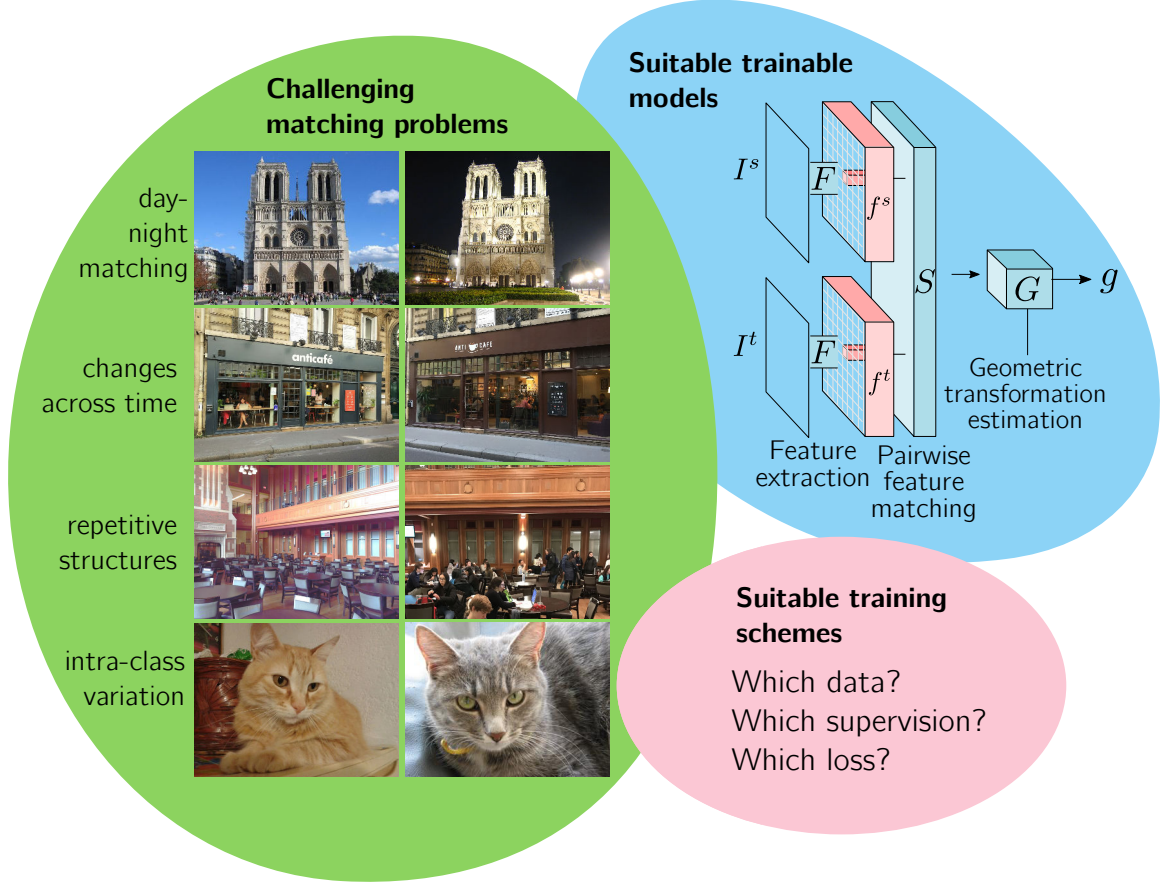
Figure 1-2: Challenges. We identify three main types of challenges: (i) those inherent to solving the difficult matching problems we address, such as day-night matching or category-level matching, (ii) those related to the formulation of suitable end-to-end trainable models for solving the correspondence problem, and (iii) finding a suitable training scheme for training such models.
