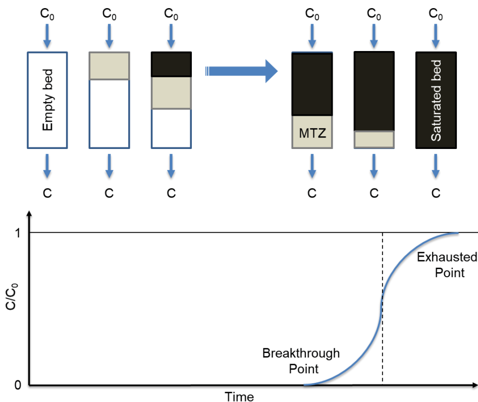
Figure 1.7 Traveling of the mass transfer zone (MTZ) through the column and development of the breakthrough curve (BTC)
