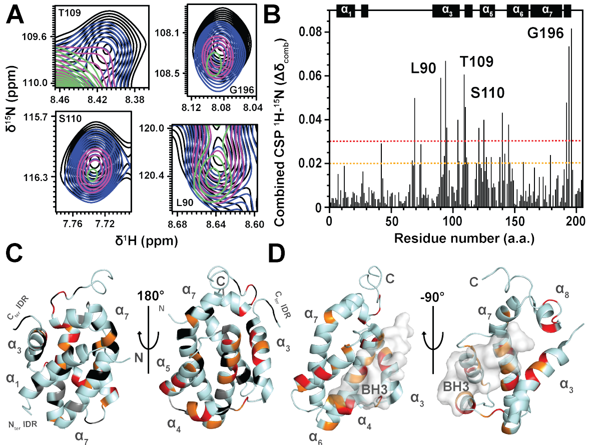
Fig. 4.26 NMR characterization of Bcl-xL in the transient complex with TCTP. (A) Overlay of ^1\text{H} - ^{15}\text{N} SOFAST HMQC spectra from isolated ^{15}\text{N} -Bcl-xL \Delta\text{TM} (500 \mu\text{M} ) (black) and in presence of 0.25 eq. (blue), 0.50 eq. (purple) or 0.75 eq. (green) His 6 -TCTP. Close-up views from residues T109, G196, S110 and L90 are shown. (B) Combined ^1\text{H} - ^{15}\text{N} chemical shift perturbations calculated between isolated ^{15}\text{N} -Bcl-xL \Delta\text{TM} and in presence of TCTP (0.75 eq.). (C) Mapping of combined ^1\text{H} - ^{15}\text{N} chemical shift perturbations (red \geq 0.03 , 0.03 \geq orange \geq 0.02 , grey \leq 0.002 ). Residues for which no data were available (overlap, line broadening...) are highlighted (black). (D) Same as (C) with representation of the TCTP BH3 peptide in the BH3-binding groove of Bcl-xL from the crystal structure of the complex (pdb code: 4Z9V) with color code (red \geq 0.03 , 0.03 \geq orange \geq 0.02 ). Experiments were recorded at 800 MHz and 35 °C in the following buffer: 50 mM HEPES pH 7.4, 50 mM NaCl, 2 mM TCEP and 5% D 2 O / 95 % H 2 O.
