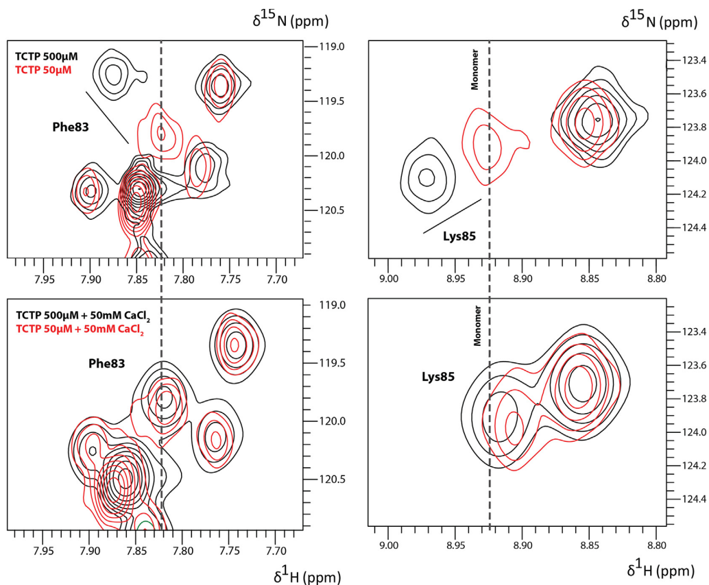
Fig. 10. NMR cross-peaks of dimer-sensitive residues Phe83 (left) and Lys85 (right) at low ( 50 \mu\text{M} ) or medium ( 500 \mu\text{M} ) concentration of protein, without (top) or with 50 \text{ mM} calcium (bottom). The NMR spectra were otherwise collected in the buffer Hepes 50 \text{ mM} (pH 7.4), 150 \text{ mM} NaCl, and 2 \text{ mM} TCEP at 298 \text{ K} .
