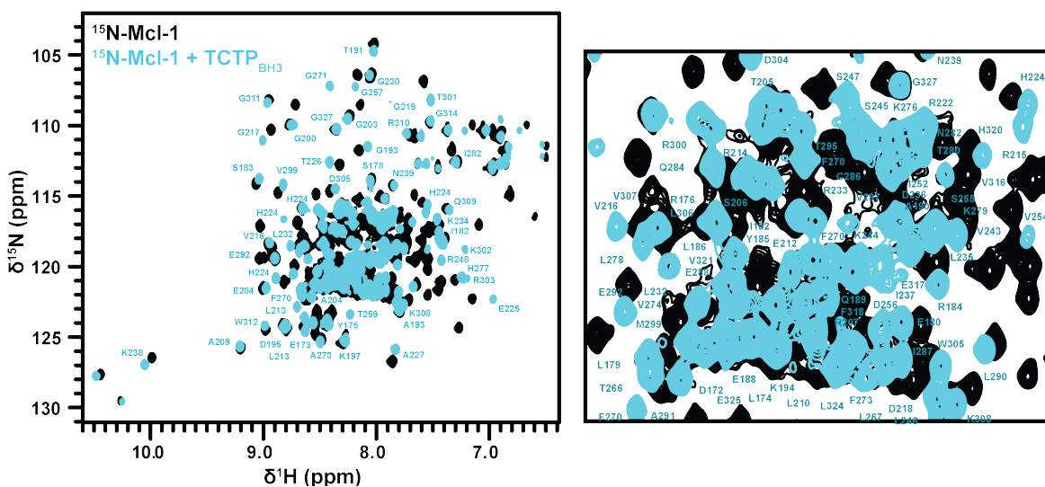
Fig. 4.16 Comparison of free Mcl-1 and in the complex with TCTP BH3 at pH 6.5. Overlay of ^1\text{H} - ^{15}\text{N} SOFAST HMQC spectra from isolated ^{15}\text{N} -Mcl-1 (100 \mu\text{M} ) (black) and upon addition of TCTP BH3 (5 eq.) (blue). Backbone assignment of bound TCTP is reported (labels). A close-up view of the central, crowded region of the spectrum is shown (right). Experiments were recorded at 950 MHz and 35 °C in the following buffer: 50 mM MES pH 6.5, 50 mM EPPS, 50 mM NaCl, 2 mM TCEP and 5% \text{D}_2\text{O} / 95 % \text{H}_2\text{O} .
