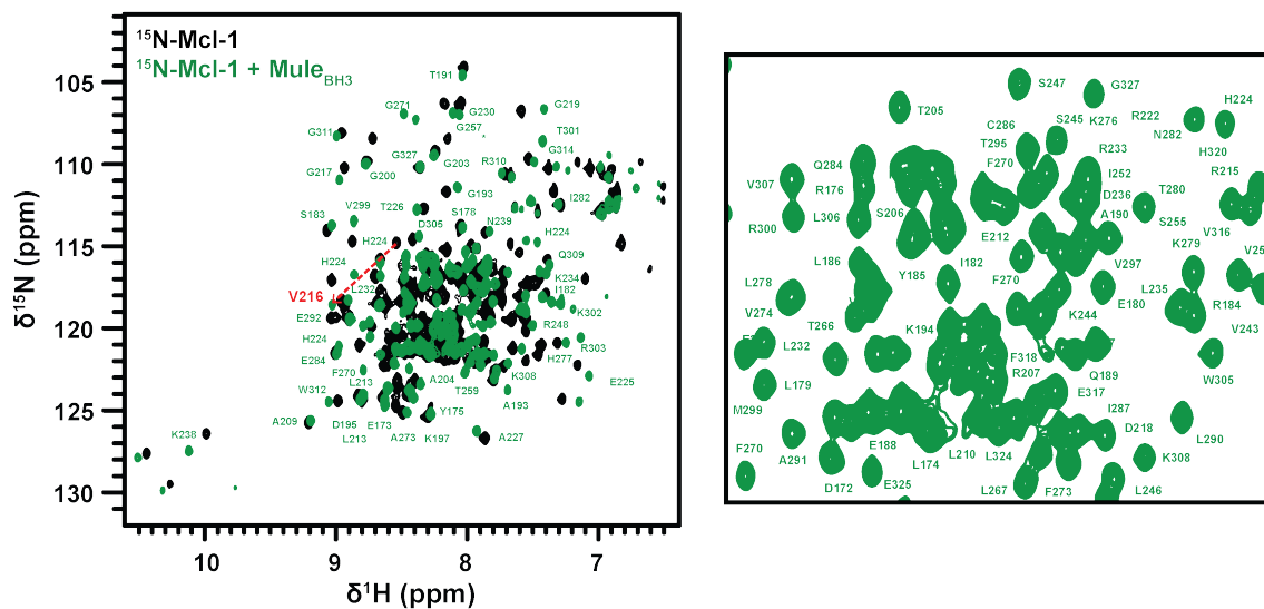
Fig. 4.32 Comparison of free Mcl-1 and in the complex with Mule BH3 . Overlay of ^1\text{H} - ^{15}\text{N} SOFAST HMQC spectra from isolated ^{15}\text{N} -Mcl-1 (100 \mu\text{M} ) (black) and upon addition of Mule BH3 (green) (2 eq.). A close-up view of the central, crowded region of Mcl-1 spectrum is shown. Backbone assignments of bound Mcl-1 are also reported (labels). Experiments were recorded at 950 MHz and 35 °C in the following buffer: 50 mM MES pH 6.5, 50 mM EPPS, 50 mM NaCl, 2 mM TCEP and 5% D 2 O / 95 % H 2 O.
