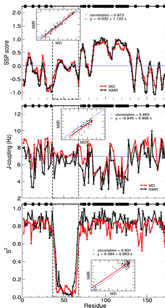
Fig. 1. Comparison between NMR (black) and noCa–noPhos MD (red) SSP scores calculated from C\alpha , C\beta and H\alpha chemical shifts (top), coupling constants ^3J_{H_N-H\alpha} (middle), and N–H bond order parameters S^2 as a function of residue number. NMR experiments were done at 50 \mu\text{M} TCTP concentration in the buffer Hepes 50 mM (pH 7.4), 150 mM NaCl, and 2 mM TCEP at 298 K.
