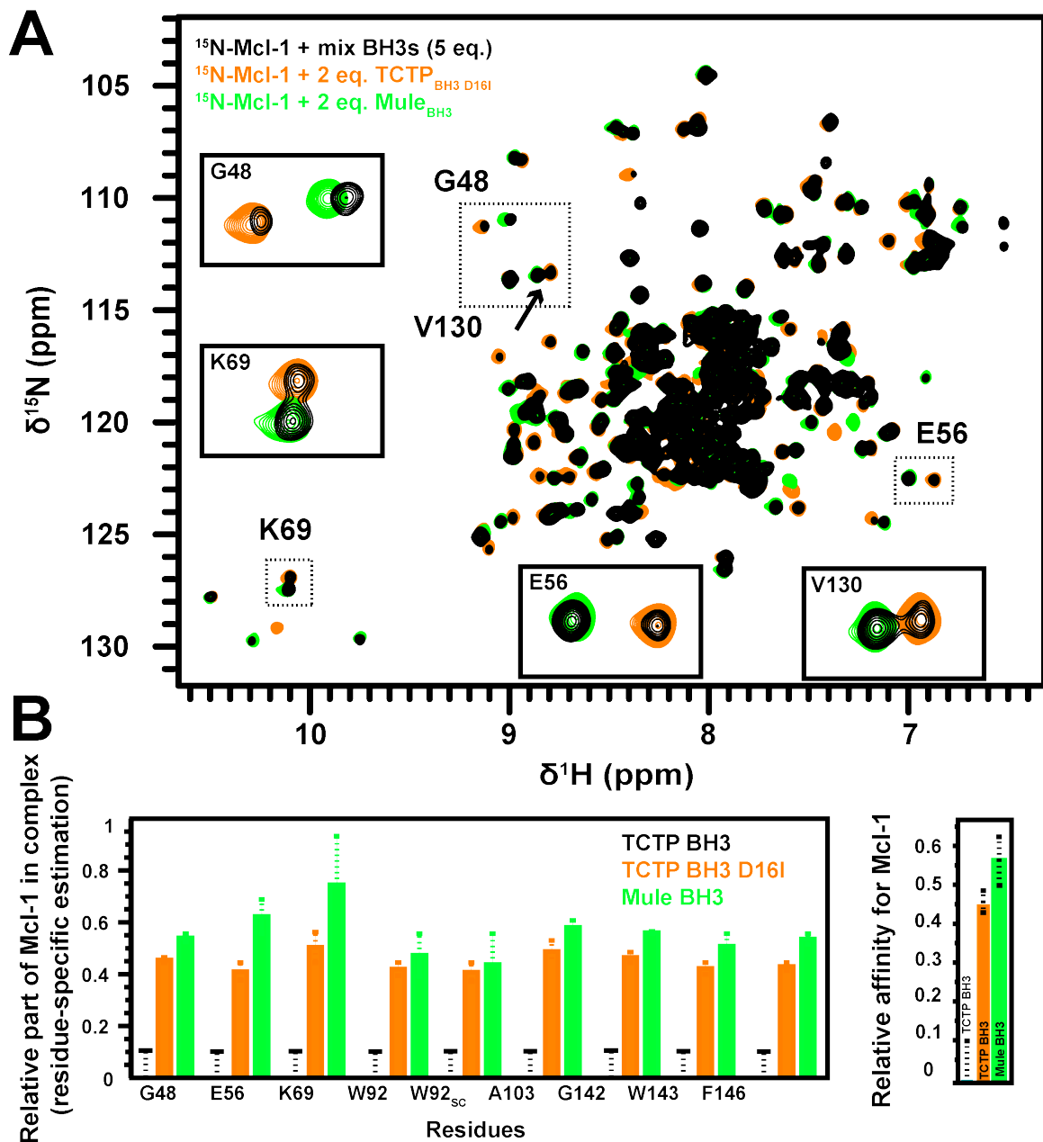
Fig. 4.37 Relative affinity of TCTP BH3, BH3D16I and Mule BH3 for Mcl-1. (A) Overlay of 1 H- 15 N SOFAST HMQC spectra from 15 N-Mcl-1 (100 μM) in complex with TCTP BH3D16I (orange), Mule BH3 (green) and with equimolar mix (5 eq. each) of the three peptides (black). (B) Relative population of 15 N-Mcl-1 bound to TCTP BH3 , TCTP BH3D16I or Mule BH3 . Ratios represent R_{Exp}/R_{Ref} , where R_{Exp} is, for example, equal to I_{bound}/I_{free} . Data are shown for all separated reported residues (left) and also the average (right). Experiments were recorded at 25 °C and 950 MHz in the following buffer: 50 mM EPPS pH 8, 50 mM NaCl, 2 mM TCEP and 5 % D 2 O / 95 % H 2 O.
