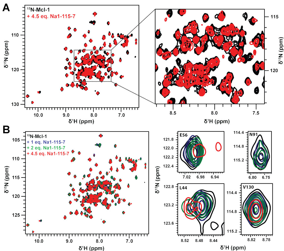
Fig. 5.18 Na-1-115-7 binds to human Mcl-1 with medium affinity. (A) Overlay of ^1\text{H} - ^{15}\text{N} SOFAST HMQC spectra from isolated Mcl-1 (50 \mu\text{M} ) (black) and in presence of Na-1-115-7 (4.5 eq.) (red). A close-up view of the central region is shown (right). (B) Overlay of SOFAST ^1\text{H} - ^{15}\text{N} HMQC spectra from isolated Mcl-1 (50 \mu\text{M} ) (black) and in presence of increasing concentrations of Na-1-115-7 (blue, green, red). A close-up view of residues experiencing spectral perturbations is shown (right). Experiments were recorded at 950 MHz and 25 ^\circ\text{C} in the following buffer: 20 mM \text{NaPO}_4 pH 7.4, 50 mM NaCl, 2 \mu\text{M} EDTA, 2 mM TCEP, 0.005% pluronic acid, 3.5% DMSO, and 5% \text{D}_2\text{O} / 95 % \text{H}_2\text{O} .
