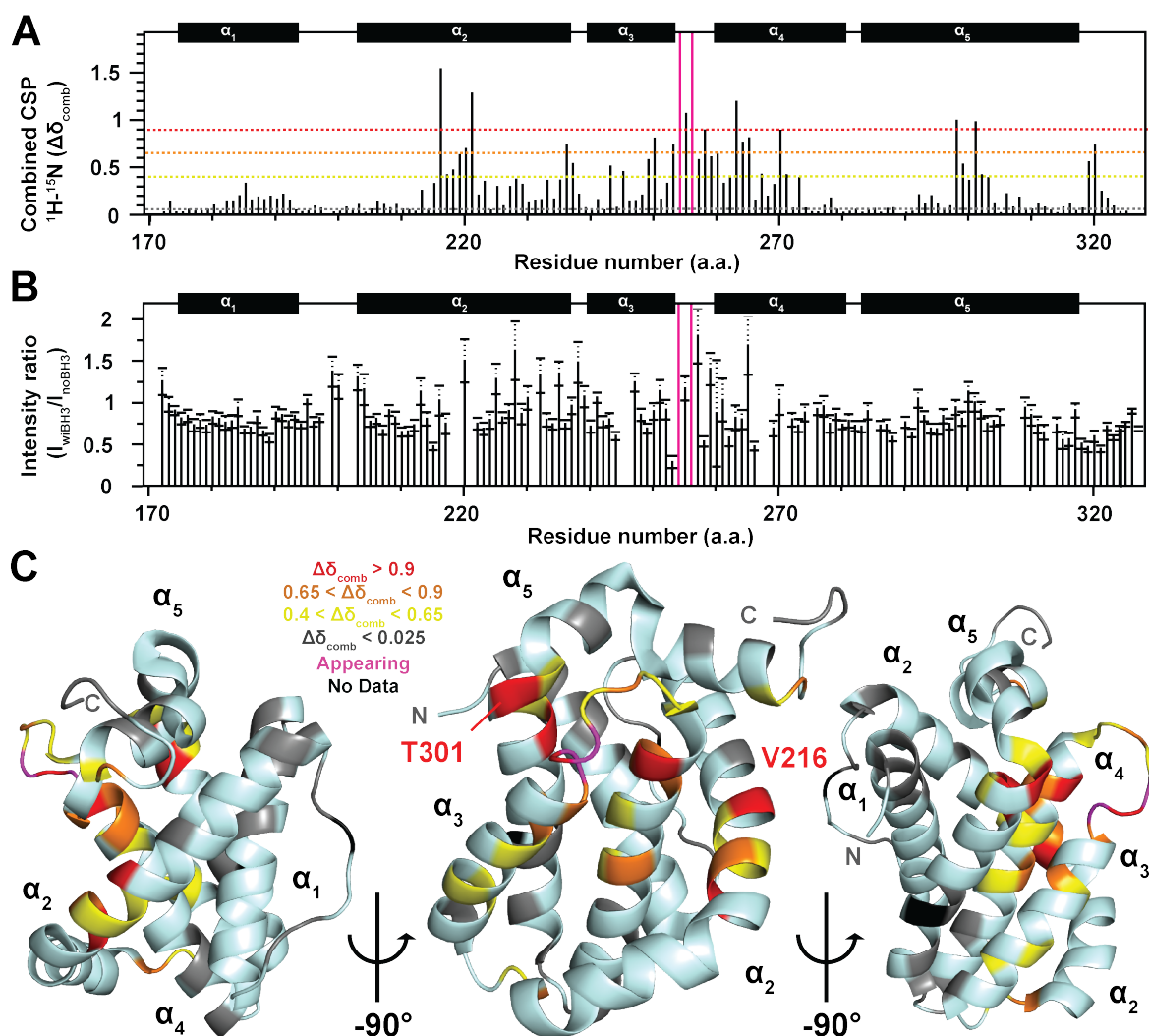
Fig. 4.31 NMR mapping of TCTP BH3D16I binding site in Mcl-1. (A) Combined {}^1\text{H}-{}^{15}\text{N} chemical shift perturbations and (B) intensity ratios computed between {}^1\text{H}-{}^{15}\text{N} SOFAST HMQC spectra from isolated {}^{15}\text{N} -Mcl-1 (100 \mu\text{M} ) and upon addition of TCTP BH3D16I (5 eq.). Appearing (magenta bar) residues upon complex formation are shown. Dotted colored bars indicate thresholds for mapping. (C) Mapping of combined {}^1\text{H}-{}^{15}\text{N} chemical shift perturbations (red \geq 0.9 , 0.9 \geq \text{orange} \geq 0.65 , 0.65 \geq \text{yellow} \geq 0.4 , 0.025 \geq \text{grey} ) and {}^1\text{H}-{}^{15}\text{N} signal appearing (magenta) on Mcl-1 structure. Residues for which no data are available (overlap, line broadening...) are highlighted (black).
