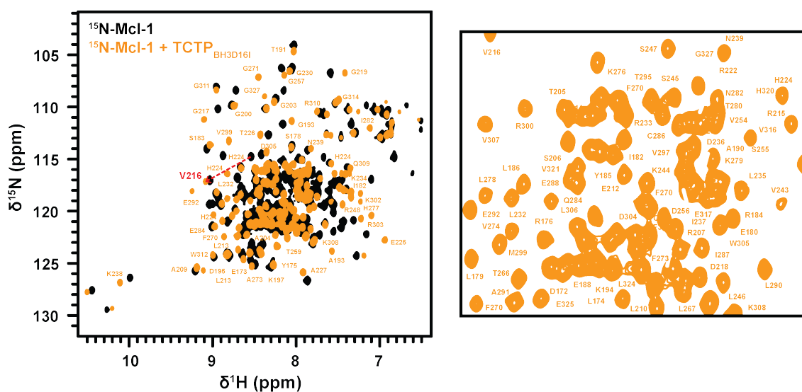
Fig. 4.30 Comparison of free Mcl-1 and in the complex with \text{TCTP}_{\text{BH3D16I}} . Overlay of ^1\text{H} - ^{15}\text{N} SOFAST HMQC spectra from isolated ^{15}\text{N} -Mcl-1 (100 \mu\text{M} ) (black) and upon addition of \text{TCTP}_{\text{BH3D16I}} (3 eq.) (orange). A close-up view of the central, crowded region of Mcl-1 spectrum is shown (right). Backbone assignments of bound Mcl-1 are also reported (labels). Experiments were recorded at 950 MHz and 35 ^\circ\text{C} in the following buffer: 50 mM MES pH 6.5, 50 mM EPPS, 50 mM NaCl, 2 mM TCEP and 5% \text{D}_2\text{O} / 95 % \text{H}_2\text{O} .
