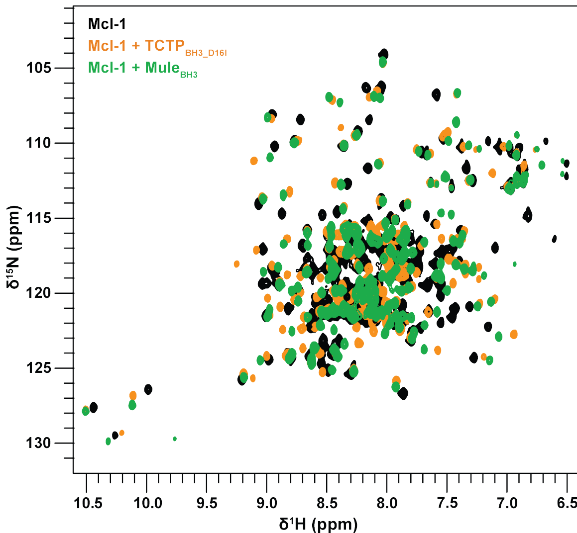
Fig. 16 Comparison between free Mcl-1 and in complex with TCTP BH3D16I or Mule BH3 . Overlay of ^1\text{H} - ^{15}\text{N} SOFAST HMQC spectra from isolated Mcl-1 (100 \mu\text{M} ) (black) and in complex with TCTP BH3D16I (yellow) or with Mule BH3 (green). Experiments were recorded at 950 MHz and 308 K in the following buffer: 50 mM MES pH 6.5, 50 mM EPPS, 50 mM NaCl, 1 mM TCEP in 95 % \text{H}_2\text{O} / 5 % \text{D}_2\text{O} .
