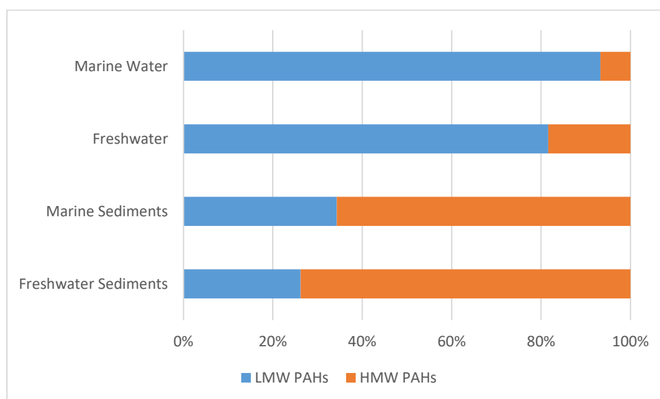
Figure 4.4: Distribution of HMW and LMW PAHs in dissolved and sedimentary phases from marine and freshwater systems.
