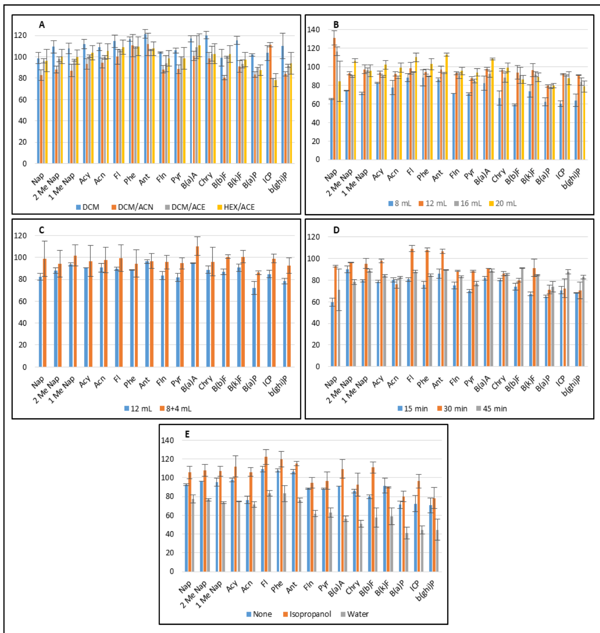
Figure S.3.3: Extraction recoveries obtained from spiked soils at 150 ppb for optimization of extraction parameters: (A) extraction solvent, (B) Extraction volume, (C) Solvent fractionation, (D) Extraction time and (E) water and isopropanol effect.
