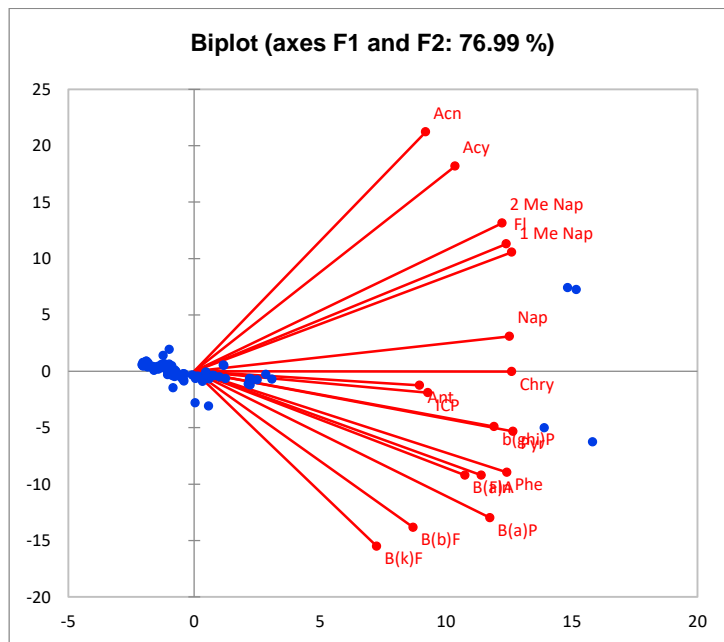
Figure 3.1: Principal Component Analysis (PCA) plot showing the PAHs variation among 100 soil samples. Vectors indicate the direction and strength of each PAHs to the overall distribution. Dots correspond to soil samples. The first two principal axes explained 76 % of the variance.
