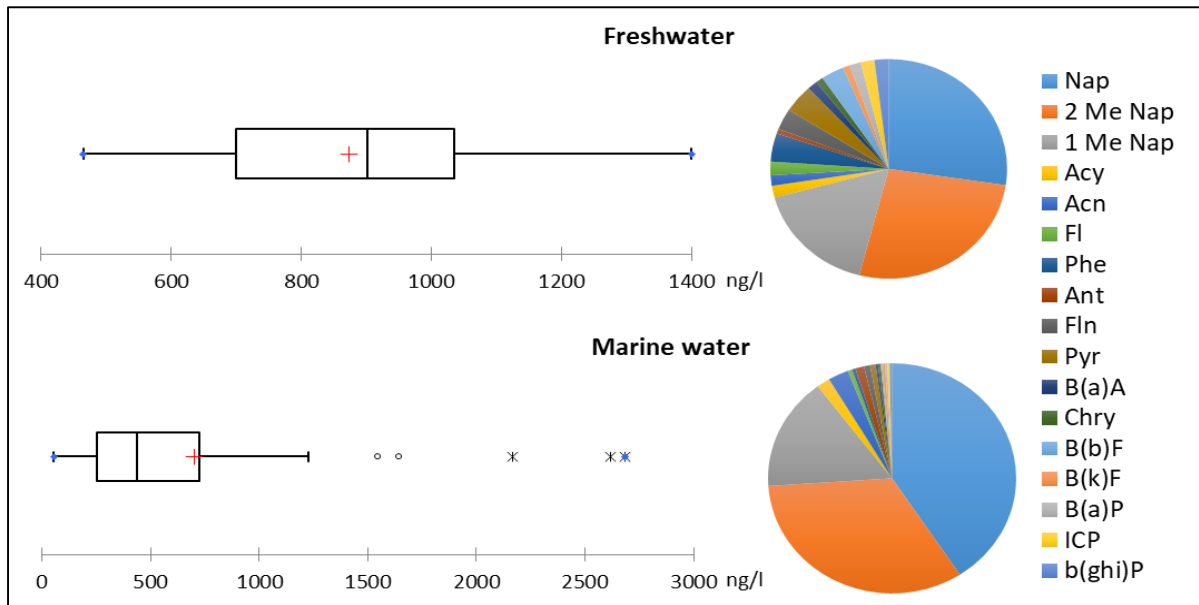
Figure 4.2: The descriptive summary of the total contamination with PAHs in aqueous phase and the contribution of the 17 PAHs.
