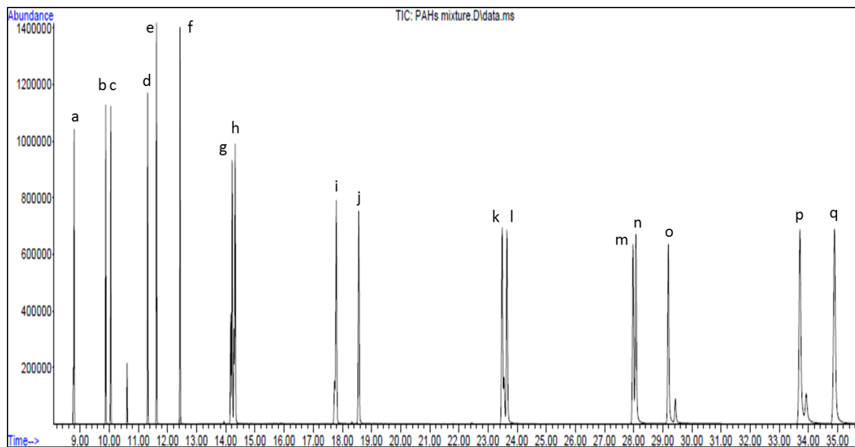
Figure S.3.2: Obtained chromatogram of the 17 PAHs: (a) Nap, (b) 2 Me Nap, (c) 1 Me Nap, (d) Acy, (e) Acn, (f) Fl, (g) Phe, (h) Ant, (i) Fln, (j) Pyr, (k) B[a]A, (l) chry, (m) B[b]F, (n) B[k]F, (o) B[a]P, (p) ICP, (q) b[ghi]P.
