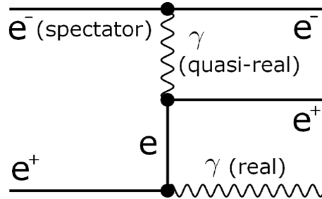
Figure 4.1: Radiative Bhabha scattering process at vanishing photon scattering angle.
