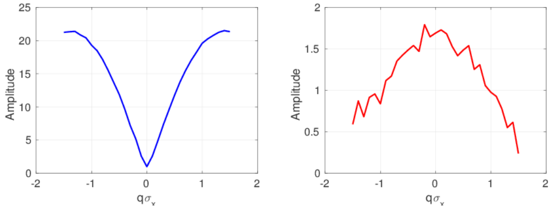
Figure 3.4: Magnitude of peaks at the fundamental (left) and twice the fundamental (right) frequency as a function of the offset between the two beams in the case of a dithering amplitude of 0.1\sigma_x and a relative precision of the fast luminosity signals of 1% per ms.
