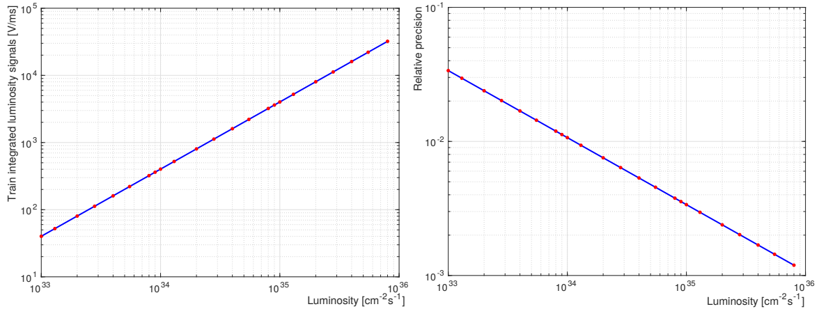
Figure 4.23: Example of simulated train integrated luminosity signal (left) and relative precision (right) at 1 kHz as a function of actual luminosity.
