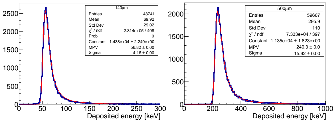
Figure 3.9: Landau distribution of deposited energy in the diamond detector (left: with thickness of 140 \mu\text{m} ; right: with thickness of 500 \mu\text{m} ) by 1.6 MeV electrons, based on simulation by Geant4.
