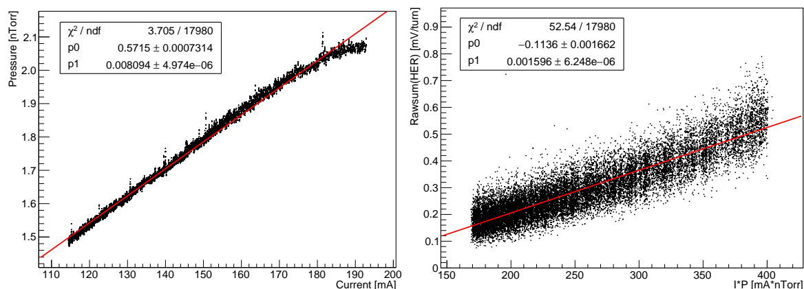
Figure 5.16: Vacuum pressure as a function of the beam current in the HER on the left and the HER signal as a function of the product of beam current and vacuum pressure on the right.
