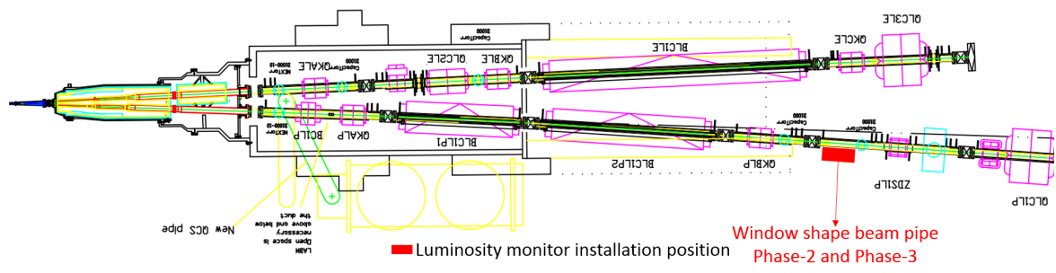
Figure A.4: The installation position of our luminosity monitor in the LER, about 10 m downstream of the IP.
