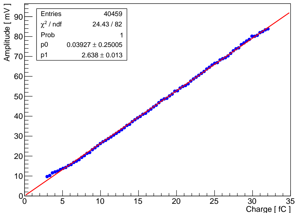
Figure 3.17: Relationship between signal amplitude and charge generated in the diamond detector with thickness 140 \mu\text{m} coupled with a broadband current amplifier.
