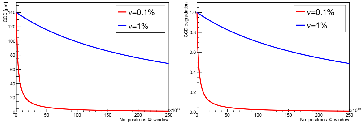
Figure 4.36: The CCD (on the left) and normalized CCD degradation (on the right) of the sCVD diamond detector with thickness of 140 \mu\text{m} as a function of the number of the Bhabha positrons lost on the 45^\circ window in the LER.
