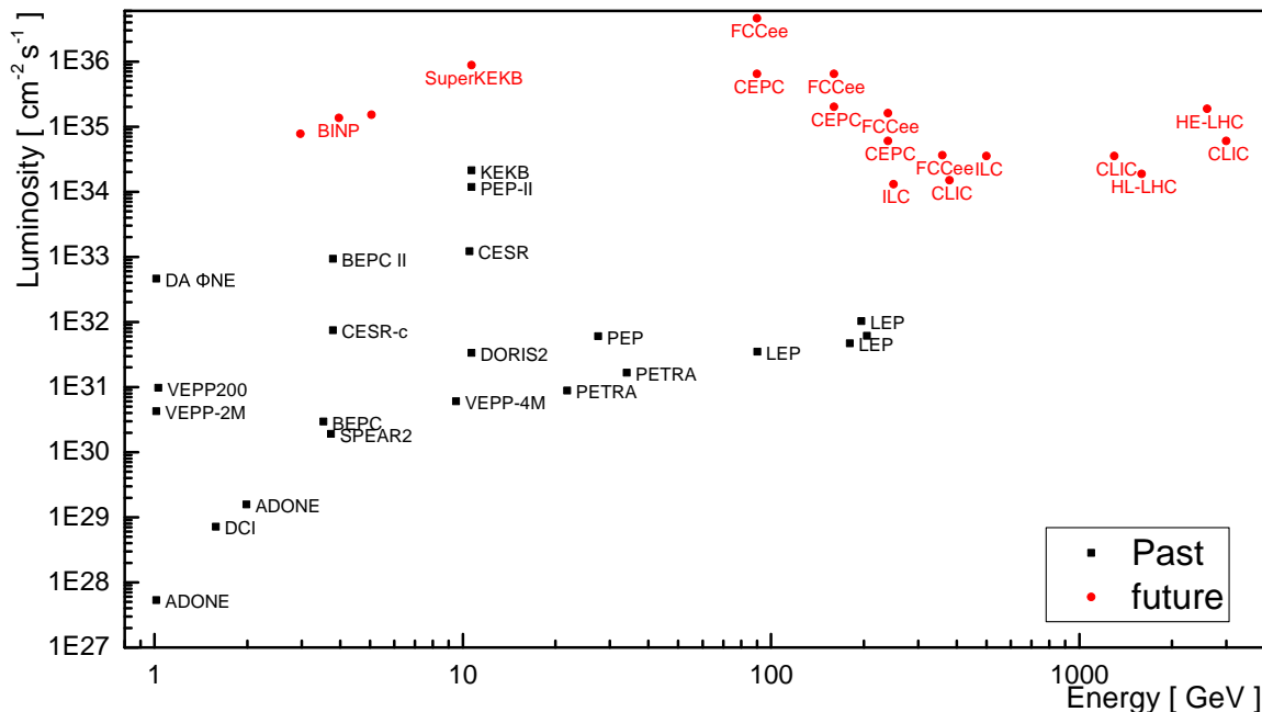
Figure 1.2: Luminosity as function of collision C.M.S energy for past and future particle colliders. Both CEPC and FCCee will be operated in Z, W, and Higgs modes.
