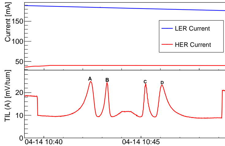
Figure 5.24: TIL signal response during the sampling phase scan with the phase shifter for the diamond detector with thickness of 140 \mu\text{m} coupled with a C2 broadband current amplifier, located at position A in the LER.
