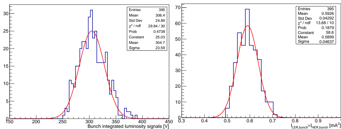
Figure 5.34: Histogram of the Bunch Integrated Luminosity signals displayed in Figure 5.33 in the left and the product of the LER and HER bunch currents in the right.
