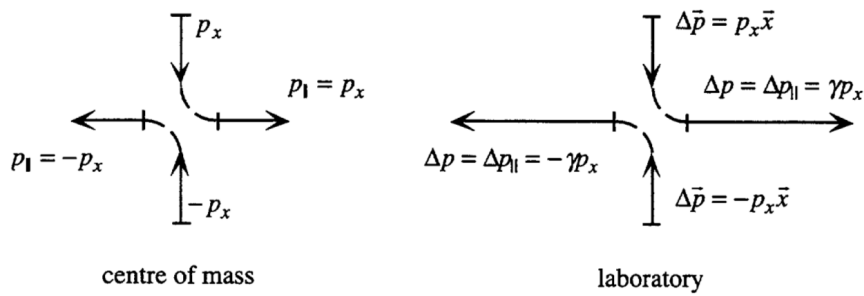
Figure 4.25: A typical example of Touschek scattering process in CMS and laboratory systems.
