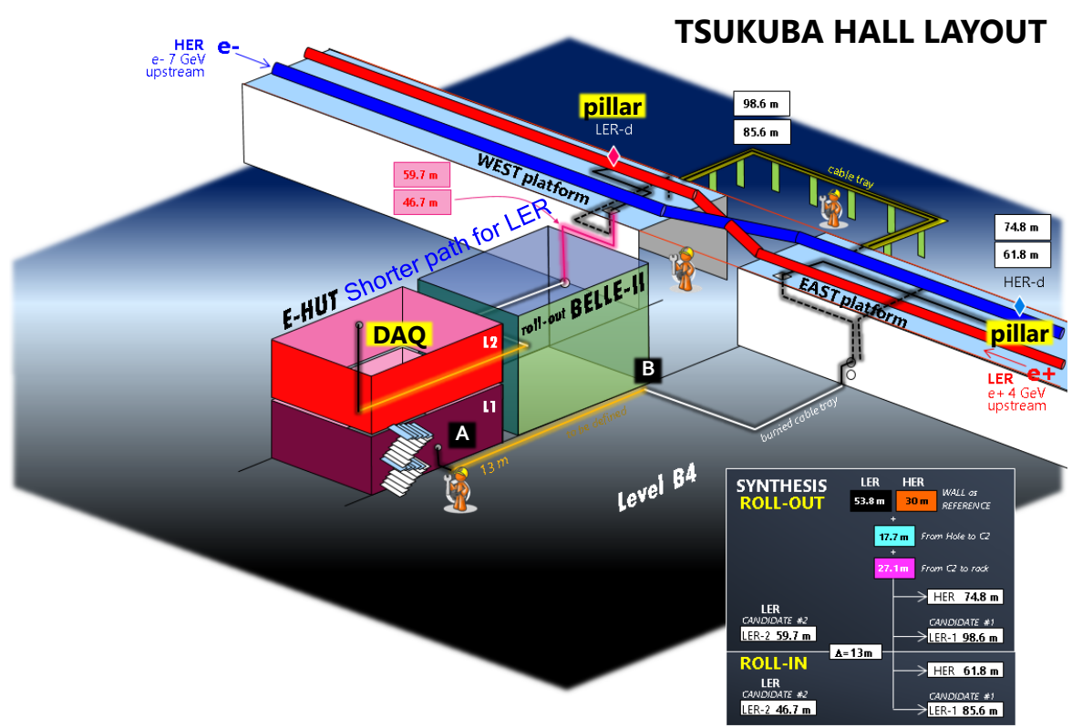
Figure A.3: The layout of the Tsukuba hall showing the Belle II detector with its Electronics-Hut and the cabling path for the diamond detectors in LER and HER.
