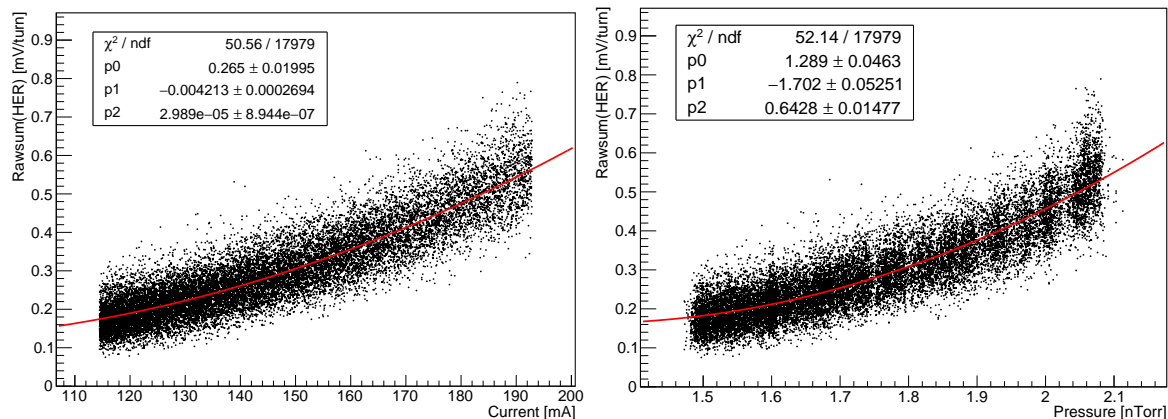
Figure 5.15: Example of HER signals as a function of machine parameters: beam current (left) and vacuum pressure (right).
