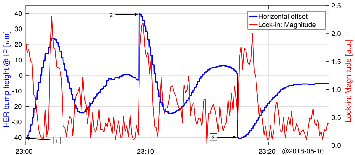
Figure 5.37: Dithering feedback system test with deliberately introduced horizontal offsets by using the LumiBelle2 signal as input to the lock-in amplifier.
