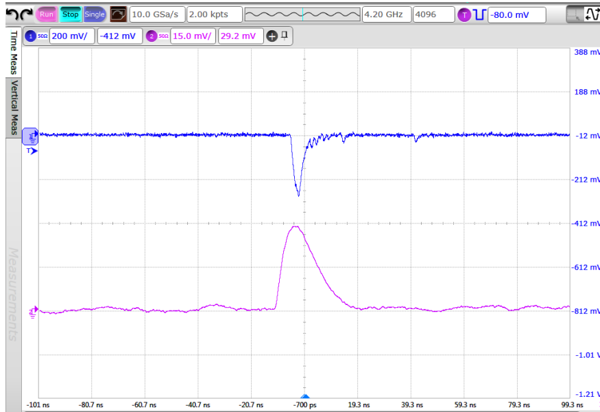
Figure 3.13: Screen shot from the oscilloscope showing the signals from the diamond detector coupled with a fast charge amplifier (pink) and from the scintillator used for triggering (blue).
