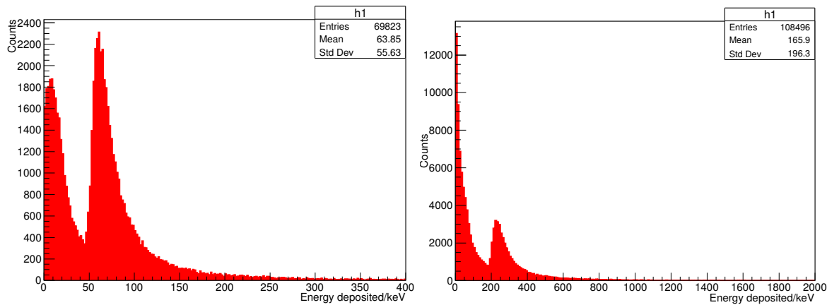
Figure 4.15: Histogram of the deposited energy in the diamond detector for each charged secondary: left for 140 \mu\text{m} , right for 500 \mu\text{m} .
