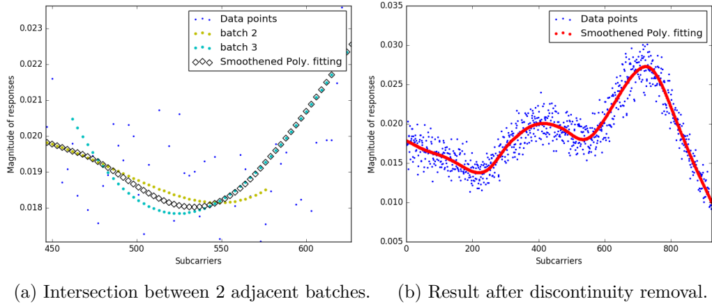
Figure 4.7: Discontinuity Removal
