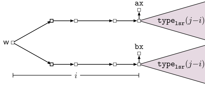
Figure 9.10: Schema of a pointed forest (\mathcal{K}, w) satisfying \text{fork}_j^i(\text{ax}, \text{bx}) .
