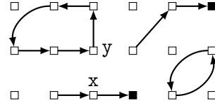
Figure 2.5: A memory state satisfying \forall x \neg (\_ \hookrightarrow x * \_ \hookrightarrow x) .
