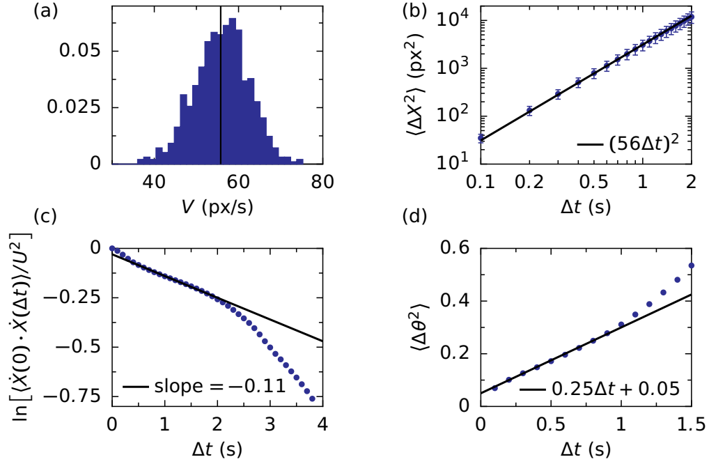
Figure 11.2: Determination of the experimental parameters. 670 particles are tracked for 35 frames on average. (a) Histogram of the average velocities of the particles, the vertical black line is the mean. (b) Mean square displacement. Error bars show the distribution over different particles. (c) Velocity autocorrelation. (d) Mean square angle. (No error bars are given for the last two observables since we consider all available data points for detected trajectories of heterogeneous lengths.)
