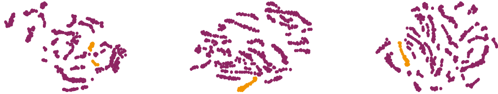
(a) InceptionResnet
