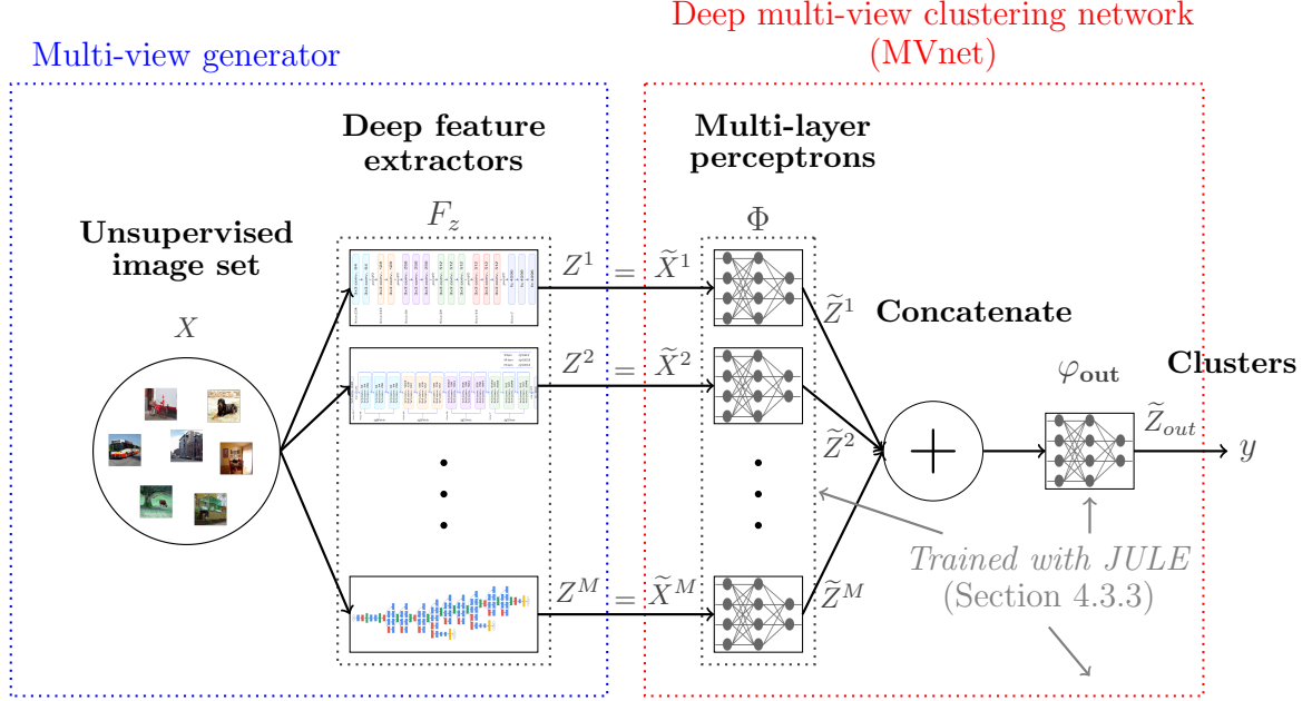
Figure 4.1: Proposed multi-view generation + deep multi-view clustering (DMVC) approach to solve the Image Clustering problem.
