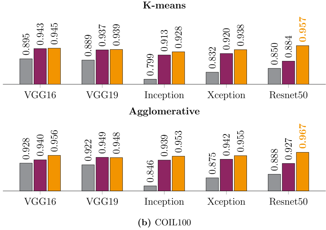
Figure C.1: NMI scores on natural object recognition datasets.
