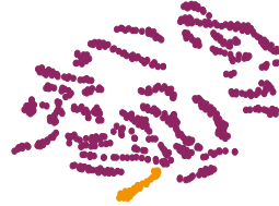
(b) VGG16
