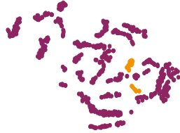
(a) InceptionResnet
