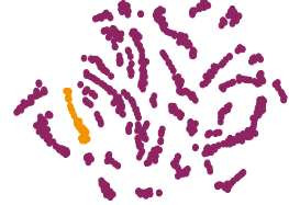
(c) Densenet121
