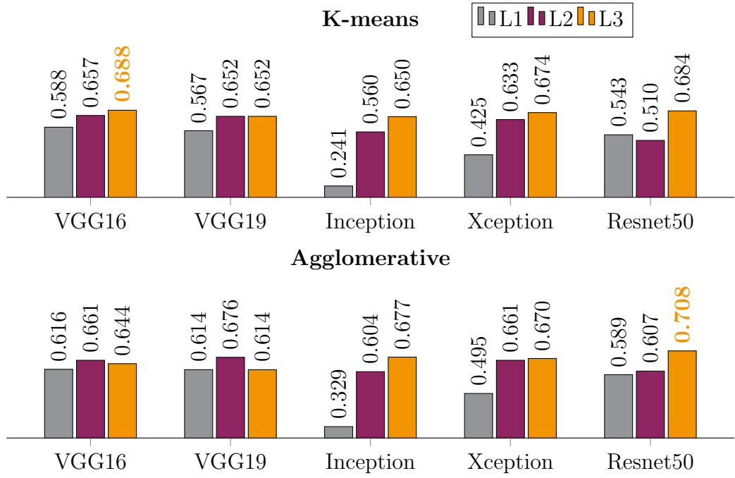
(a) Flowers
