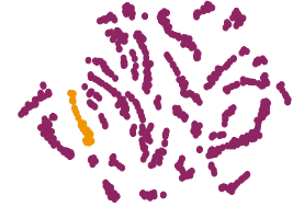
(c) Densenet121
