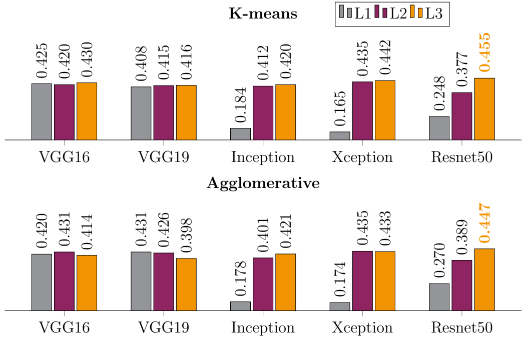
(a) Archi
