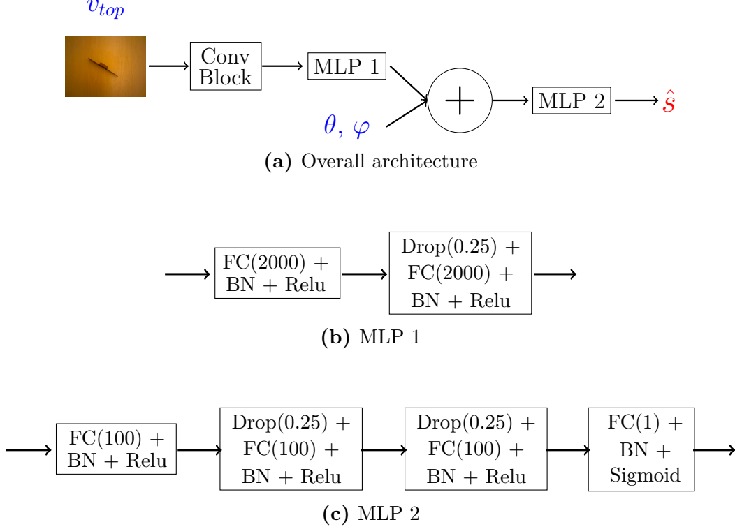
Figure 6.5: Proposed SV-net architecture. Inputs are in blue and outputs in red. The Conv Block is the convolutional part of VGG19 (until “block4_pool” layer).
