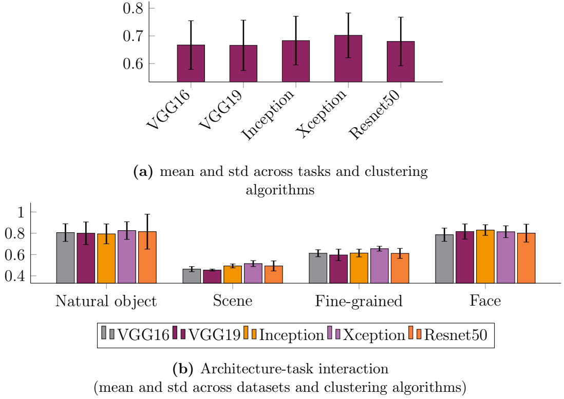
Figure 3.4: Influence of the CNN architectures (L3) on the clustering results (NMI).
