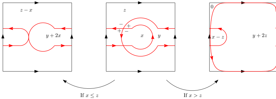
Figure 3.8: In the middle: a self-overlapping loop on the torus. It can be transformed into the one on the left if the area z is large enough to ‘absorb’ the area x , otherwise it will be stuck in the configuration in the right.
