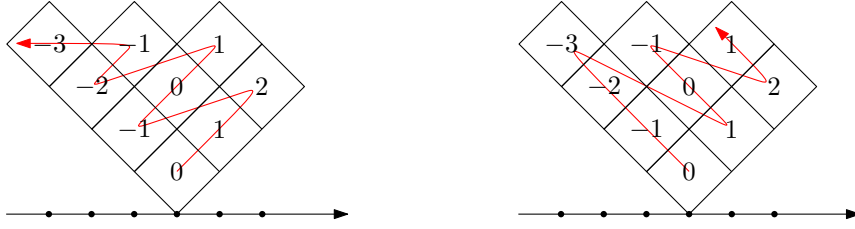
Figure 2.4: Two ways of listing the contents of the boxes of the diagram (3, 3, 2, 1) .
