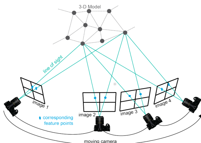
FIGURE 3.1 – Exemple de processus SfM (source UNAVCO)
