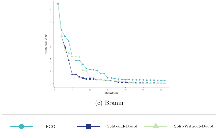
Figure 5.4: Comparison of 3 optimization strategies. Mean over N_{seed} of the best current value as a function of the number of iterations.
