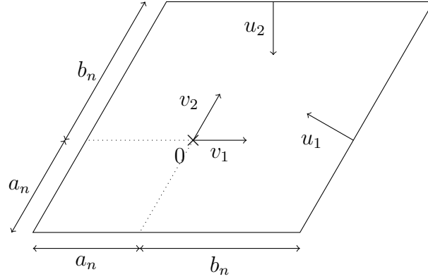
Figure 1.3: \mathcal{P}_n .
