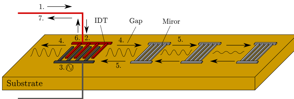
Figure 7.2: SAW filter working scheme through the delay line filter example
