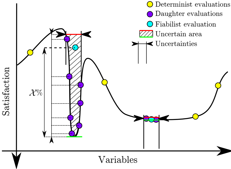
Figure 6.1: The fiabilist evaluation
