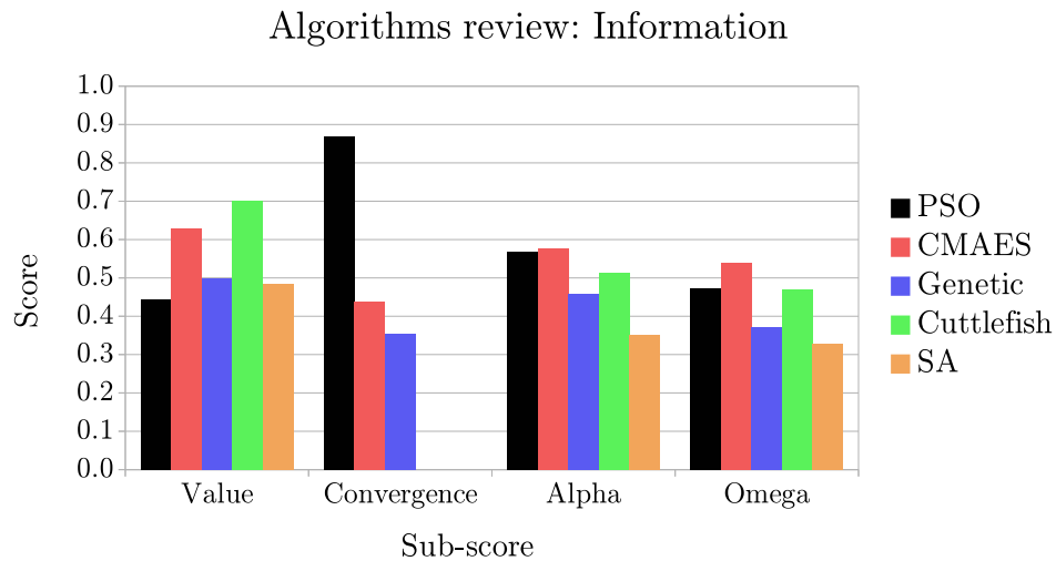
Figure 4.8: Meta-heuristic algorithms analysis: Information sub-scores
