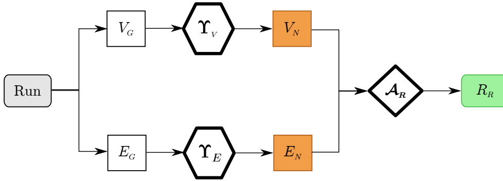
Figure 4.3: Run results computation workflow
