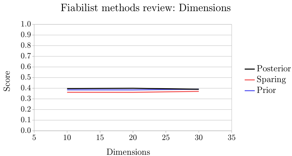
Figure 6.6: Fiabilist methods review: Average dimension sub-scores
