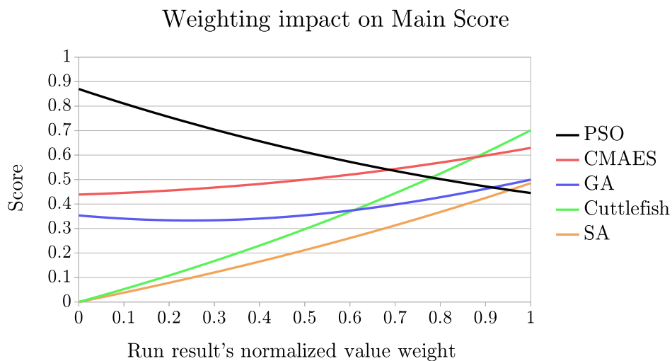
Figure A.2: Impact of run result aggregation's V_N 's weight on Main score for tested algorithms
