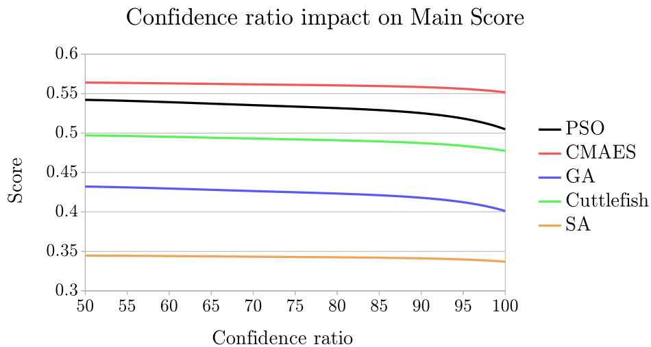
Figure A.3: Impact of confidence limit ratio on Main score for tested algorithms
