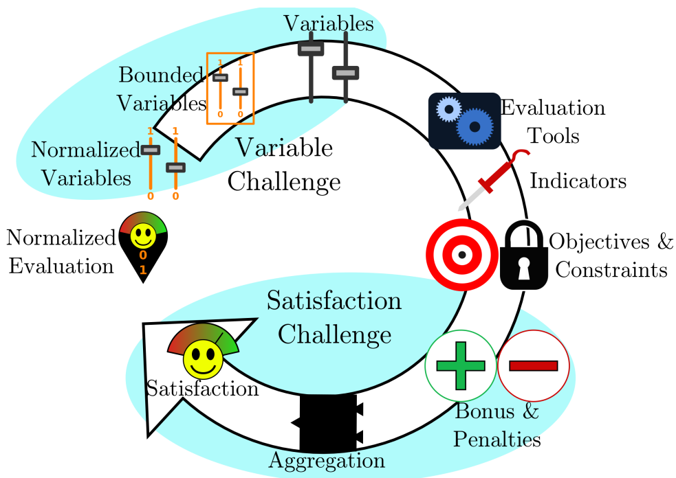
Figure 3.1: NE approach workflow
