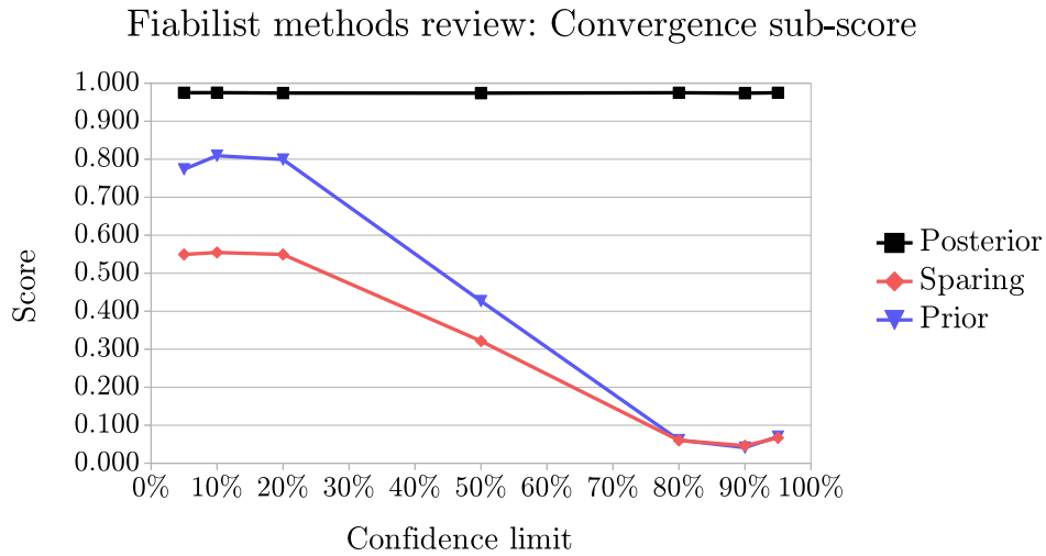
Figure 6.11: Fiabilist methods review: Convergence sub-score with respect of the confidence limit
