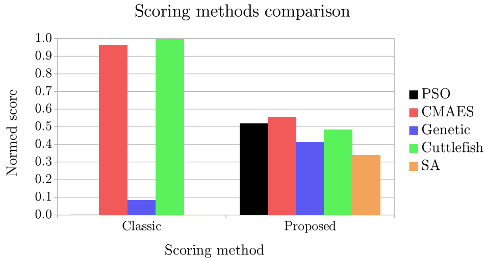
Figure 4.7: Scores from the CEC benchmark and the proposed benchmark for classical metaheuristic algorithms
