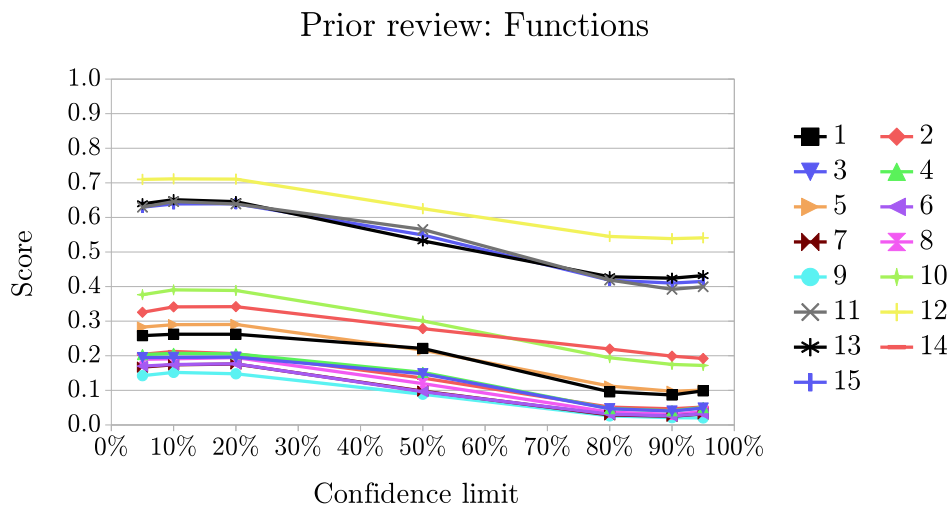
Figure 6.12: The influence of the confidence limit on the function sub-scores obtained by the prior function
