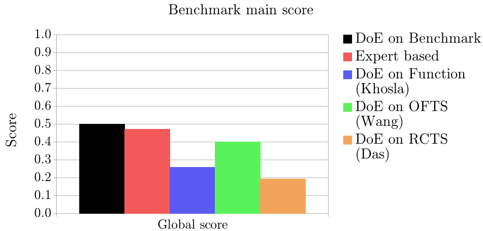
Figure 5.6: Settings review: global score
