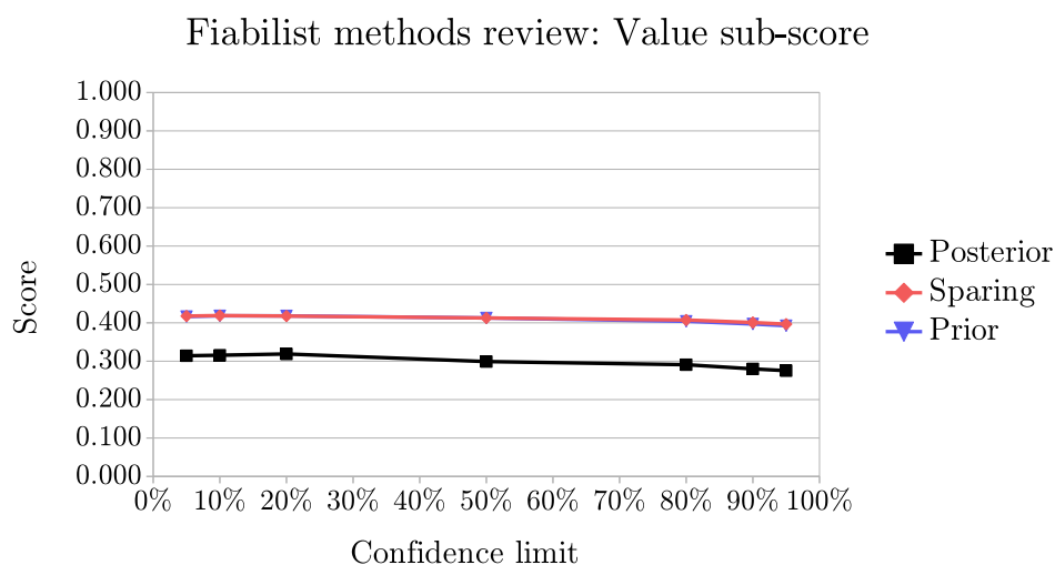
Figure 6.10: Fiabilist methods review: Value sub-score with respect of the confidence limit
