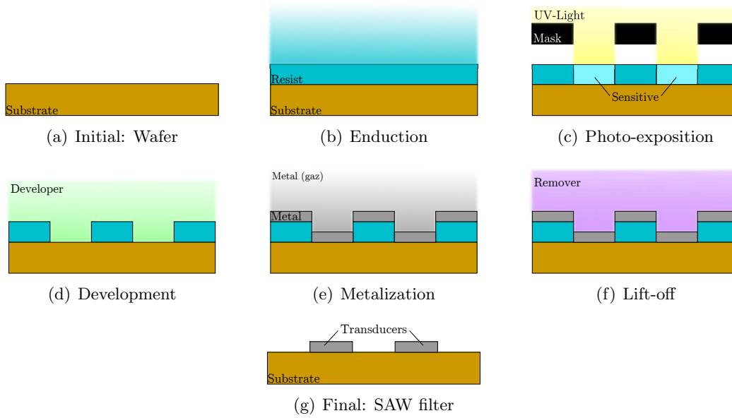
Figure 7.6: Lift-off process in the application case
