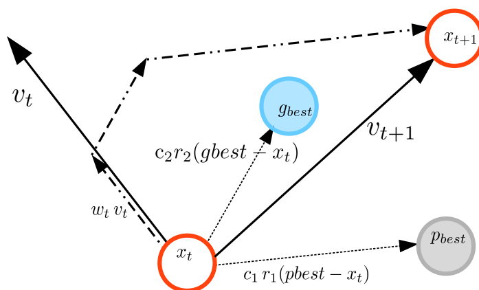
Figure 1.6: PSO particles displacement
