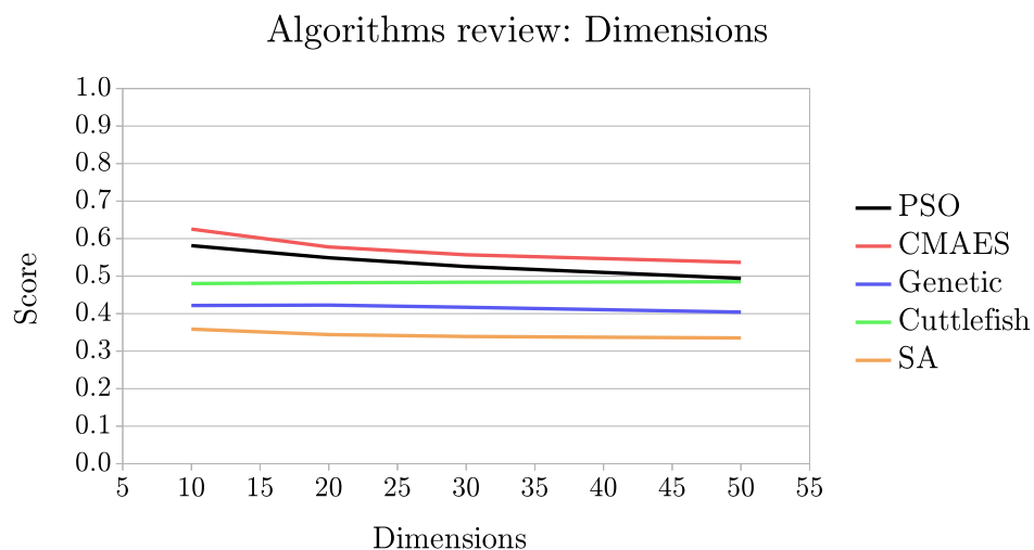
Figure 4.9: Meta-heuristic algorithms analysis: Dimensions scores
