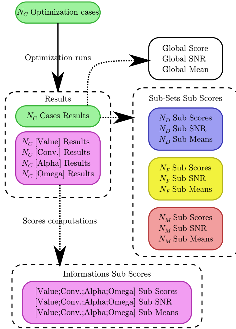
Figure 4.2: Benchmark scores work-flow
