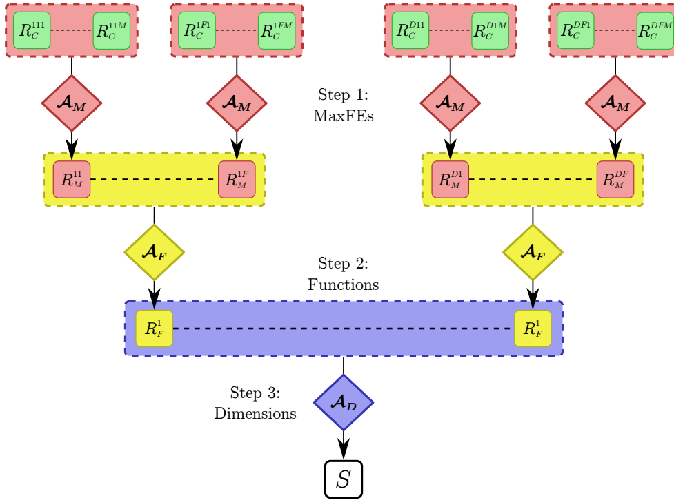
Figure 4.6: Global score computation flowchart
