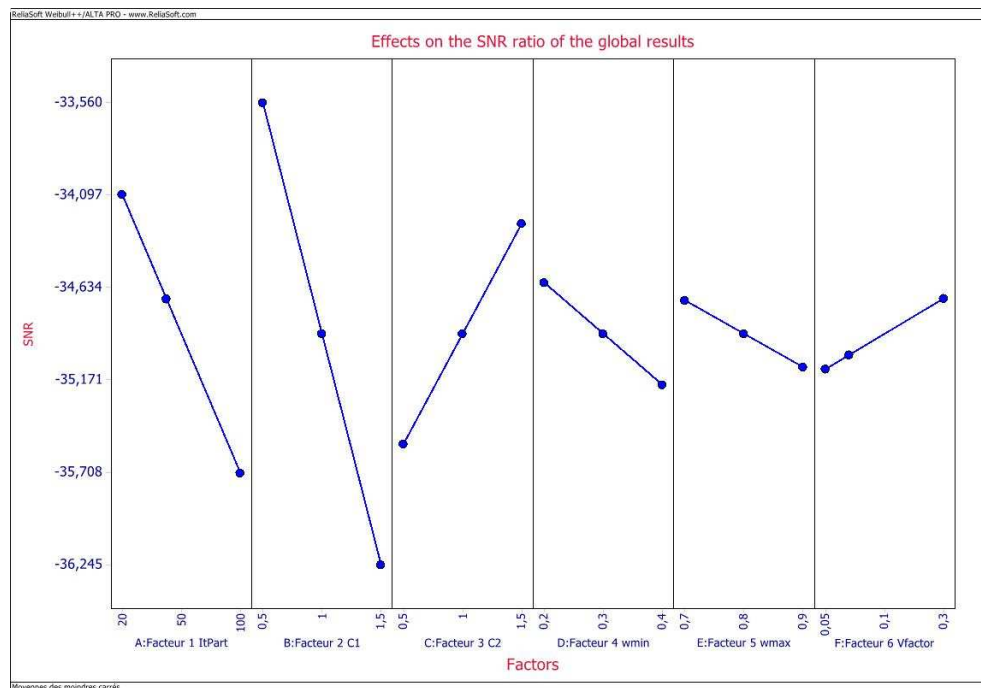
Figure 5.2: DOE factors' SNR Response graph
