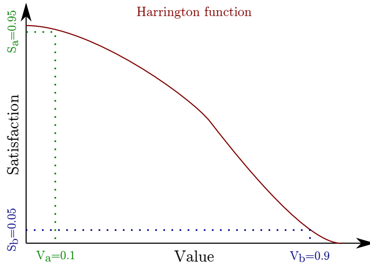
Figure 4.4: Harrington normalization function in 'the lower the better case' with pre-defined settings
