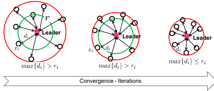
Figure 1.7: PSO radius stopping criterion
