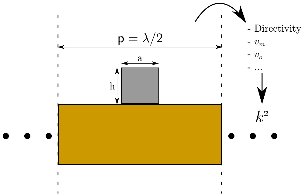
Figure 7.4: SAW filter modeling - unit element simulation
