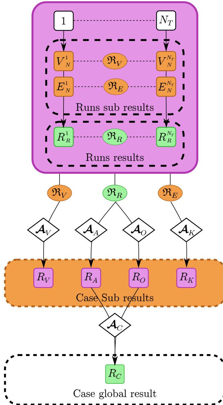
Figure 4.5: Optimization case results workflow
