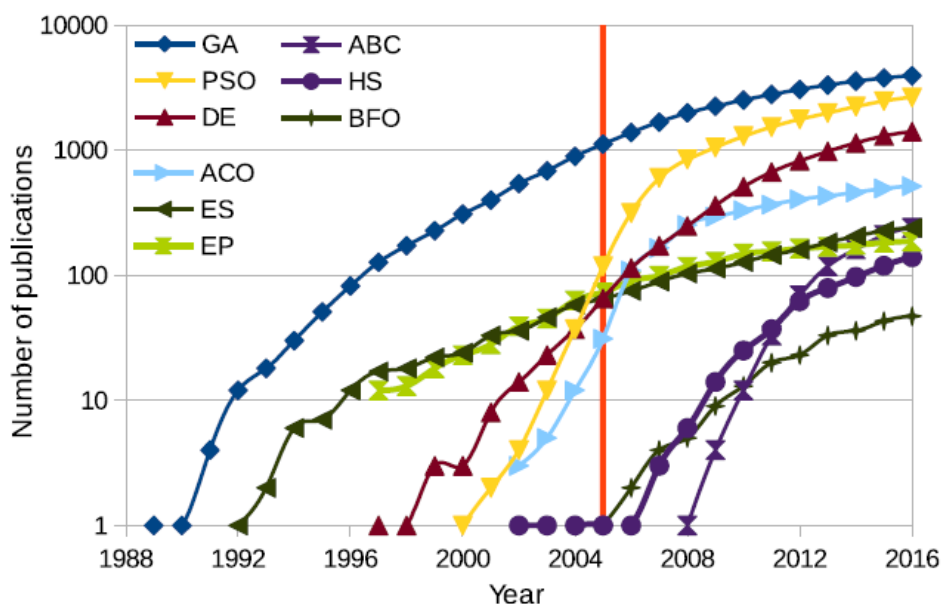
Figure 1.5: Evolution of the number of publications related to meta-heuristic algorithms [13]
