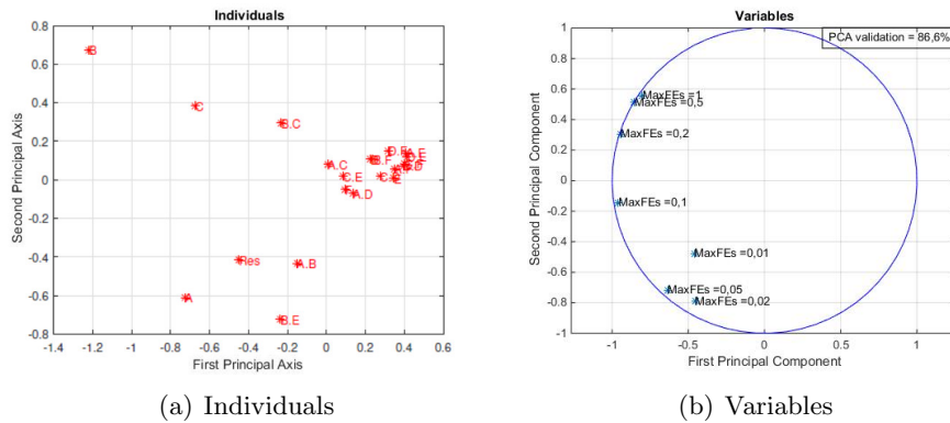
Figure 5.5: PCA in case 3 - DoEs with fixed MaxFEs
