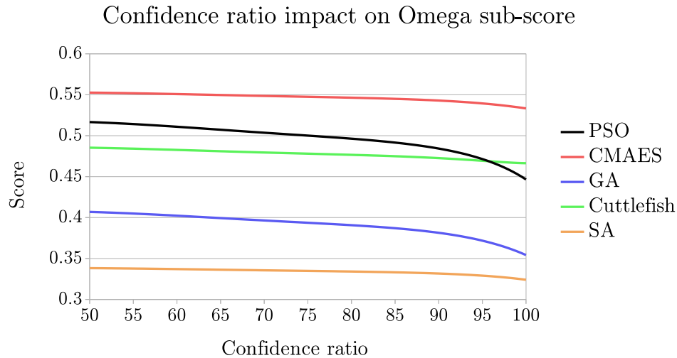
Figure A.4: Impact of confidence limit on Omega sub-score for tested algorithms
