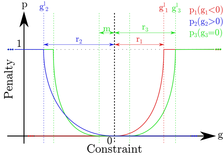
Figure 3.2: Penalty in function of constraint for different penalty types: Lower, Higher, Equal
