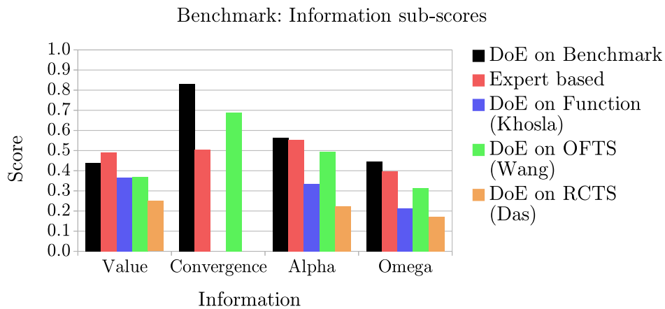
Figure 5.7: Settings review: information sub-scores
