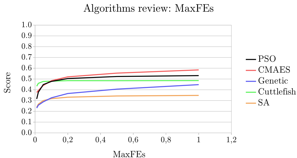
Figure 4.11: Meta-heuristic algorithms analysis: MaxFEs scores
