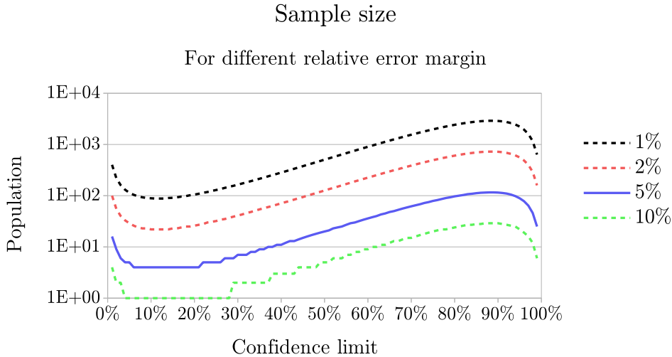
Figure 6.2: Sample size with respect to the confidence limit for different relative error margins
