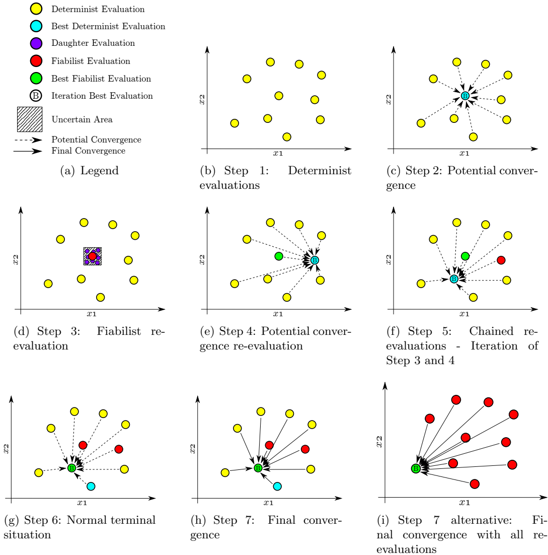
Figure 6.3: The SFO method scheme - Pictured in the PSO algorithm case
