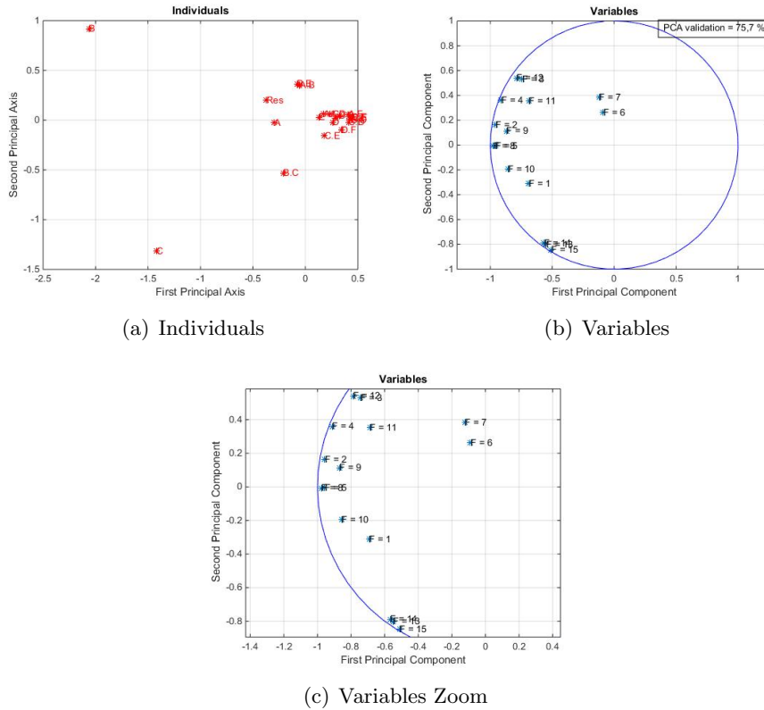
Figure 5.4: PCA in case 2 - DoEs with fixed functions
