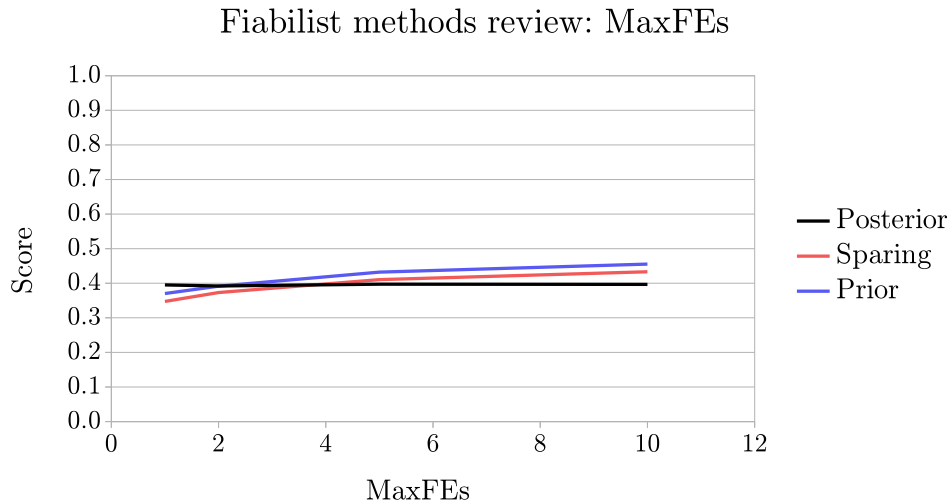
Figure 6.8: Fiabilist methods review: Average MaxFEs sub-scores
