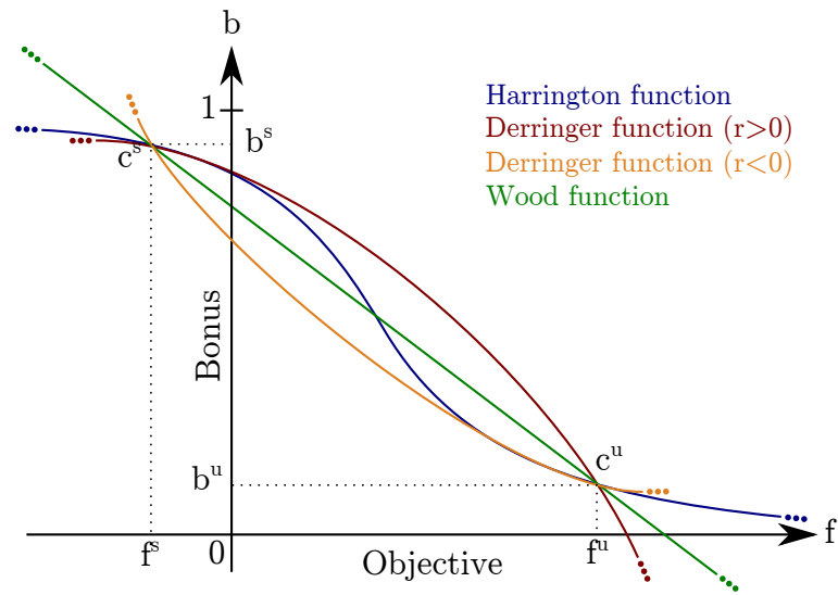
Figure 3.3: Satisfaction functions in an objective minimization case with a linear scale
