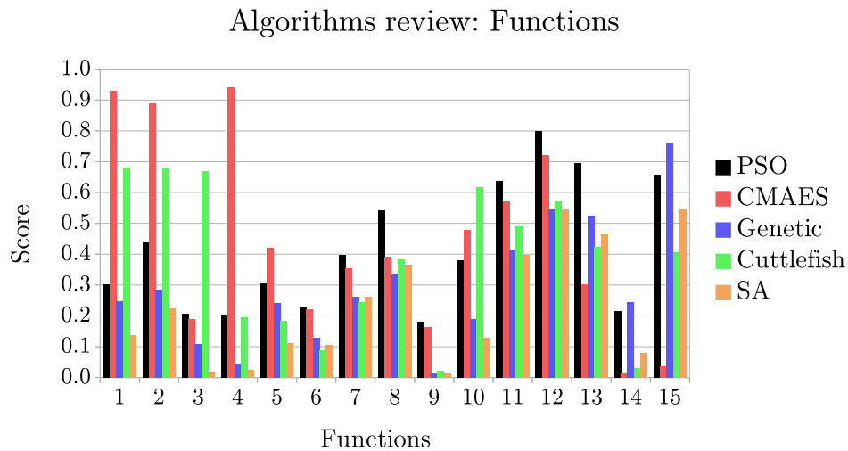
Figure 4.10: Meta-heuristic algorithms analysis: Functions scores
