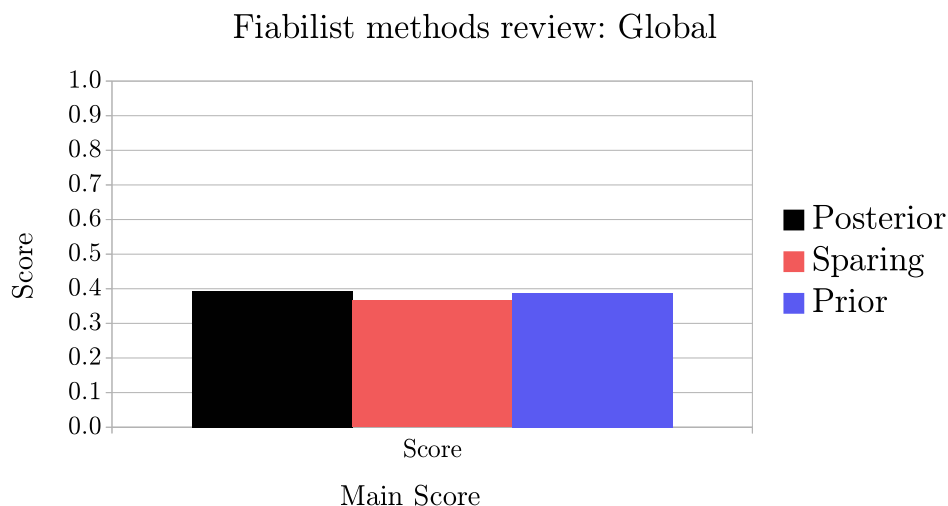
Figure 6.4: Fiabilist methods review: Average global scores
