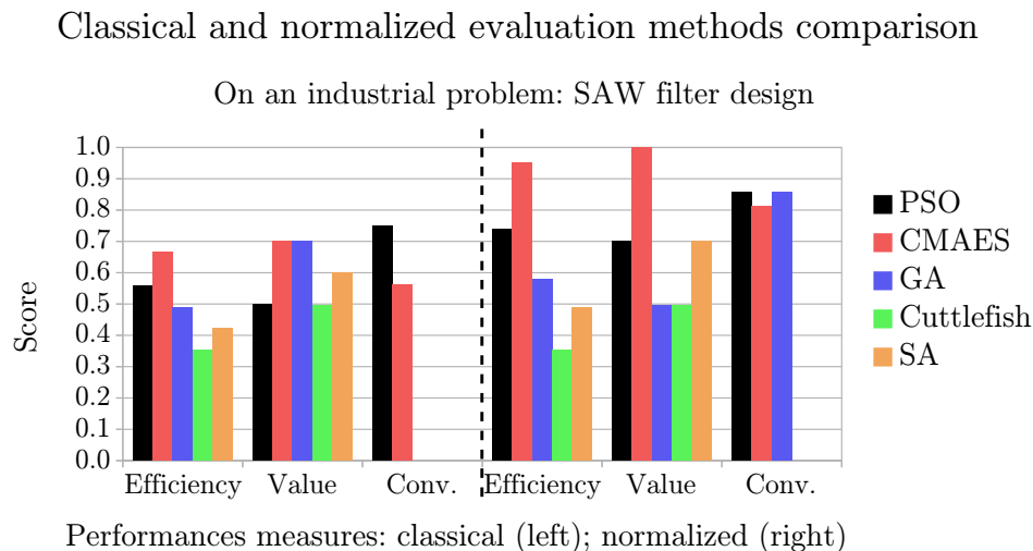
Figure 3.4: Evaluation methods review on an industrial case
