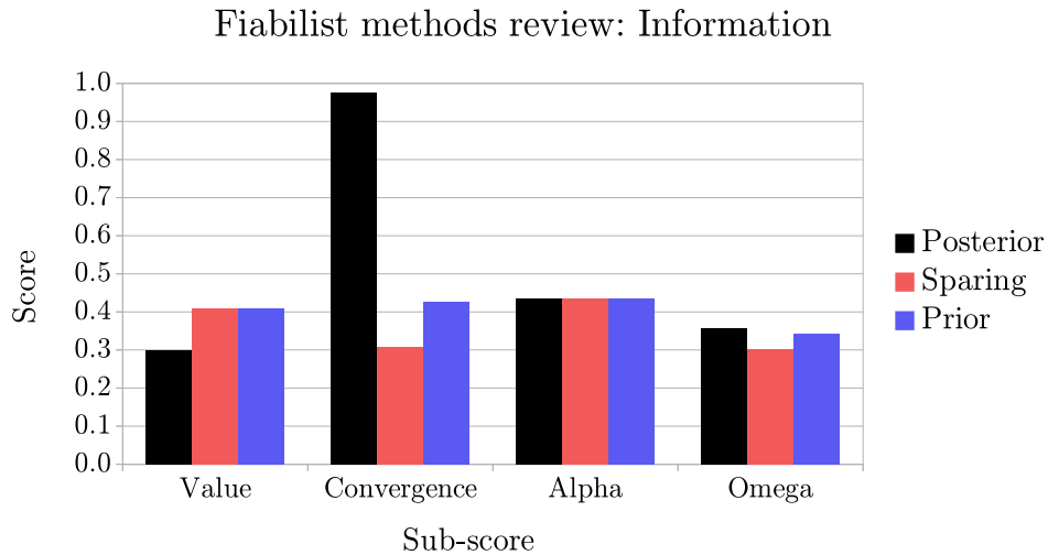
Figure 6.5: Fiabilist methods review: Average information sub-scores
