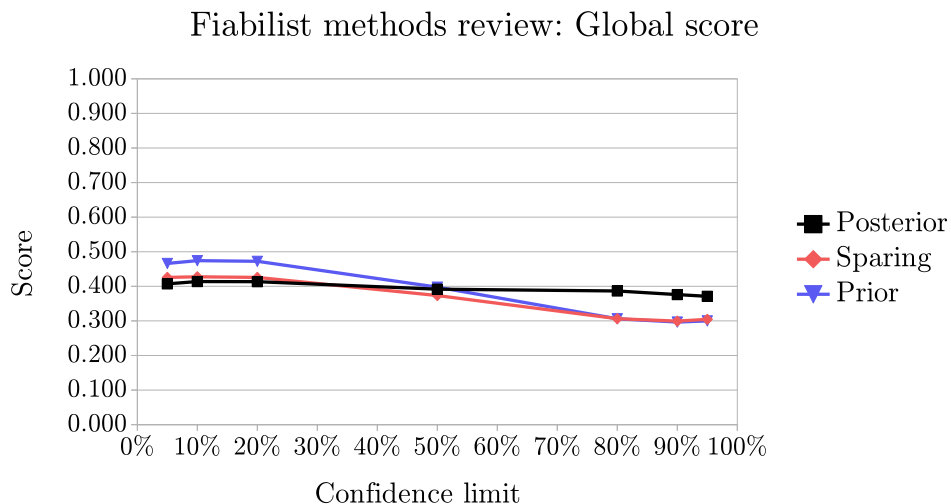
Figure 6.9: Fiabilist methods review: Global score with respect of the confidence limit
