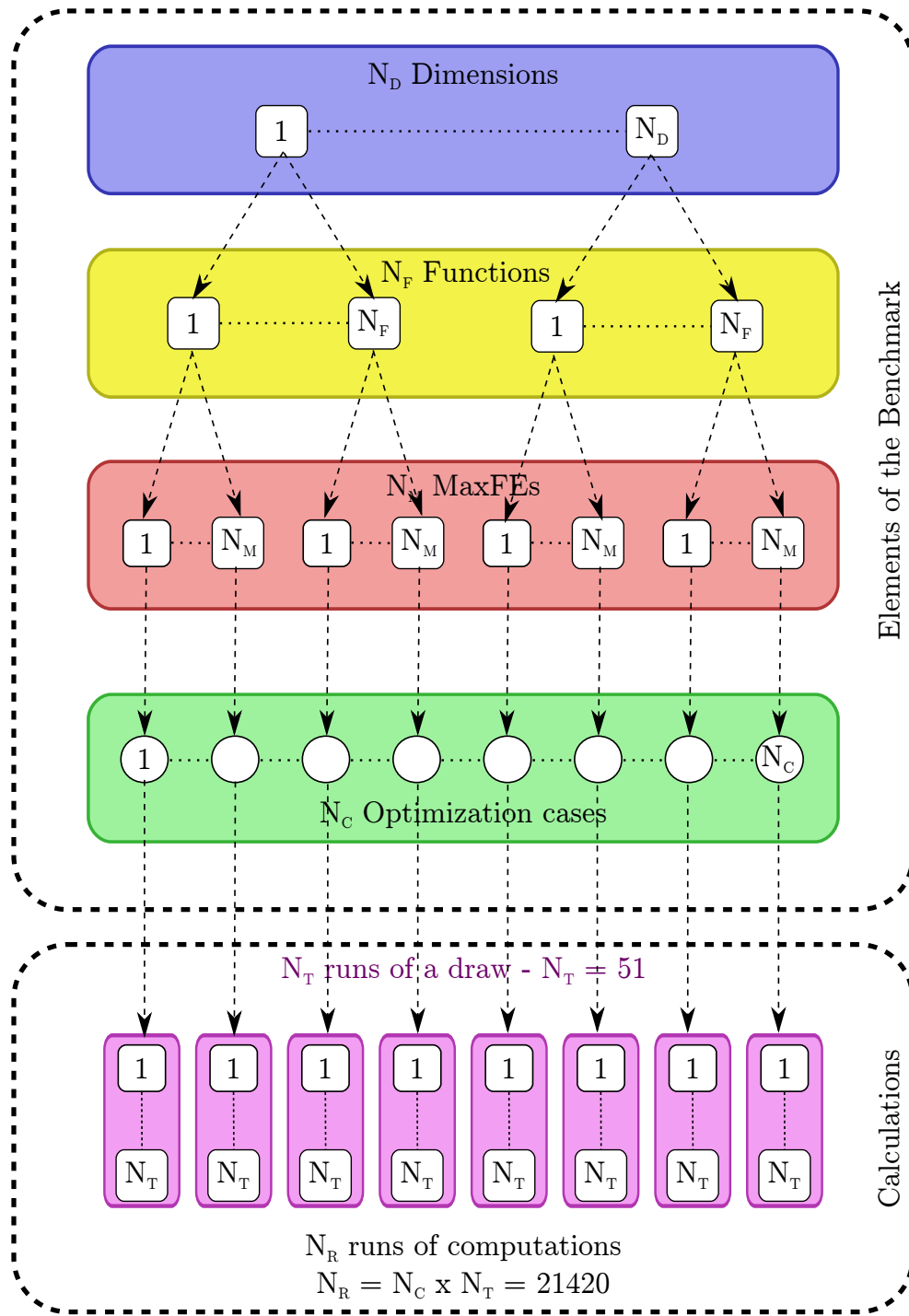
Figure 4.1: Global architecture of the benchmark - optimization cases and runs generation
