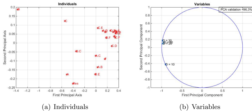
Figure 5.3: PCA in case 1 - DoEs with fixed dimensions
