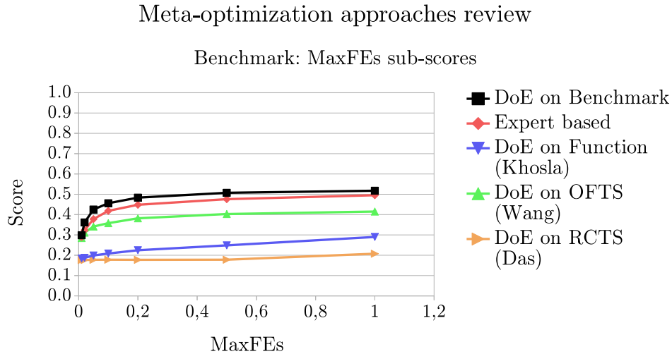
Figure 5.10: Settings review: MaxFEs sub-scores
