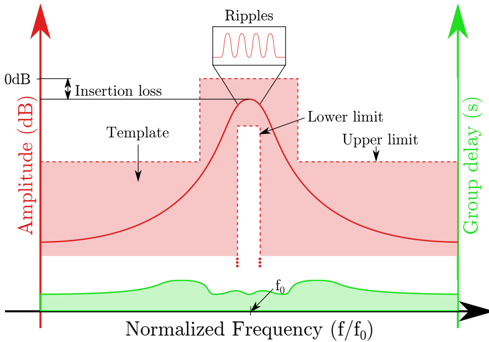
Figure 7.1: Filter specifications on the transfer function
