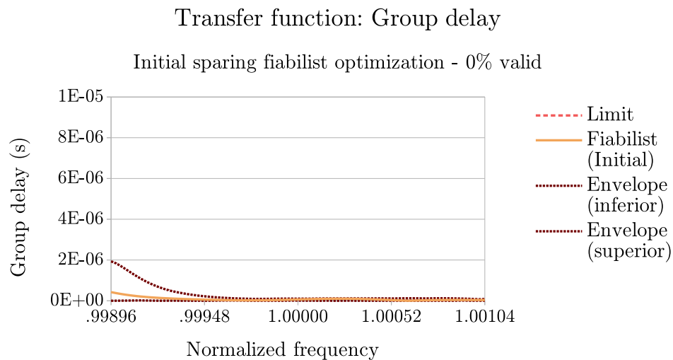
(b) Sparing initial optimization - Group delay transfer function
