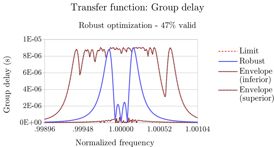
(b) Group delay transfer function
