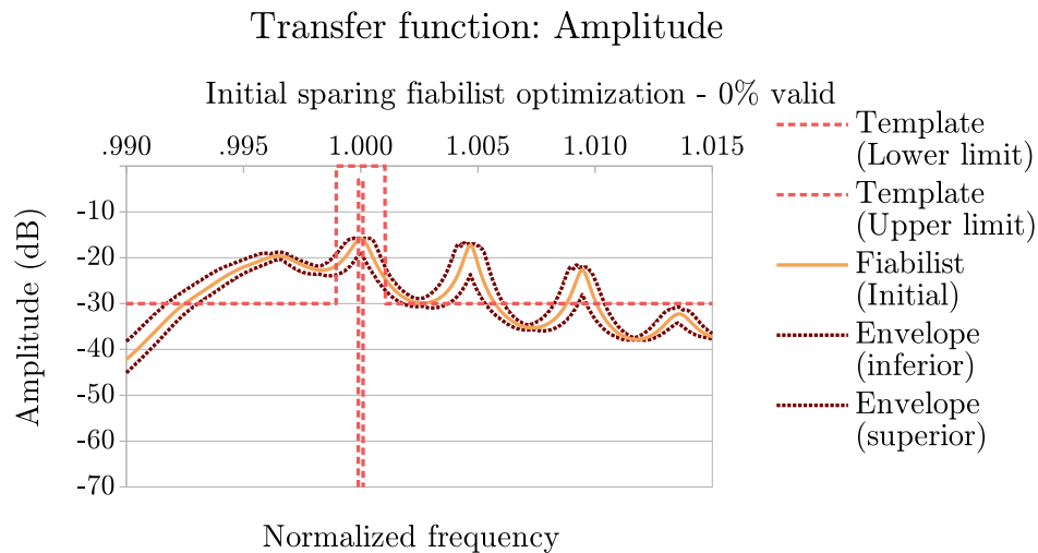
(a) Sparing initial optimization - Amplitude transfer function
