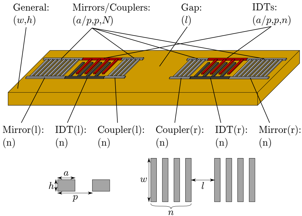
Figure 7.5: DMS design parameters
