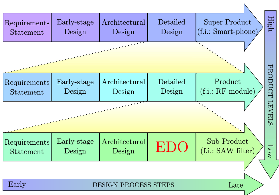
Figure 1.1: EDO process positioning into the design process - Inspired by [21]
