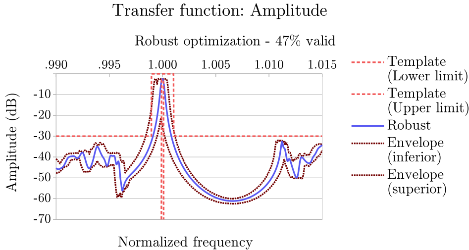
(a) Amplitude transfer function
