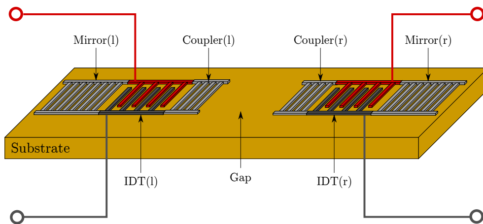
Figure 7.3: DMS filter architecture
