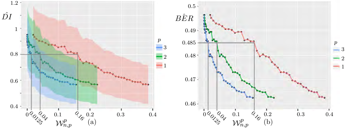
Figure 5.3 – Evolution of (a) \hat{D}I and (b) \hat{B}ER with \mathcal{W}_{n,p}^p(\mathcal{L}(f(\tilde{X}_{0,\lambda}) \mid S=0), \mathcal{L}(f(\tilde{X}_{1,\lambda}) \mid S=1))
