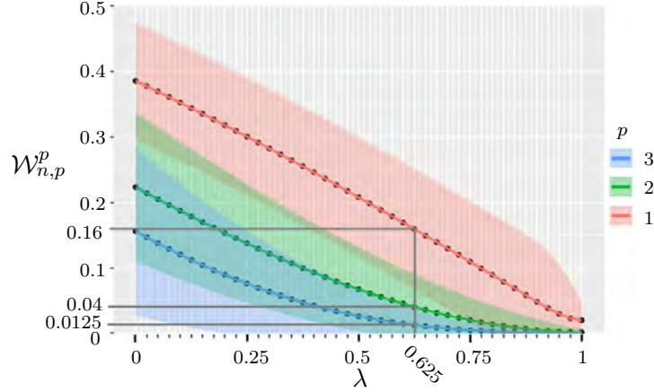
Figure 5.2 – Asymptotic confidence interval for \mathcal{W}_p^p(\mathcal{L}(f(\tilde{X}_{0,\lambda}) \mid S=0), \mathcal{L}(f(\tilde{X}_{1,\lambda}) \mid S=1))
