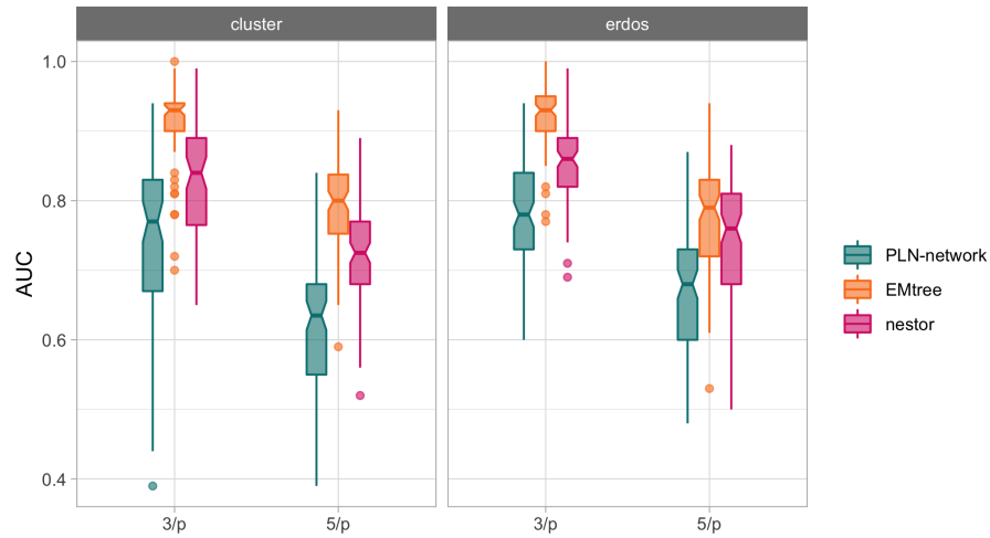
Figure 3.13 – AUC measures obtained with PLN-network, EMtree and nestor on 100 datasets of each type and density level.
