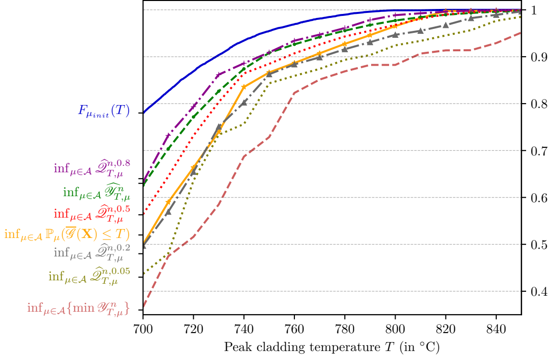
Figure 6.2: One compute a PoF sample \mathcal{Y}_{T,\mu}^n of size n = 100 . Different quantiles of this sample \widehat{\mathcal{Q}}_{T,\mu}^{n,p} [see Eq. (6.8)] are optimized over the measure space, as well as the sample mean \widehat{\mathcal{Y}}_{T,\mu}^n [see Eq. (6.6)]. In solid line, we compute the output initial distribution, and the optimization of the CDF lower envelop from the predictor of the metamodel (reduced to 6 input). Each curve takes approximately two days to compute on a regular computer, without any optimization and parallelization of the algorithm.
