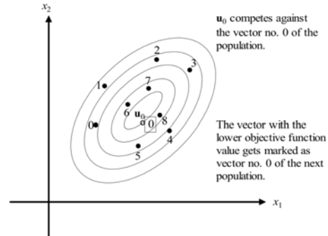
(d) Selection. Because it has a lower function value, \mathbf{u}_0 replaces the vector with index 0 in the next generation.
