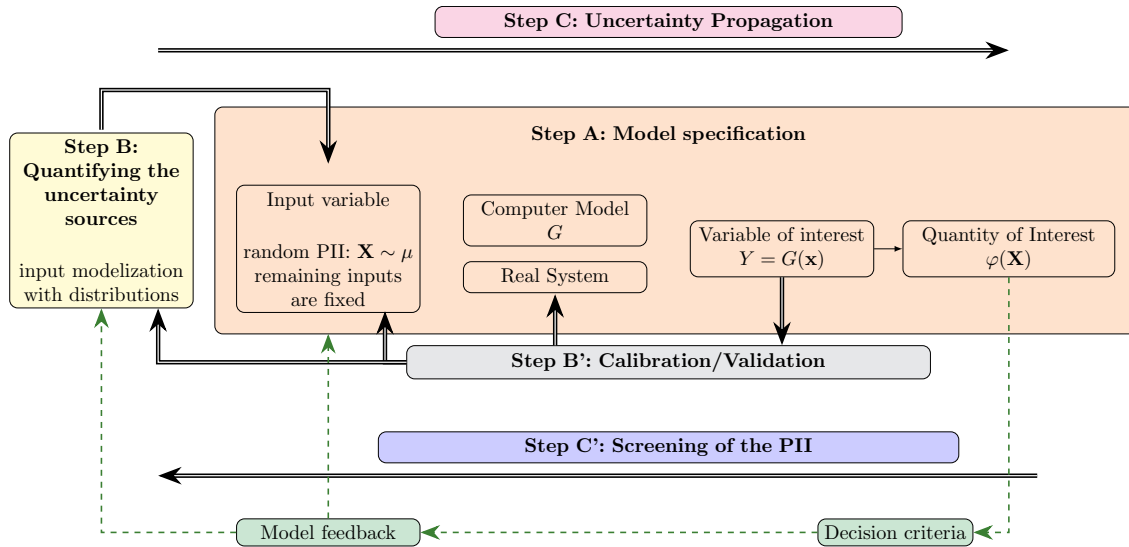
Figure 1.1: This scheme represents the usual UQ methodology employed in engineering study.
