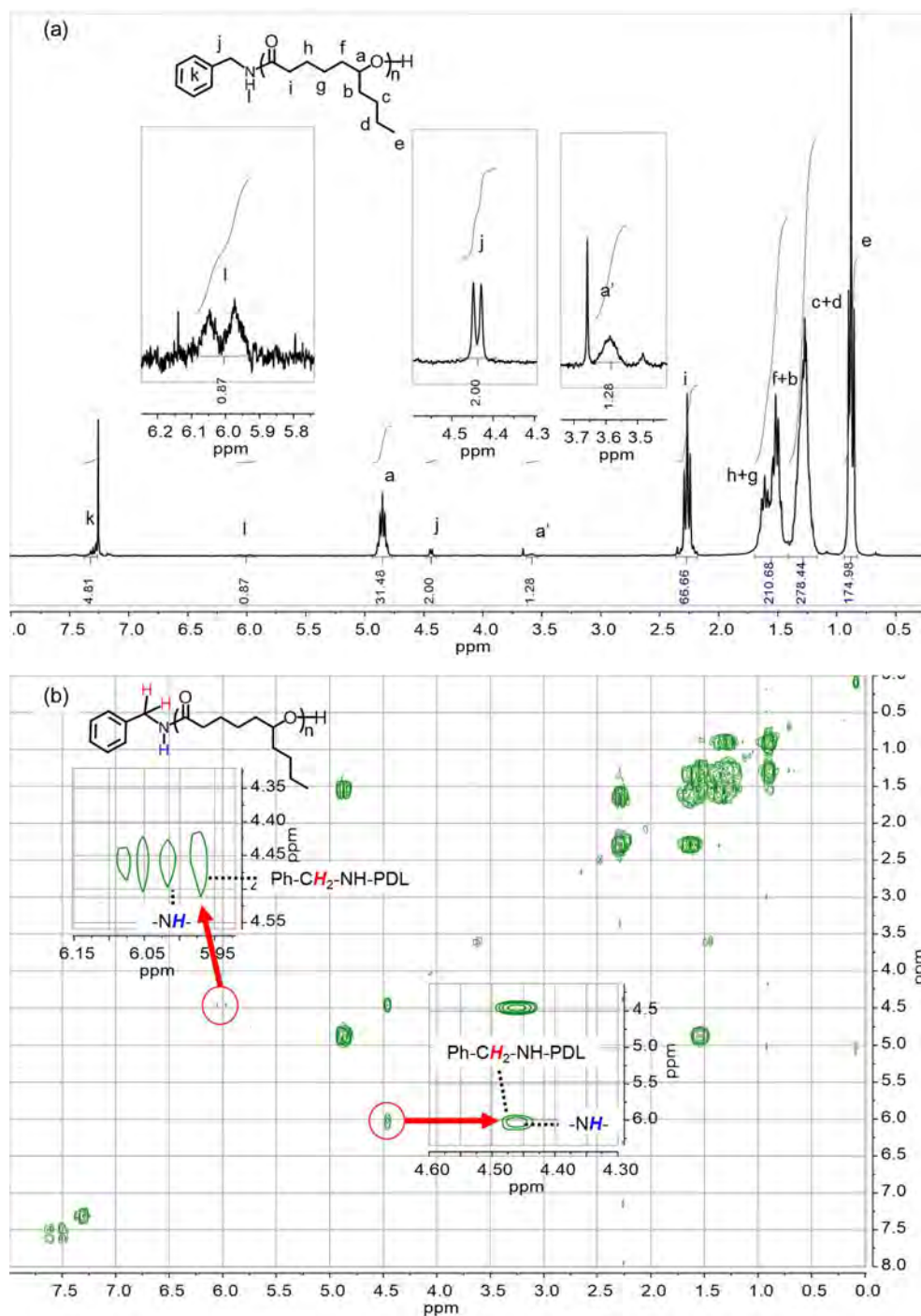
Figure 2.6. a) 1 H NMR spectrum (CDCl 3 , 300 MHz) and b) Extract of the 2D COSY, of a PDL of DP 30 initiated by BnNH 2 , [ε-DL] 0 /[BnNH 2 ] 0 /[InCl 3 ] 0 /[NEt 3 ] 0 = 30/1/1/2 in toluene at 60 °C, [ε-DL] 0 = 3 mol/L.
