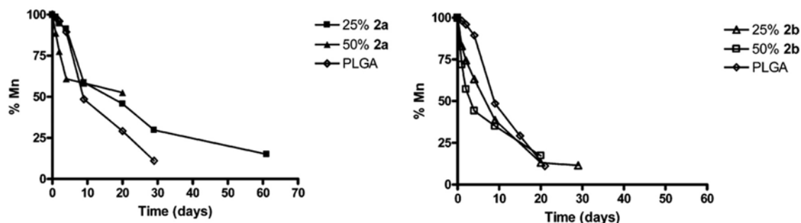
Figure 3.11 Relative decrease in M_n as a function of time for PLGA and copolymers with either 25% or 50% of hydroxyl groups. 13
