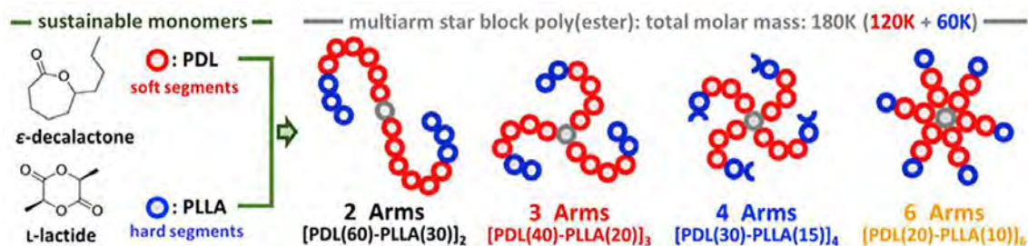
Figure 3.4 Semi-crystalline PLLA/PDL-based block copolymers with different multiarm shapes. 8
