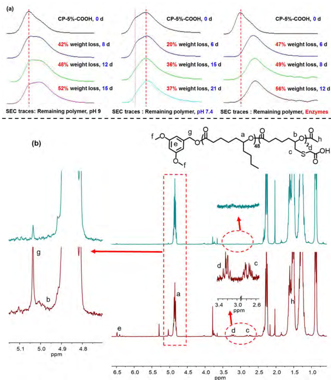
Figure 4.19 (a) SEC traces of remaining copolymers from the degradation of CP-5%-COOH in three different conditions. (b) Stacked 1 H NMR spectra of remaining polymer after enzymatic degradation and CP-5%-COOH.
