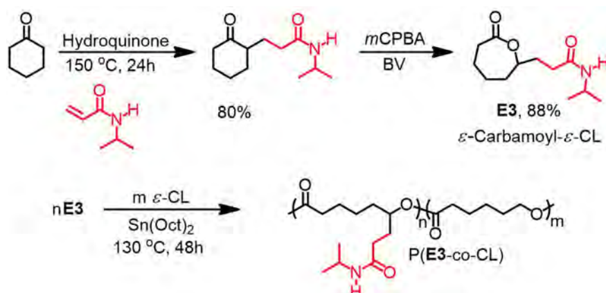
Scheme 1.24 Synthetic route of \epsilon -carbamoyl- \epsilon -CL ( E3 ) and its copolymerization with \epsilon -CL. 43b
