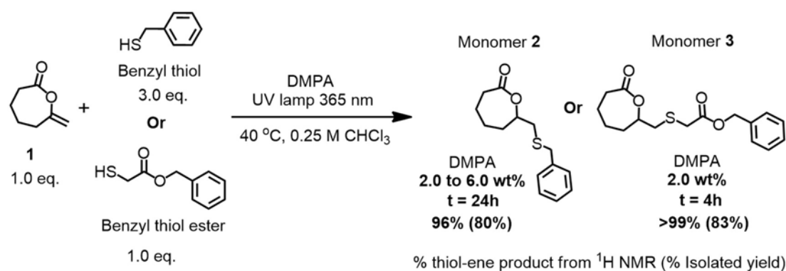
Scheme 1.55 The summary protocol for the synthesis of new functional monomers via thiol-ene functionalization
