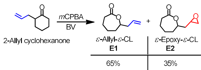
Scheme 1.23 The single synthetic step of \epsilon -allyl- \epsilon -CL ( E1 ) with the side product \epsilon -epoxy- \epsilon -CL ( E2 ). 43a
