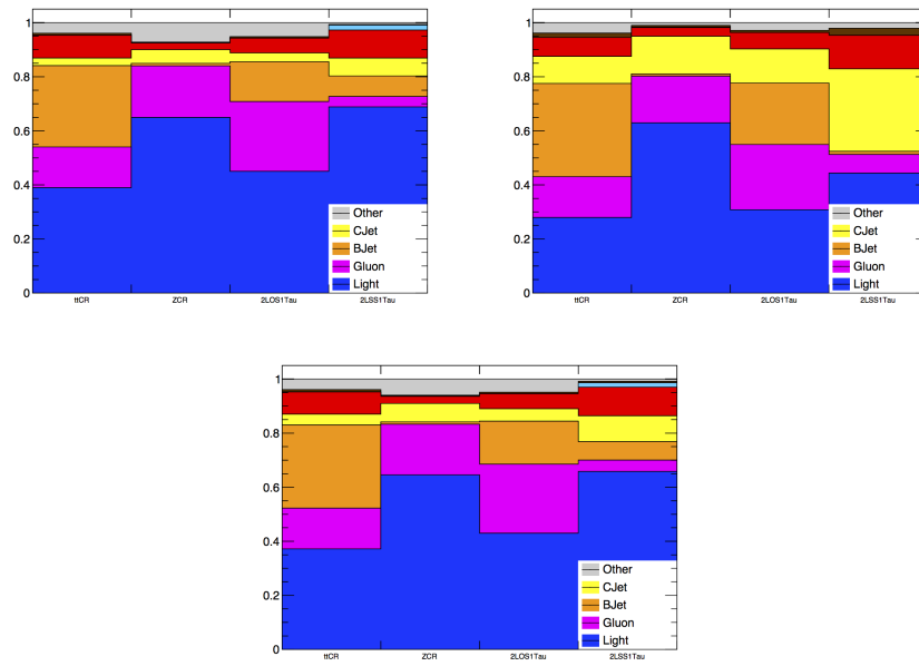
FIGURE 5.12: Composition plots of fake \tau origin for 1-prong (left), 3-prong (middle) and all-prong (right).
