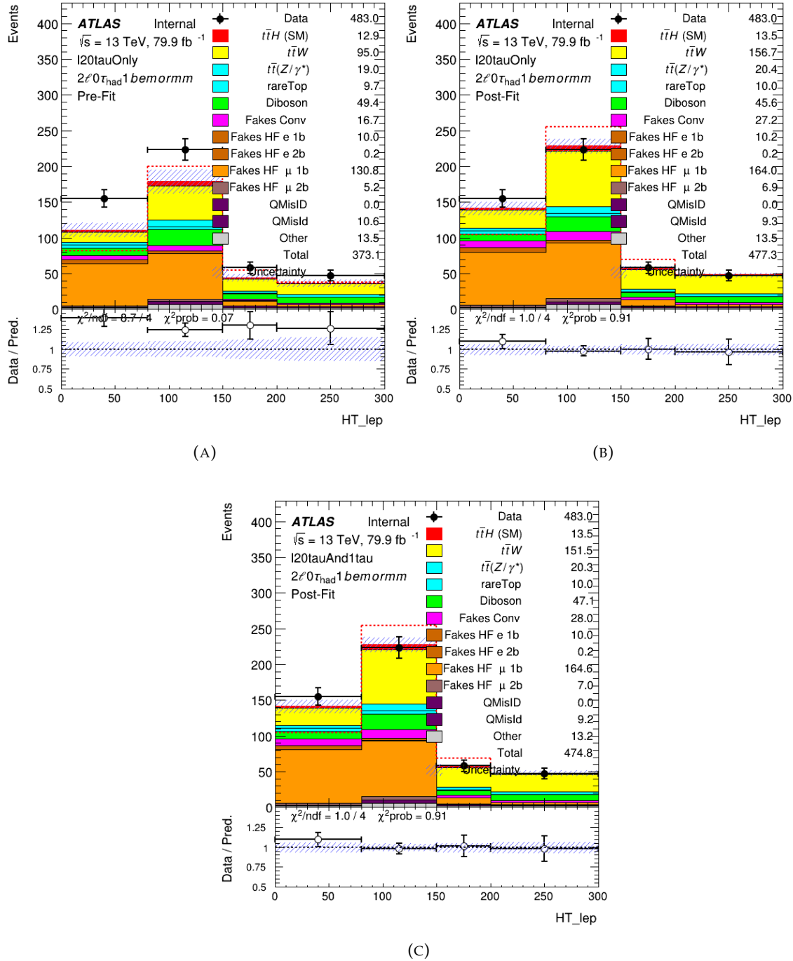
FIGURE 5.19: Prefit plot of CR1 in 2\ell\text{SS}+1\tau_{\text{had}} channel used in the template fit validation (A), Postfit plots after 2\ell\text{SS} regions only fit (scenario 1) (B) and after 2\ell\text{SS} plus 2\ell\text{SS}+1\tau_{\text{had}} regions fit (scenario 2) (C).
