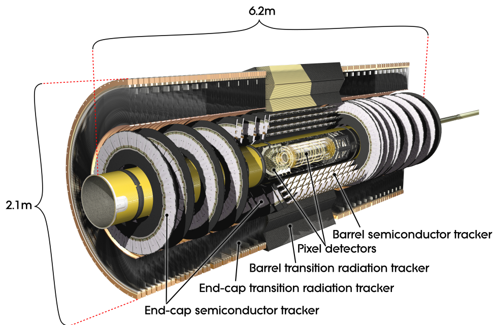
FIGURE 3.6: An overview of the ATLAS inner detector.
