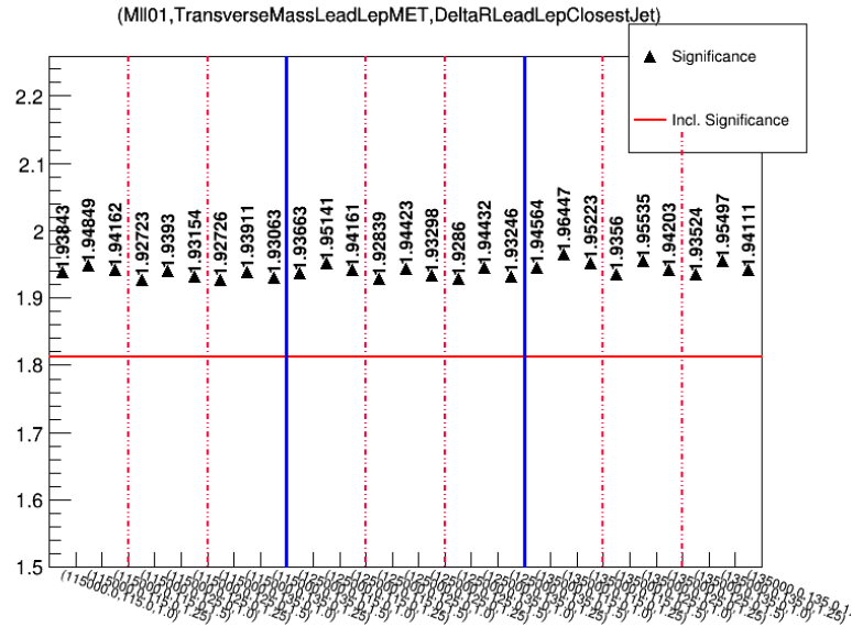
FIGURE 5.7: Results of the 3-D scanning of the variables which are chosen to build the final categorisation. The blue line splits the whole range according to the value of Mll01(left to right, 115 GeV, 125 GeV and 135 GeV). Then The red dash line split each smaller range according to the value of TransverseMassLeadLepMET (left to right, 115 GeV, 125 GeV and 135 GeV). Finally the three bins in each region defined by red dash lines represent the value of DeltaRLeadLepClosestJet (from left to right, 1, 1.25, 1.5).
