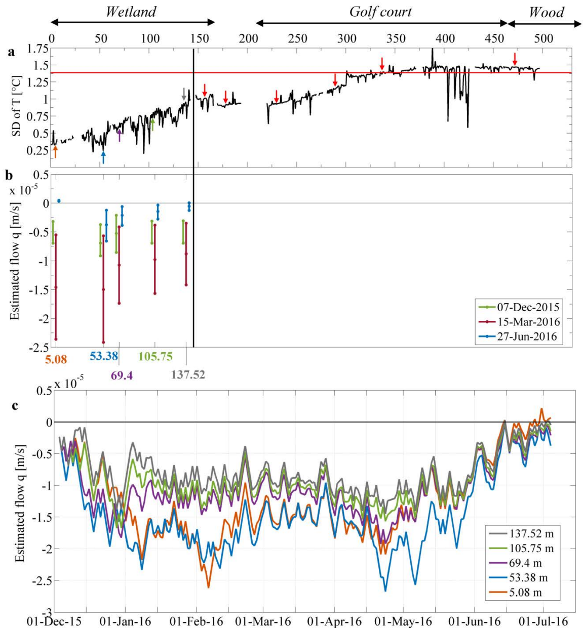
Figure 2-14. a. Application of the model on DTS measurements: selection of the spots according to the value of SD measured along the FO cable. The non-buried sections were removed from the data set. The model presented consistent results only for DTS measurements located in the first 150 meter of the stream providing b. Range of flow estimated at three different dates and c. Temporal evolution of the estimated flow considering \lambda=2.5\text{W/m/K} .
