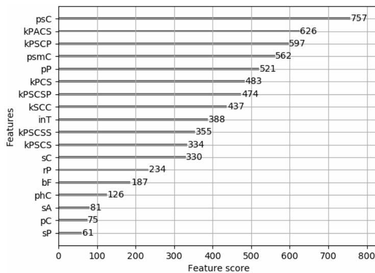
Figure 4.12: Local detection: XGBoost feature importance
