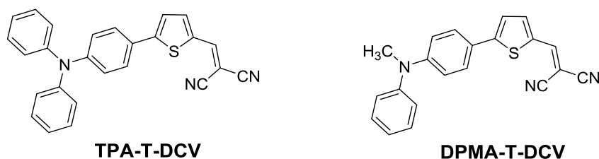
Figure 1.31 Structure of TPA-T-DCV and DPMA-T-DCV , DPMA stands for DiPhenylMethylAmine.
