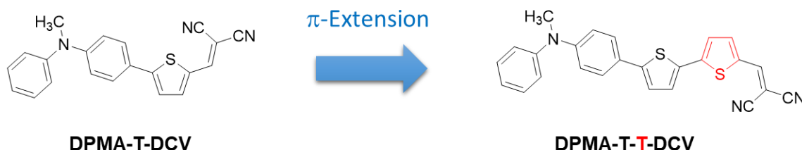
Chart 3.1. \pi -Extended DPMA-T-T-DCV as push-pull molecular donor for OPV.
