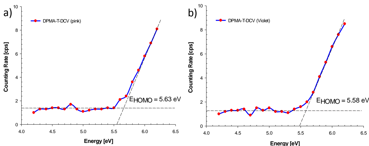
Figure 2.5. PYSA spectra of films of DPMA-T-DCV on ITO a) as cast (pink film, left) and b) after reorganization with time (violet film, right) .
