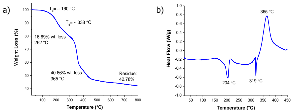
Figure 5.3. a) TGA and b) DSC curves of T-2 measured under \text{N}_2 using a heating rate of 10^\circ\text{C}/\text{min} .
