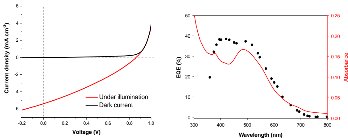
Figure 5.7. a) Best current density-voltage characteristic of the BHJ OSC in the dark and under AM 1.5 solar simulation ( 100 \text{ mW cm}^{-2} ). b) EQE spectrum of the BHJ OSC and UV-vis spectrum of the blend T-2 :PC 71 BM (1:3 w/w) on glass.
