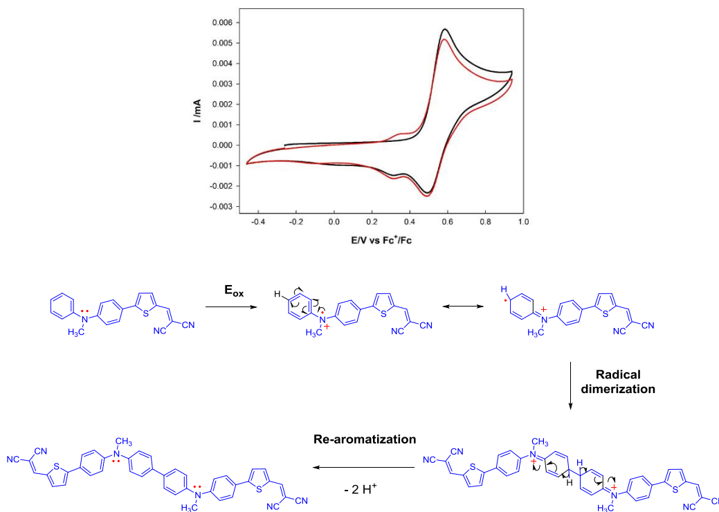
Figure 5.6. CVs of DPMA-T-DCV, 0.5 mM in 0.10 M Bu 4 NPF 6 /CH 2 Cl 2 , scan rate 100 mV s -1 , Pt working electrodes (1 st and 2 nd traces in black and red, respectively). Mechanism of formation of the benzidine product.
