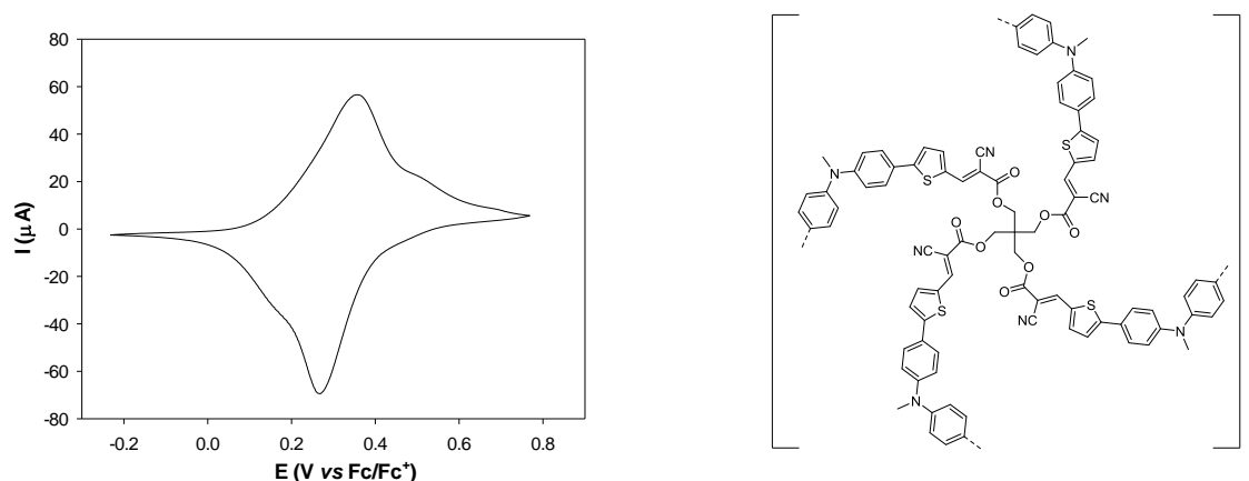
Figure 5.5. Left: CV response of poly( T-2 ) in 0.1 M n -Bu 4 NPF 6 /CH 3 CN, scan rate 100 mV/s, grown in potentiostatic conditions using 0.5 mM of T-2 in 0.1 M n -Bu 4 NPF 6 /CH 2 Cl 2 ( E = 0.52 V, 50 mC/cm 2 ). Right: structure of the expected electrogenerated polymer.
