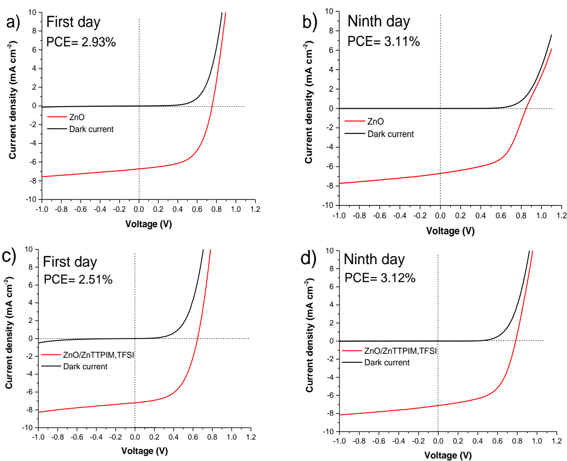
Figure 2.20. J-V characteristics of ITO/ETL/ C_{70} /DPMA-T-DCV (15 nm)/ \text{MoO}_3 /Ag devices using as ETL: a) ZnO (1 st day), b) ZnO (9 th day), c) ZnO/TTPIM, TFSI (1 st day) and d) ZnO/TTPIM, TFSI (9 th day).
