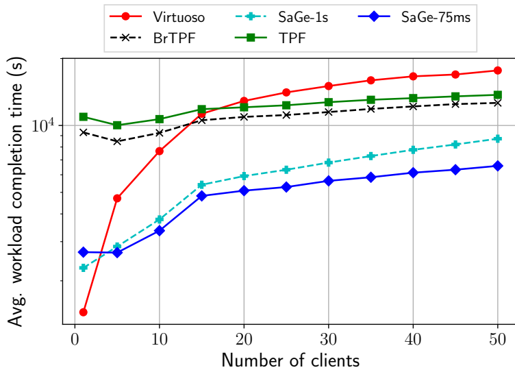
Figure 4.7: Average workload completion time per client, with up to 50 concurrent clients (logarithmic scale).
