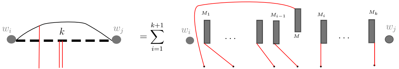
Figure 3.6 – Homological relation.
