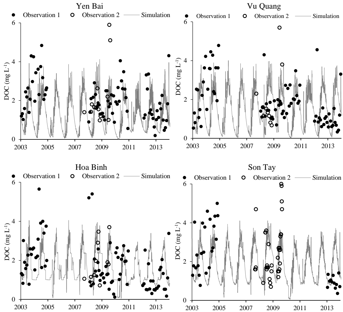
Figure 5-4 Daily variations of dissolved organic carbon (DOC) concentration (mg L -1 ) at four stations from 2003 to 2013. Observation 1 (black dot) shows the DOC measured by Le et al. (2017a); observation 2 (white dot) shows the DOC measured by Dang (2006); calculations from Equation 1 based on the simulated discharge ( Q , m 3 s -1 ) from Wei et al. (2019) with the values of the parameters given in Table 2 are the gray solid line.
