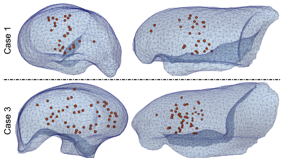
Figure 3.4: Spatial distribution of anatomical landmarks within the lung in the pre-operative configuration.
