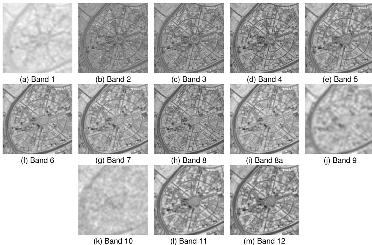
Figure A.1: Example of Sentinel-2 image bands. Differences in spatial resolutions can be perceived as a variance in sharpness in the images above.
