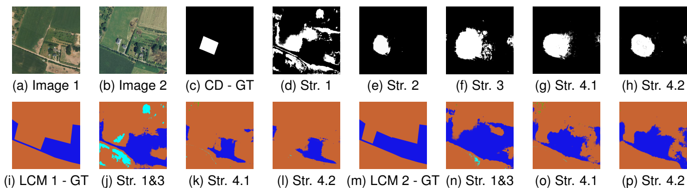
Figure 4.11: Illustrative images of the obtained results: (a)-(b) multitemporal image pair; (c) ground truth change detection map; (d)-(h) predicted change maps; (i)-(l) ground truth and predicted land cover maps for image 1; (m)-(p) ground truth and predicted land cover maps for image 2.
