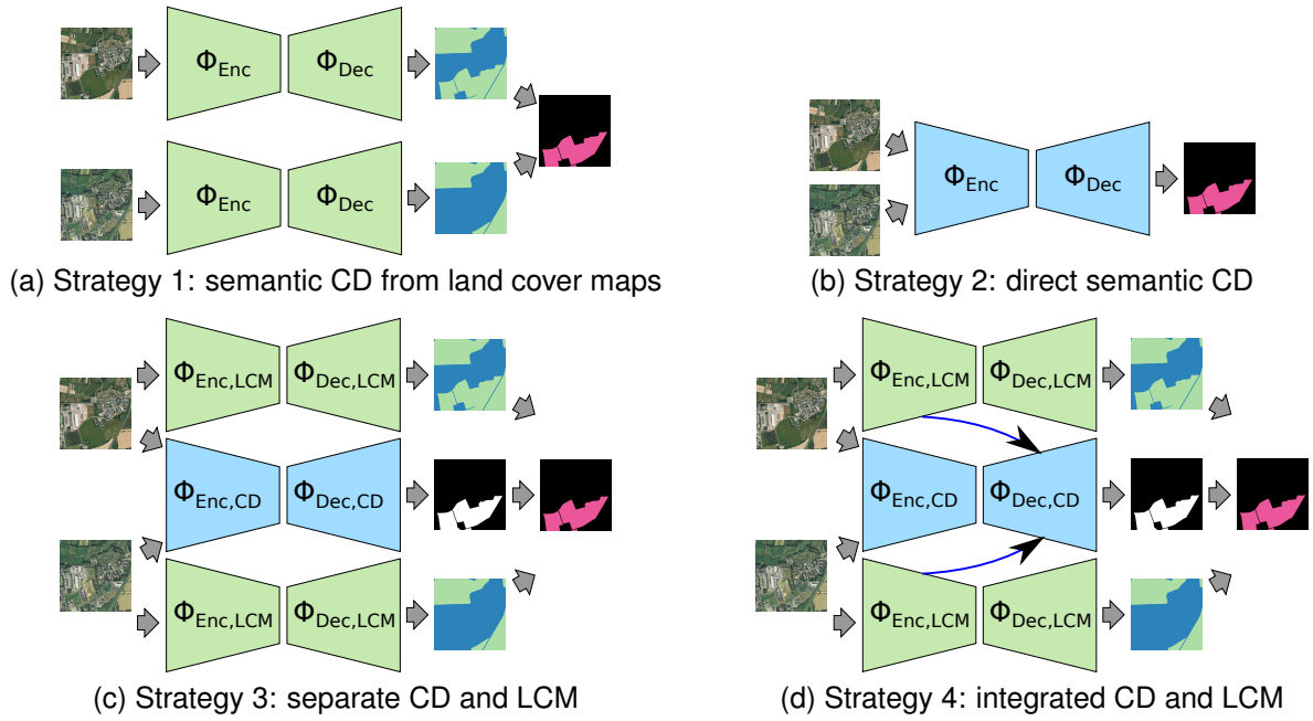
Figure 4.4: Schematics for all four proposed strategies for semantic change detection. \Phi represents the network branch’s learnable parameters, “Enc” means encoder, “Dec” means decoder, “LCM” means land cover mapping, and “CD” means change detection.
