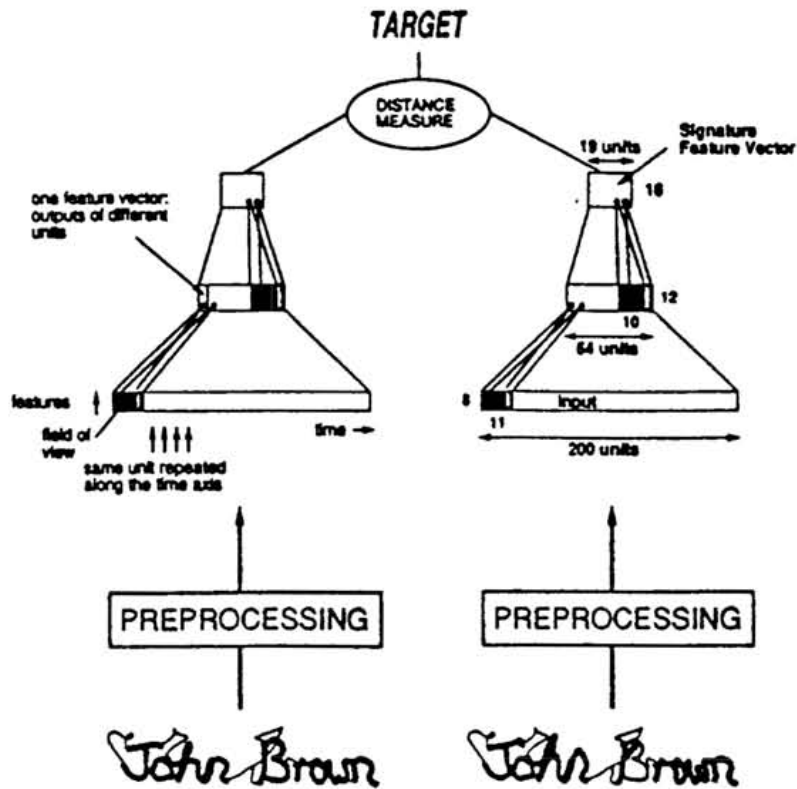
Figure 2.6: The CNN proposed by Bromley et al. was the first one to have a Siamese structure. It was used to compare signatures automatically. Image reproduced from [BGL + 94].
