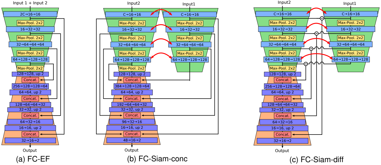
Figure 3.6: Schematics for the three FCN architectures for change detection. These architectures are U-Net inspired extensions of the patch based networks presented previously. In (b) all the activations from both streams are used for skip connections, while in (c) the magnitude of their difference is explicitly calculated. Red arrows represent shared weights between Siamese branches.
