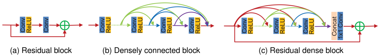
Figure 2.10: Schematics of (a) residual block, (b) dense block, and (c) residual dense block as described in [ZTK + 18].
