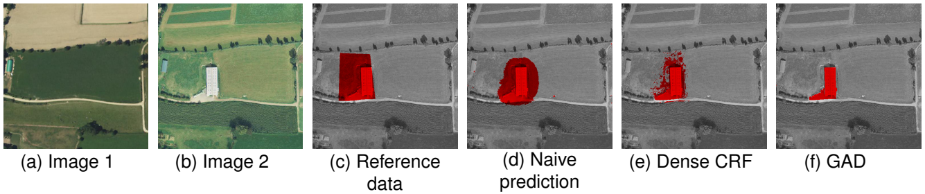
Figure 5.8: Comparison between (c) original dataset ground truth, (e) prediction filtered by Dense CRF, and (f) prediction filtered with guided anisotropic diffusion for 20000 iterations.
