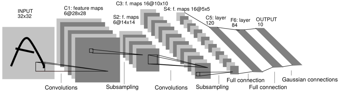
Figure 2.5: LeNet-5 was the first convolutional neural network to combine bioinspired weight sharing operations with gradient-based learning. Image reproduced from [LBBH98].
