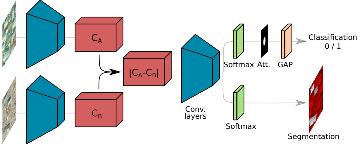
Figure 5.6: Basic schematic of the network used for weakly supervised change detection. Two paths can be taken: the classification path uses the proposed attention layer and global average pooling to produce a classification of the image, while the segmentation path avoids these steps to output pixel-level predictions. Supervision is only available on the classification path.
