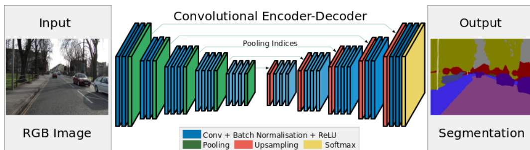
Figure 2.8: SegNet architecture for semantic segmentation, in which the pooling indices were used for the unpooling operations to recover spatial information at each upsampling step. Reproduced from [BKC17].
