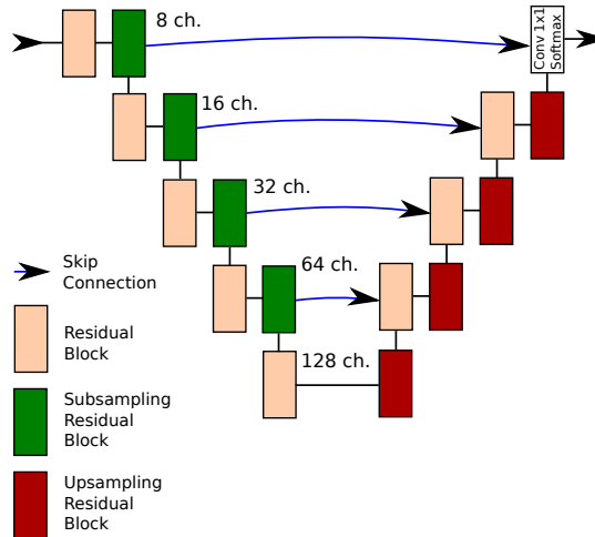
Figure 4.3: FC-EF-Res architecture, used for tests with smaller datasets to avoid overfitting. Using residual blocks improves network performance and facilitates training.
