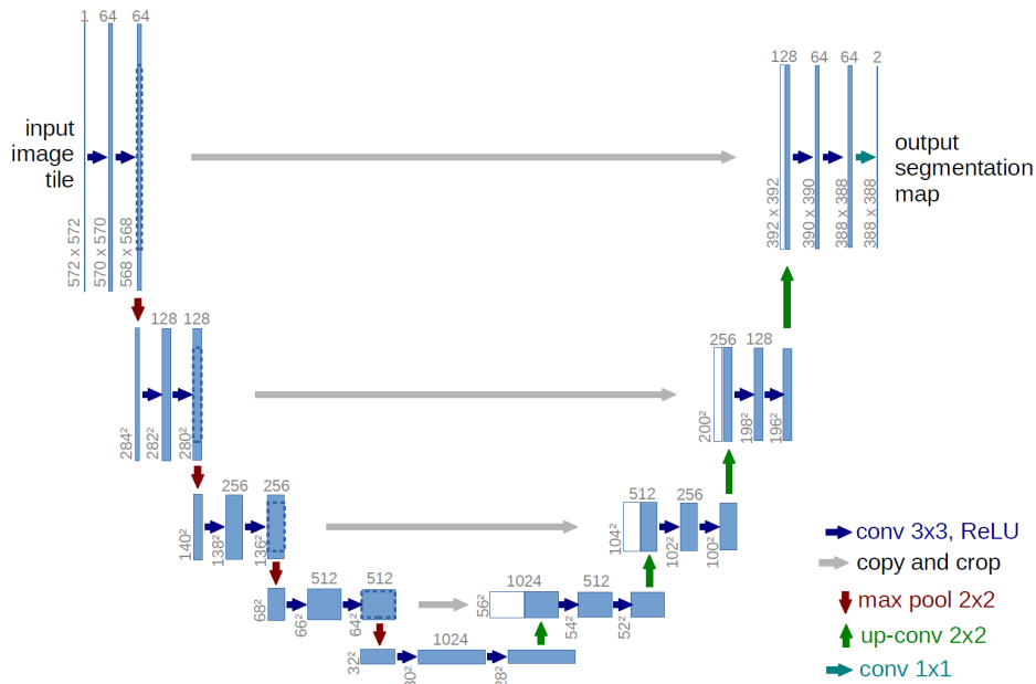
Figure 2.9: U-Net architecture schematic. The output of transposed convolutions are concatenated with feature maps produced by the encoder at several levels to combine high spatial accuracy with high-level features. Reproduced from [RFB15].
