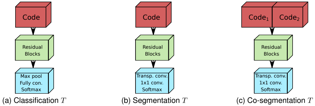
Figure 6.4: Basic schematic for the architectures of T network for each of the considered tasks.
