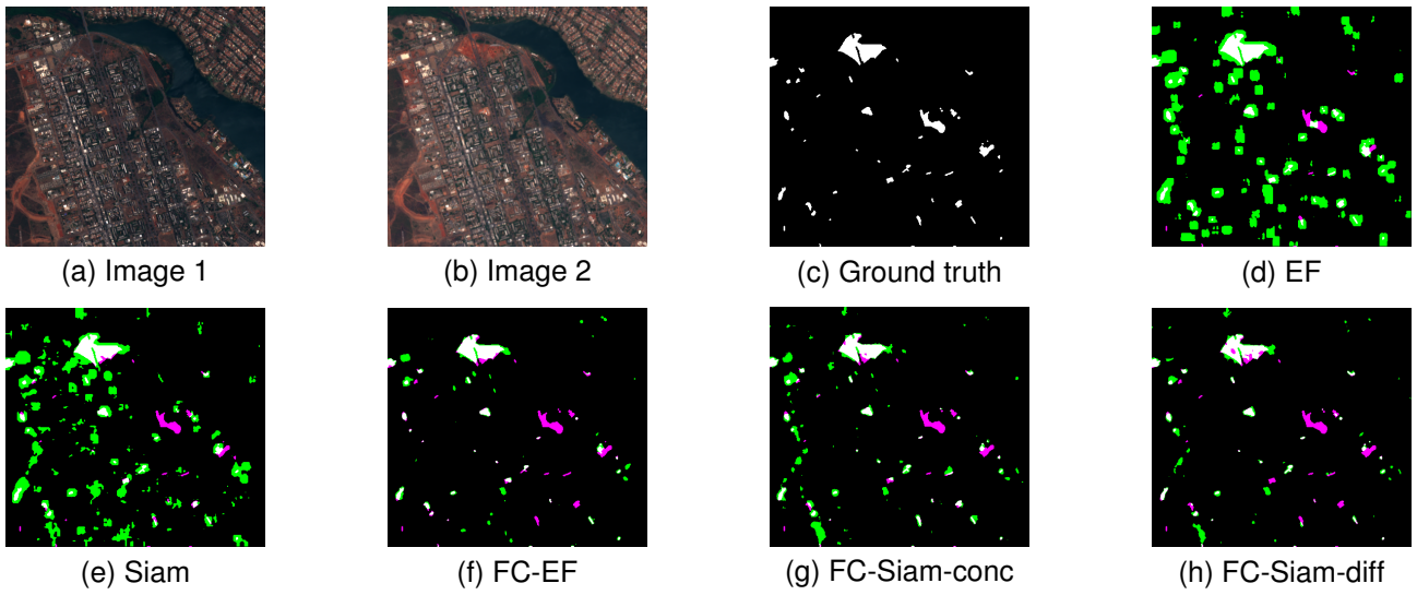
Figure 3.8: Results on the OSCD brasilia image pair using all 13 available spectral channels. White represents true positives, black represents true negatives, green represents false positives, and magenta represents false negatives.
