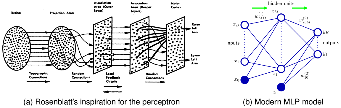
Figure 2.4: (a) While Rosenblatt's inspiration came partially from retinal nerves, the perceptron model is not restricted to vision. (b) Information flows in a single direction from inputs to outputs and through hidden units in a multilayer perceptron. Images reproduced from [Ros60] and [Mur12], respectively.
