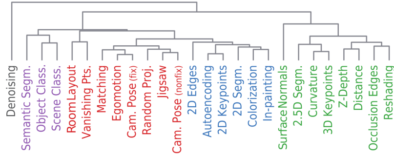
Figure 2.12: Task similarity tree proposed by the Taskonomy project. It was shown that there are several benefits from learning a single latent space representation from which several tasks are performed, such as the need for fewer annotated data. Reproduced from [ZSS + 18].
