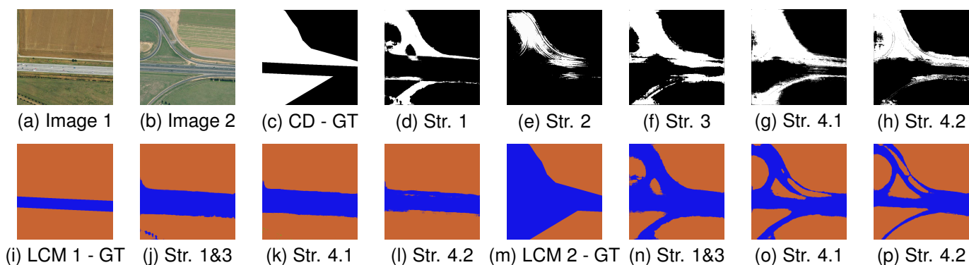
Figure 4.9: Illustrative images of the obtained results: (a)-(b) multitemporal image pair; (c) ground truth change detection map; (d)-(h) predicted change maps; (i)-(l) ground truth and predicted land cover maps for image 1; (m)-(p) ground truth and predicted land cover maps for image 2.
