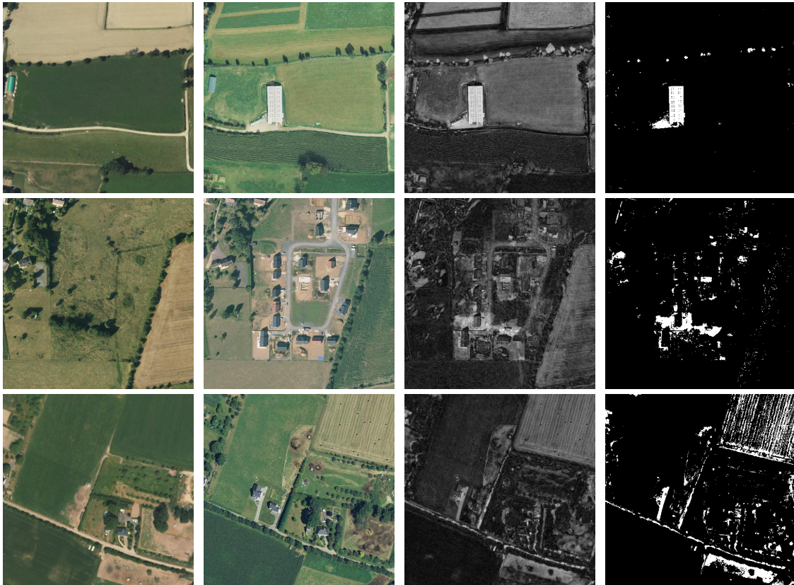
Figure 2.15: Naive change detection methods for producing and thresholding difference images tend to detect either too few or too many changes. Humans are very good at understanding difference based on the context, but the direct pixel colour difference is usually much less discriminative than our intuition suggests. Adaptive thresholding algorithms also assume there are changed and unchanged pixels in the image (often in comparable quantities), which is sometimes a flawed assumption, especially for the automated analysis of large image collections.
