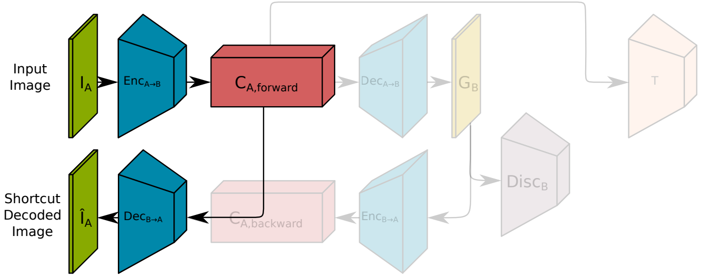
Figure 6.3: Shortcut decoding path, used for validating alignment of feature spaces during forward and backward translations.
