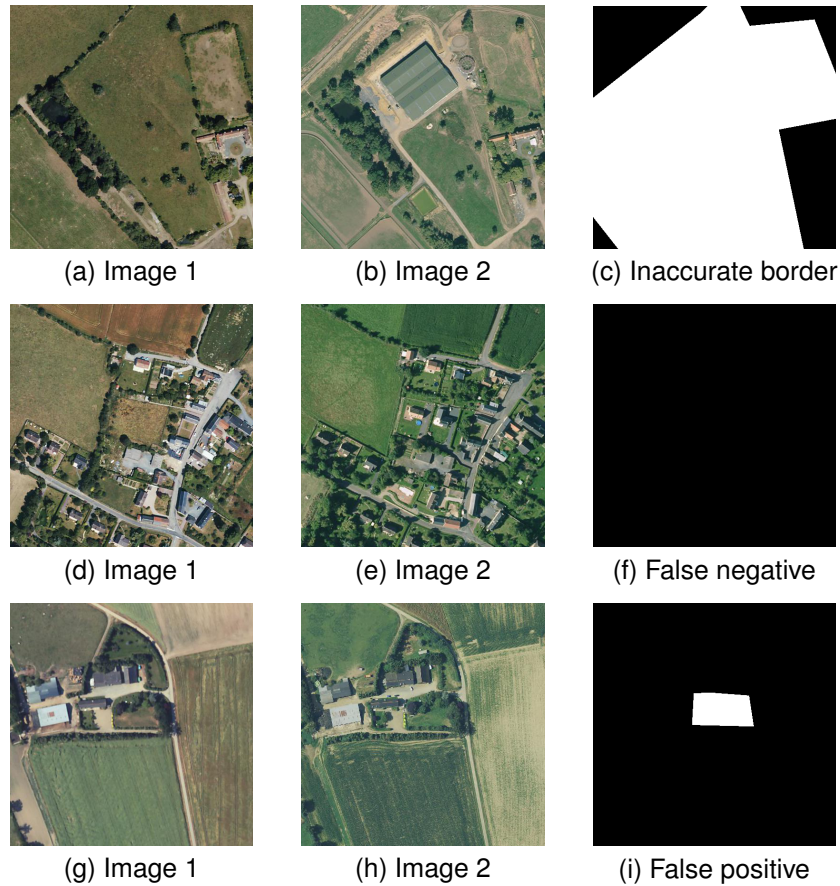
Figure 4.2: Examples of: (a)-(c) overly large change markings, (d)-(f) failure to mark changes, (g)-(i) false positive.
