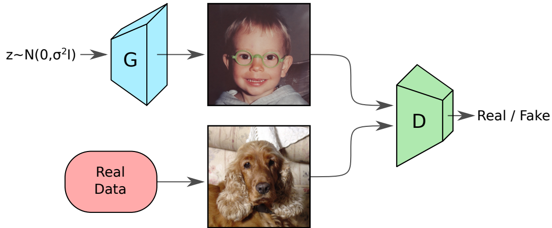
Figure 2.14: General Adversarial Networks are trained by forcing two networks to accomplish contradictory tasks. The generator G attempts to generate realistic images indistinguishable from real samples, while the discriminator D attempts to separate fake from real samples.
