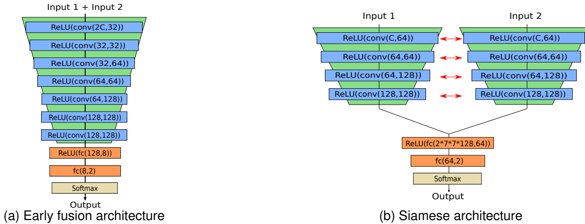
Figure 3.5: Proposed patch based CNN architectures for change detection. Processing both images since the first layer of the network allows for more total comparison operations, but does not allow for the weight sharing properties of Siamese networks.
