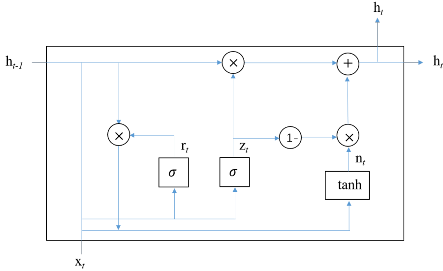
Figure 5.3: GRU cell.
