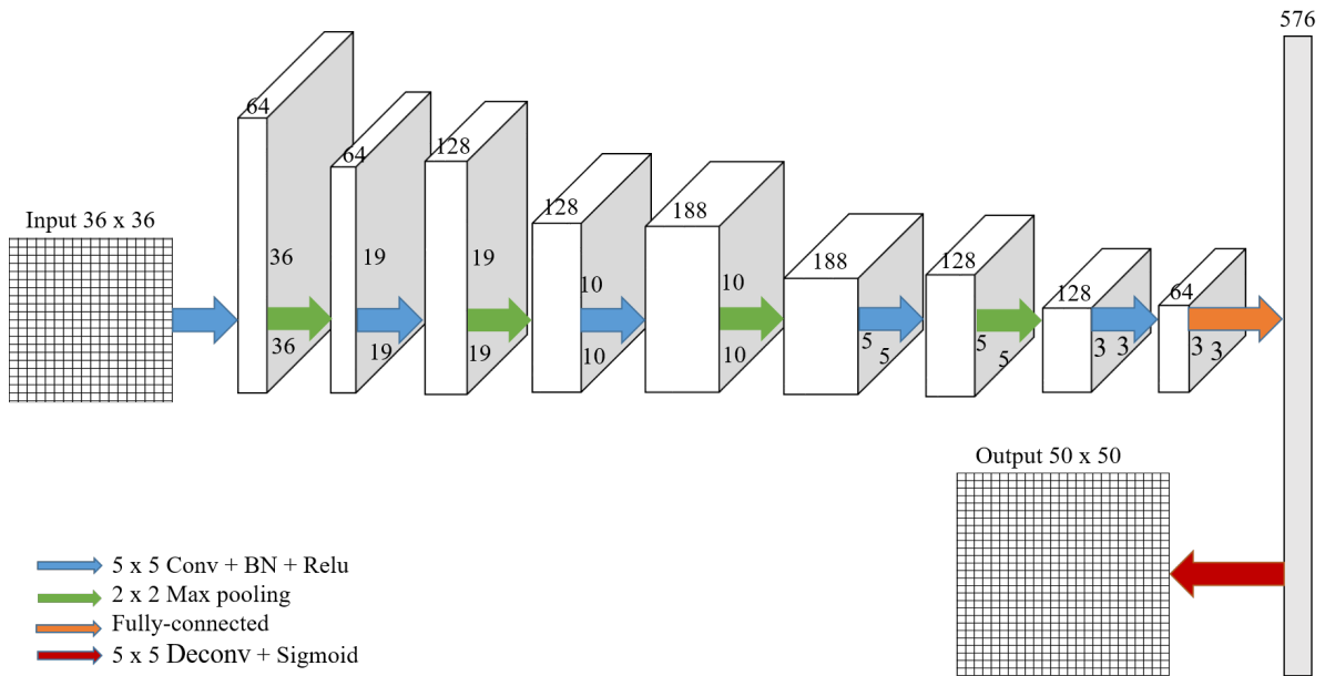
Figure 4.1: CNN architecture
