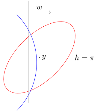
Figure 5.1 – Here \partial\Omega is in red and \partial B_r(\xi) in blue.
