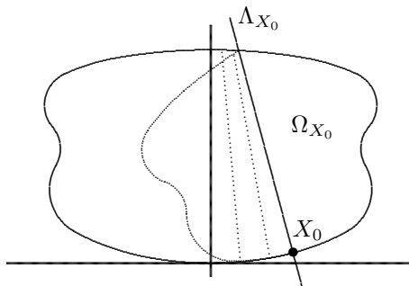
Figure 4.1 – Example of domain satisfying hypotheses (1.0.3)–(1.0.6).
