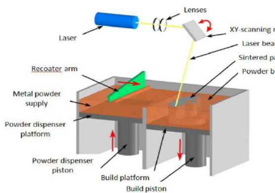
Figure 1.3: L-PBF process [35]
