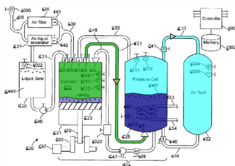
Figure 1.18: Step 4 of the compression cycle (compressed air discharge)
