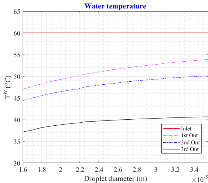
Figure 3.20: Water temperature in function of water droplet diameter
