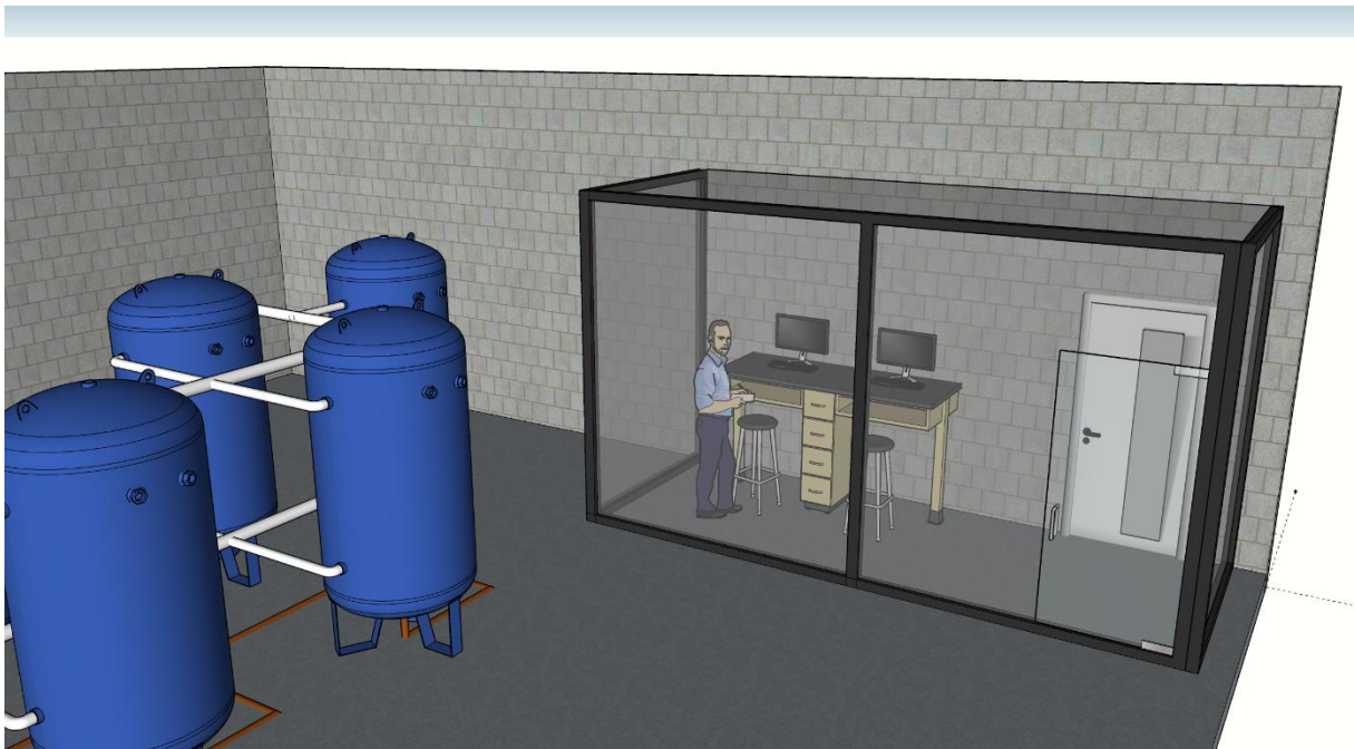
Figure 4.13: 3D model of the ideal prototype focusing the control module
