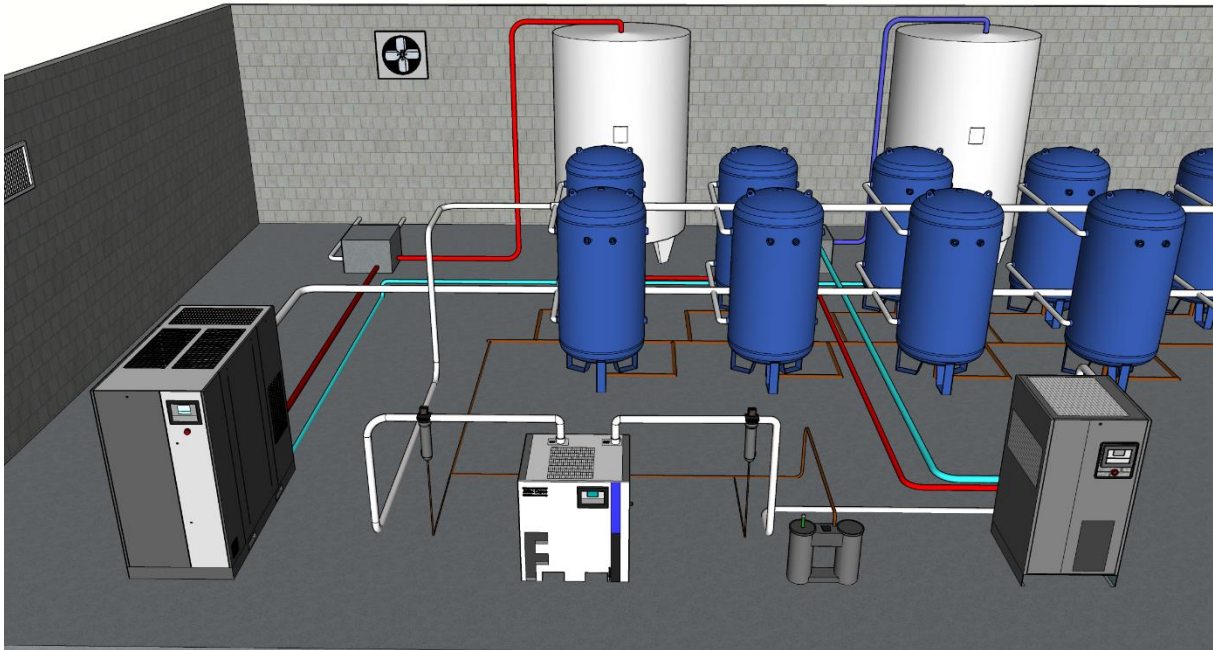
Figure 4.10: 3D model of ideal prototype with focusing on power train module (compressor, dryer, air/oil separator and expander)
