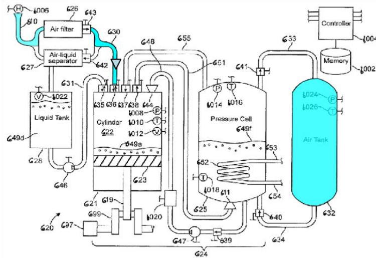
Figure 1.19: Step 5 during the compression cycle (cylinder device refill)
