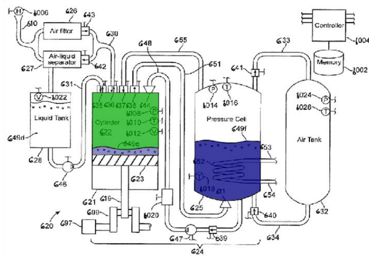
Figure 1.17: Step 3 of the compression cycle (air compression phase)
