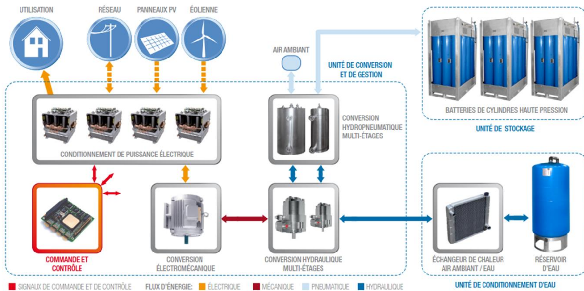
Figure 1.24: System operation of Enairys storage solution technology
