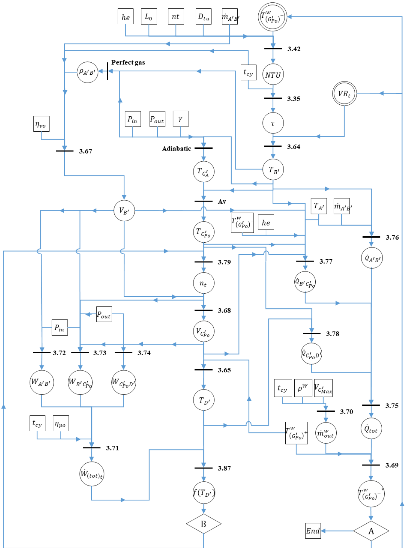
Figure 3.26: Liquid piston expander numerical code flow chart
