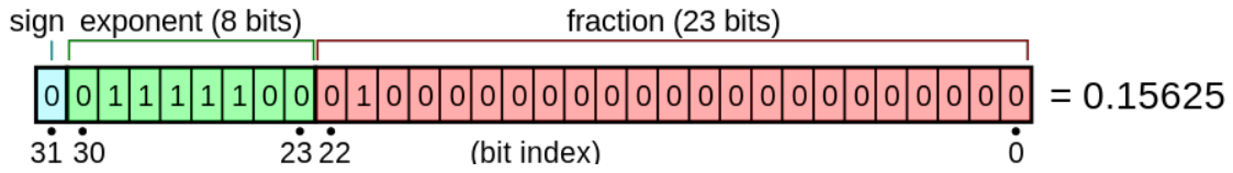
Figure 1.1: Binary representation of 0.15625 in IEEE-754 32-bit floating-point arithmetic. Picture extracted from [Stannered, 2008].
