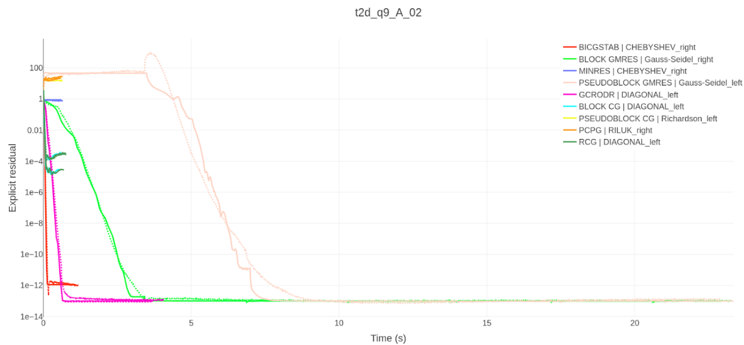
Figure 9.5: Convergence profile of a random selection of linear solvers and preconditioners for the t2d_q9_A_02 problem.
