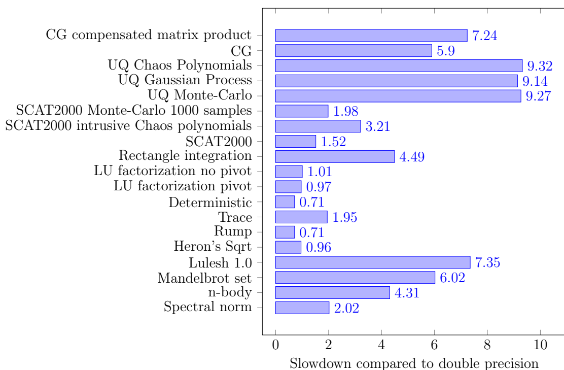
Figure 7.5: Overhead of the Shaman library compared to double precision.
