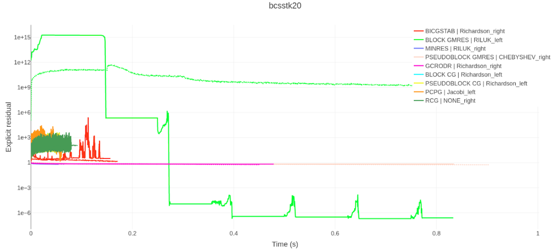
Figure 9.6: Convergence profile of a random selection of linear solvers and preconditioners for the bcstk20 problem.
